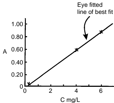
FIGURE 17.13 Standard curve for zinc.
