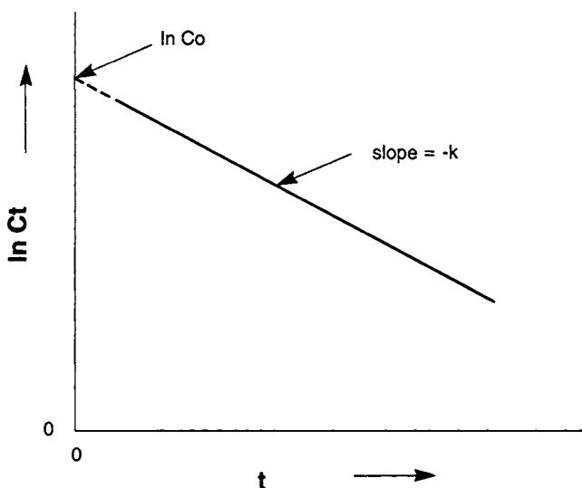
FIGURE 3.9 Theoretical plot of \ln C_t against the elapsed time.
