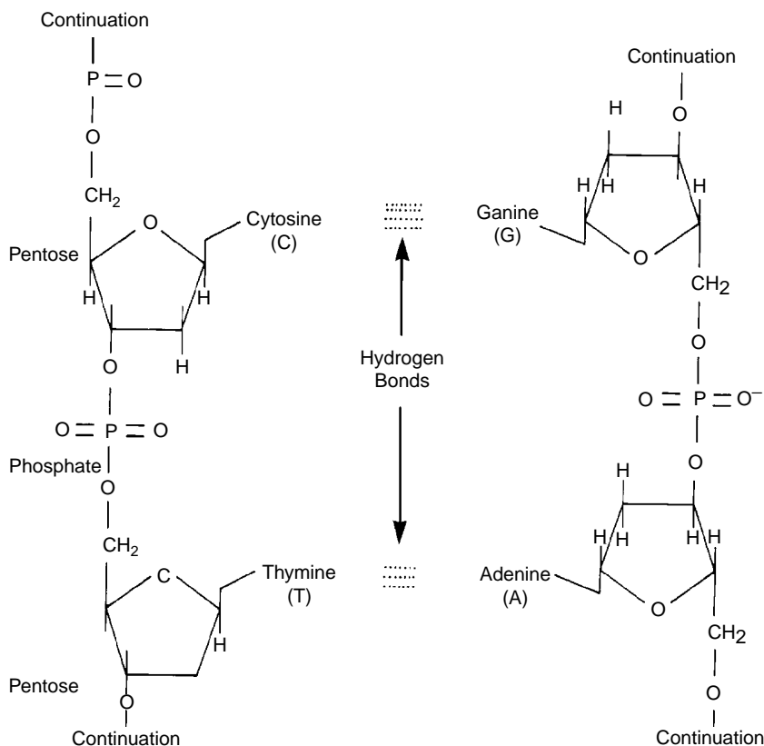
FIGURE 16.2 The chemical forms of the components of DNA and bonds between the pentose sugars and phosphate ions and between the nitrogenous base pairs.
