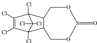
Endosulfan
