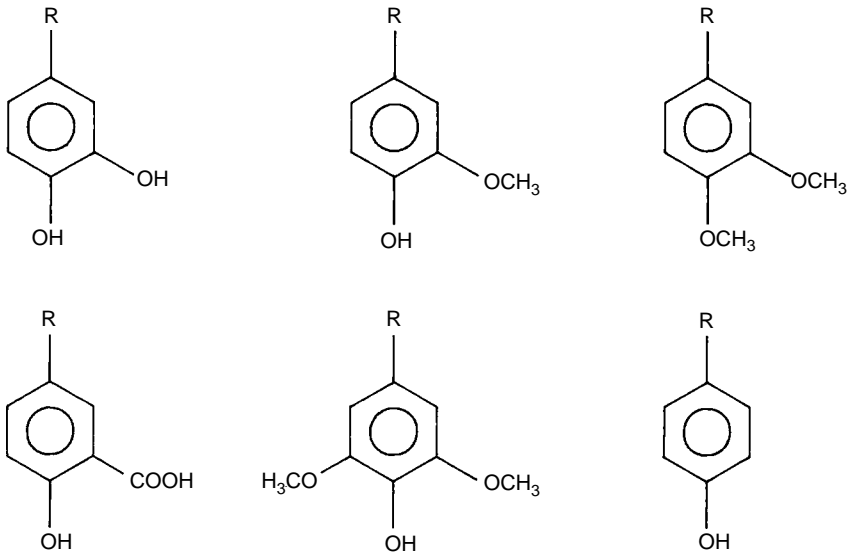
FIGURE 13.5 Phenolic groups present in the structure of humic substances.
