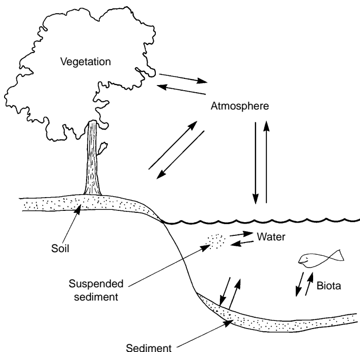
FIGURE 15.1 Distribution of a chemical between phases in the environment, with various two-phase partition processes involved, e.g., atmosphere–water, sediment–water, biota–water.
