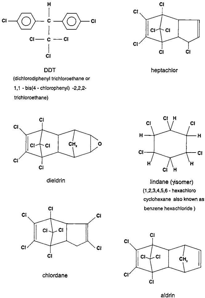
FIGURE 8.2 Examples of the chemical structures of some insecticides included in the chlorohydrocarbon group.
