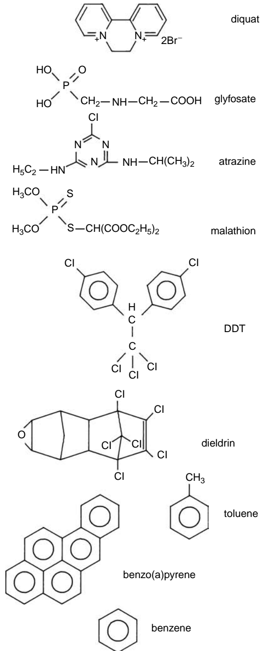
FIGURE 14.1 Chemical structure of some soil contaminants.
