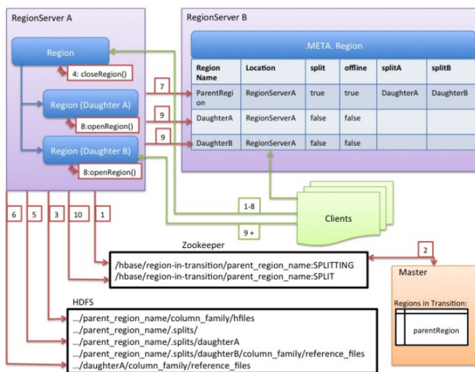
Figure 1. RegionServer Split Process
