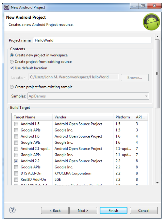
Figure 3-12 Eclipse's New Wizard: defining Android project options
