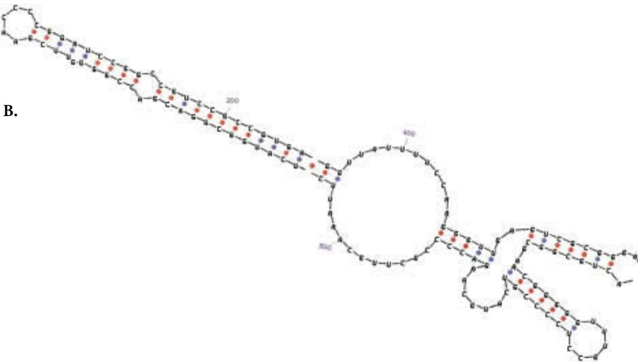
Figure 5.9. Model of RNA secondary structure of the human adenovirus pre-terminal protein. This model is one of several alternative structures represented by the above energy plot and provided as an output by the current versions of MFOLD. (A) Simple text representation of one of the predicted structures. Each stem-and-loop structure is shown separately and the left end of each structure is placed below the point of connection to the one above. (B) More detailed rendition of one part of the predicted structures. The structure continues beyond the right side of the page.
