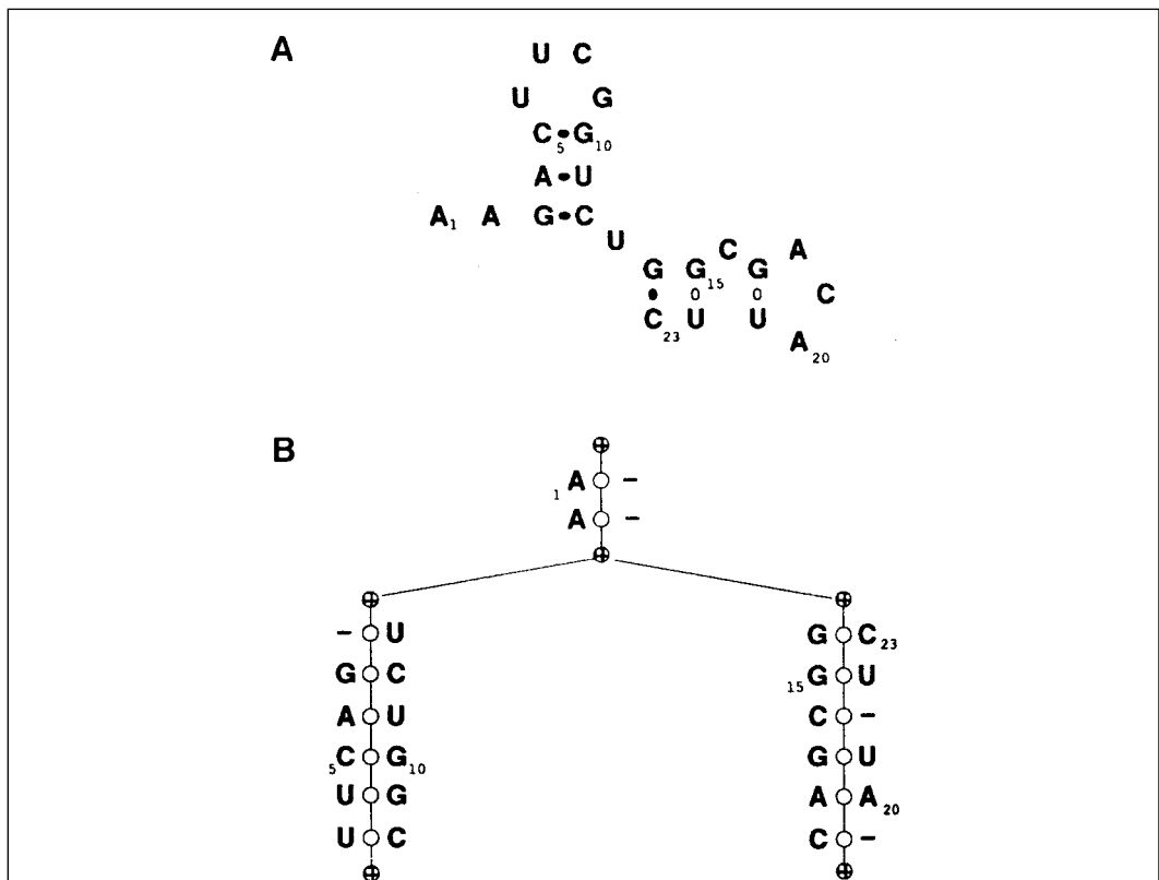
Figure 5.14. Tree model of RNA secondary structure. The model in A is represented by the ordered binary tree shown in B. This model attempts to capture both the sequence and the secondary structure of the RNA molecule. The tree is read like a sequence starting at the root node at the top of the model, then moving down the main branch to the bifurcation mode. Along the main trunk are nodes that represent matched or unmatched base pairs. Shown are two A's matching a "-", indicating no pairing with these bases. After the bifurcation mode, one then moves down the most leftward branch to the end node. Along the branch are unmatched bases, matched base pairs, and mismatched pairs. After the end node is reached, go back to the previous bifurcation node and follow the right branch. (Reprinted, with permission of Oxford University Press, from Eddy and Durbin 1994.)
