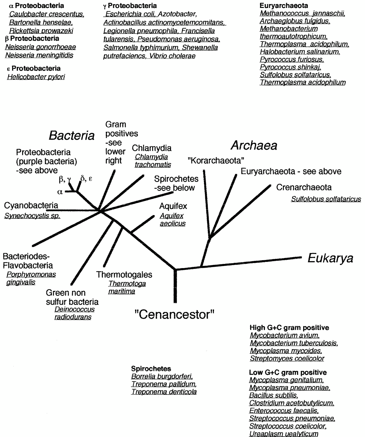
Figure 6.3. Rooted tree of life showing principal relationships among prokaryotic domains Bacteria and Archaea (Woese 1987; Barns et al. 1996; Brown and Doolittle 1997). Branch lengths are approximate only. Species that have been sequenced or are being sequenced are shown. A comprehensive database of sequenced microbial genomes is maintained at http://www.tigr.org/ .
