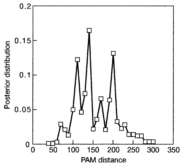
Figure 3.22. Posterior probability distribution of Dayhoff PAM scoring matrices for alignment of 1GKY and 2AK3-A.
