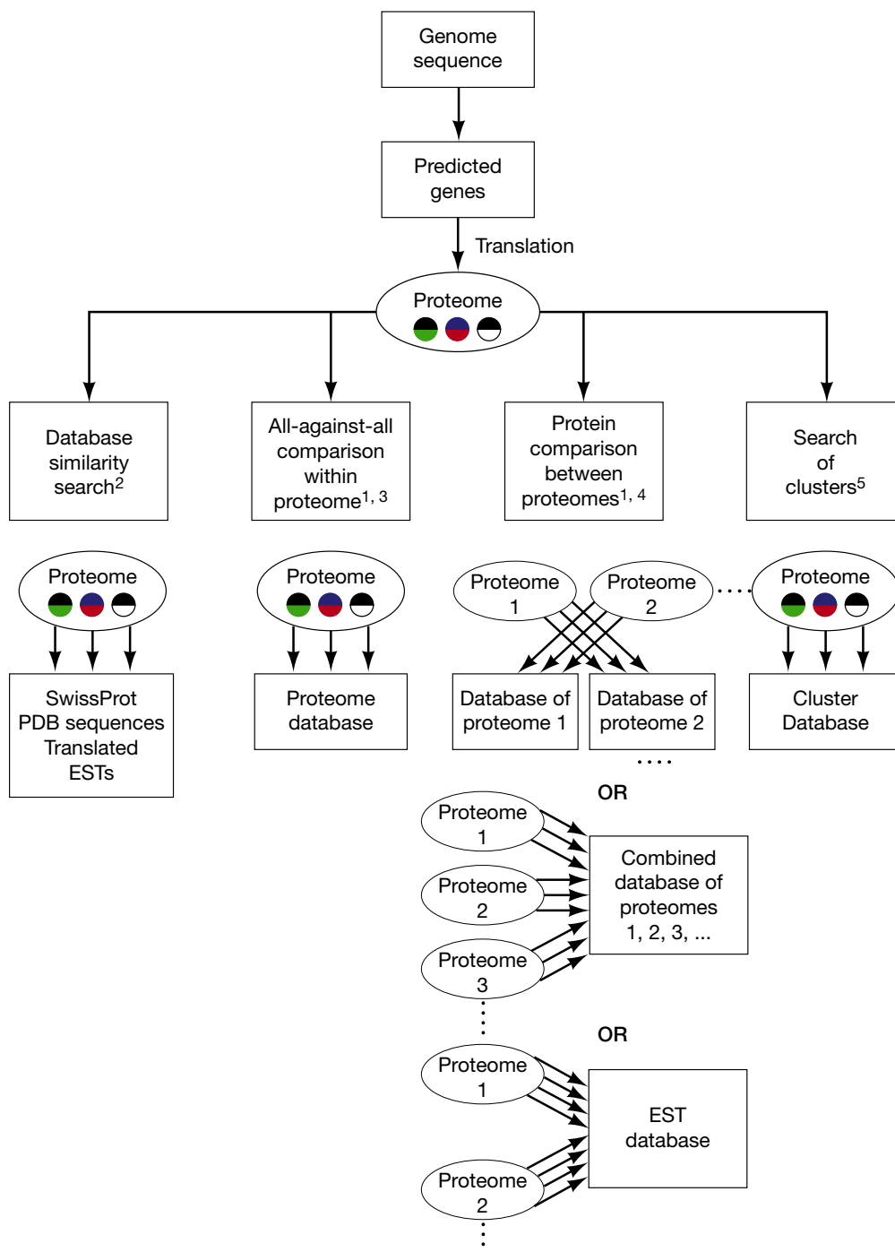
Figure 10.4. Analysis of the proteome encoded by genomes. (A) Types of proteome analyses. (B) Examples of database hits resulting from domain structure of proteins. (C) Cluster analysis of similar sequences. (D) Domain identification.
