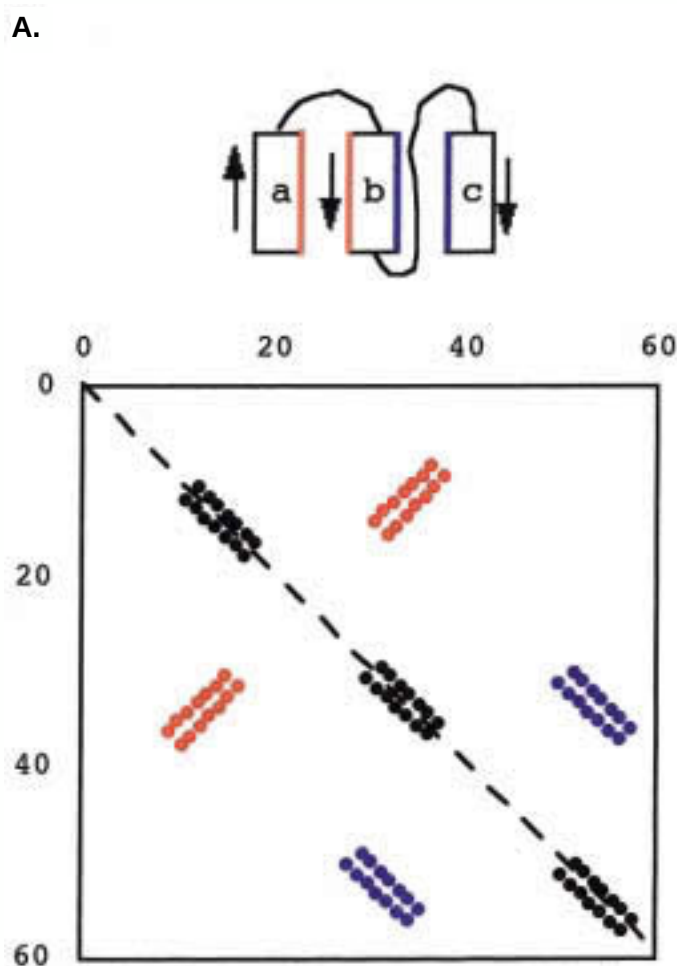
Figure 9.15. Distance matrix of hypothetical three-helix structure. (A) Matrix positions that represent closest distances of approximately <12 Å between the C_{\alpha} atoms in the known three-dimensional structures of the protein are marked by filling them with dots. Positions marked with black dots drawn just above the main downward-pointing diagonal ( dashed line ) from upper left to lower right represent amino acid sequential positions aa1-aa2, aa2-aa3, etc., that are close to each other because they are in the \alpha helix. Marked regions of shortest C_{\alpha} - C_{\alpha} distances along this diagonal thus indicate positions of the \alpha helices. Other marked diagonal regions ( red and blue dots ) indicate tertiary structural interactions, including those between adjacent secondary structural elements. Helices a and b are close to each other and have opposite chemical polarities so that aa10-aa11-aa12 . . . are close to aa40-aa39-aa38 . . . on the red surface of the helices. An upward-running diagonal ( red dots ) from lower left to upper right reveals this spatial relationship. Helices b and c are also close to each other but have the same polarity so that aa30-aa31-aa32 . . . are close to aa50-aa51-aa52 . . . , producing a downward-directed diagonal ( blue dots ). If another protein has a matrix pattern similar to that of the above example, then the two protein structures have the same three-helical arrangement and the loops joining the helices are of approximately the same length and conformation. The distance alignment method will find such three-helix patterns, even when the loop patterns are not similar. (B) Search for a common structural pattern in proteins A and B by DALI. A hypothetical example of a three-helix architecture is again used. In the top row, DALI first searches the entire distance matrix of protein A for a set of matching helices, a and b, indicated by an
