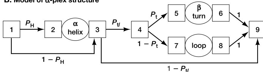
Figure 9.30. Hidden Markov model (discrete state-space model) of protein three-dimensional structure (from Stultz et al 1993; White et al. 1994). (A) Example of model for one of the basic structural elements, an \alpha helix. Squares indicate junctions in the model used to connect this model to models for other elements, including other \alpha helices, \beta strands, \beta turns, and loops. Circles represent hidden states in the model. Those circles labeled N (1 and 2) are amino-terminal amino acids, I (3) is an internal amino acid, and C (4 and 5) are carboxy-terminal amino acids in the \alpha helix. As in hidden Markov models that represent multiple sequence alignments, each of these states has a distribution of amino acids as found in aligned structures. For example, the frequency of H in an amino-terminal position in an \alpha helix is 0.015, whereas in a carboxy-terminal amino acid, it is 0.028 in the proteins modeled by Stultz et al. (1993). At portions of internal amino acids, additional amino acids may be added to the \alpha model. Arrows indicate a path to be followed through the states of the model, starting and ending with a numbered junction. Usually, the transition probability from one state to the next is 1, but at internal positions two alternative transition probabilities are possible, one ( P ) adds only one internal amino acid, whereas a second adds an additional internal amino acid with probability 1 - P . (B) Model for a particular structural complex includes elements such as the \alpha -helix model described in A. This particular model is of an \alpha -helix complex named an \alpha plex. These plexes are then combined to produce a model of a three-dimensional structural domain. The oval \alpha helix is a condensed representation of the finite-state \alpha -helix model shown in A with functions at each end. Similar oval representations for models of a \beta turn and a loop are also shown in this example. The arrows between junctions indicate transitions from one type of plex to another, and in several places there are two to three alternative possibilities in this model. Note that the plex can start with an \alpha helix with transition probability P_H , but can also skip the \alpha helix with probability 1 - P_H . The remaining paths in the model include the possibilities of an \alpha turn, a loop, or of no further elements. To turn domain models into a predictive tool, they are trained on a set of known proteins of that type. In this procedure, transitional probabilities between junctions, states, and plexes are adjusted using the sequences and structures of the training sequences until the model is optimal for distinguishing those domains from other types of domains. A structural prediction for a new protein sequence is then made by finding the most probable path of the sequence through a set of domain models and choosing the model that gives the best alignment with the new sequence. The procedure of calculating the probability of paths through each structural model and of finding the most probable path is similar to that used for sequence alignment models discussed in Chapter 4 (see Fig. 4.16 on p. 186). Only a limited number of domains have been modeled by this approach.
