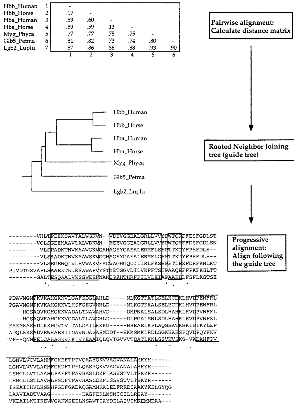
Figure 4.9. A msa of seven globins by CLUSTALW. The protein identifiers are from the SwissProt database. The amino acid substitution matrix was the Dayhoff PAM250 matrix, and gap penalties were varied to emphasize conserved ungapped regions. The approximate and known locations of seven \alpha -helices in the structure of this group are shown in boxes. (Reprinted, with permission, from Higgins et al. 1996 [copyright Academic Press].)
