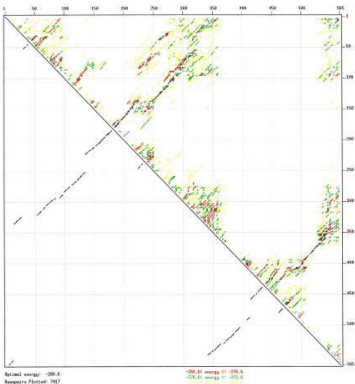
Figure 5.8. The energy dot plot (boxplot) of alternative choices of base pairs of an RNA molecule (Jacobson and Zuker 1993). The sequence is that of a human adenovirus pre-terminal protein (GenBank U52533) that is given by M. Zuker as an example on his Web site at http://bioinfo.math.rpi.edu/~zukerm . Foldings were computed using the default parameters of the MFOLD program at http://bioinfo.math.edu/~mfold/rna/form1.cgi (Mathews et al. 1999) using the thermodynamic values of SantaLucia (1998). The minimum energy of the molecule is -280.6 kcal/mole and the maximum energy increment is 12 kcal/mole. Black dots indicate base pairs in the minimum free-energy structure and are shown both above and the mirror image below the main diagonal. Red, blue, and yellow dots are base pairs in foldings of increasing 4, 8, and 12 kcal/mole energies greater than the minimum energy, respectively. A region with very few alternative base pairs such as the pairing of 370–395 with 530–505 is considered to be strongly predictive, whereas regions with many alternative base pairs such as the base-pairing in the region of 340–370 with 570–530 are much less predictive.
