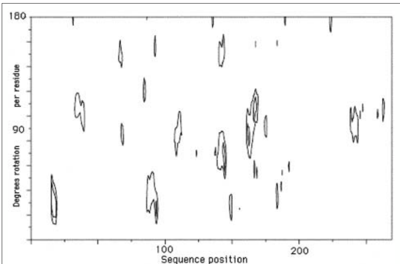
Figure 9.28. Hydrophobic moment plot of the sequence of the \alpha chain of E. coli tryptophan synthase using the Genetics Computer Group MOMENT program. The moment uses the hydrophobicity values shown in Table 9.6 to measure the tendency of hydrophobic residues to be located on one face of a secondary structural element (Lüthy and Eisenberg 1991). The values are normalized so that the mean value is 0 and the standard deviation is 1. The moment is calculated for a window of 10 residues, 5 on each side of every amino acid position and for every possible rotational angle between adjacent residues. The angle is 100^\circ for \alpha helices and 160^\circ for \beta strands. When one contour is shown, the moment values are 0.35; when two contours are shown, values are 0.35 (outer) and 0.45 (inner).
