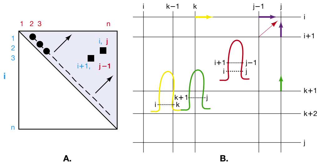
Figure 5.7. Method used in dynamic programming analysis for identifying the most energetically favorable configuration of a linear RNA molecule. (A) The sequence of an RNA molecule of length n bases is listed across the top of the page and down the side. The index of the sequence across the top is j and that down the side is i . The search only includes the upper right part of the matrix shown in gray and begins at the first diagonal line for matching base pairs. First positions i = 1 and j = 2 are compared for potential base-pairing, and if pairing can occur, an energy value is placed in an energy matrix W at position 1,2. Then, i = 2 and j = 3 base are compared, and so on, until all base combinations along the dashed diagonal have been made. Then, comparisons are made along the next upper right diagonal. As each pair of bases is compared, an energy calculation is made that is the optimal one up to that point in the comparison. In the simplest case, if i + 1 pairs with j - 1 , and i pairs with j , and if this structure is the most favorable up to that point, the energy of the i/j base pair will be added to that of the i + 1/j - 1 base pair. Other cases are illustrated in B. The process of obtaining the most stable energy value at each matrix position is repeated following the direction of the arrows until the last position, i = 1 and j = n , has been compared and the energy value placed at this position in matrix W , the value entered in W(1,n) , will be the energy of the most energetically stable structure. The structure is then found by a trace-back procedure through the matrices similar to that used for sequence alignments. The method used is a combination of a search for all possible double-stranded regions and an energy calculation based on energy values similar to those in Table 5.2. The search for the most energetic structure uses an algorithm (Zuker and Stiegler 1981) similar to that for finding the structure with maximum base-pairing (Nussinov and Jacobson 1980). These authors recognized that there are three possible ways, illustrated here by the colored arrows, of choosing the best energy value at position i,j in an energy matrix W . The simplest calculation (red arrow) is to use the energy value found up to position i - 1, j - 1 diagonally below i,j . If i and j can form a base pair (and if there are at least four bases between them in order to allow enough sequence for a hairpin) and i + 1 and j - 1 also pair, then the stacking energy of i/j upon i + 1/j - 1 will reduce the energy value at i + 1, j - 1 , producing a more stable structure, and the new value can be considered a candidate for the energy value entered at position i,j . If i and j do not pair, then another choice for the energy at i,j is to use the values at positions i, j - 1 or i + 1, j illustrated by the blue arrows. i and j then become parts of loop structures. Finally, i and j may each be paired with two other bases, i with k and j with k + 1 , where k is between i and j ( i < k < j ), illustrated by the structure shown in yellow and green, reflecting the location of the paired bases. The minimum free-energy value for all values of k must be considered to locate the best choice as a candidate value at i,j . Finally, of the three possible choices for the minimum free-energy value at i,j indicated by the four colored arrows, the best energy value is placed at position W(i,j) . The procedure is repeated for all values of i and j , as illustrated in A. Besides the main energy scoring matrix W , additional scoring matrices are used to keep track of auxiliary information such as the best energy up to i,j where i and j form a pair, and the influence of bulge loops, interior loops, and other destabilizing energies. An essential second matrix is V(i,j) , which keeps track of all substructures in the interval i,j in which i forms a base pair with j . Some values in the W matrix are derived from values in the V matrix and vice versa (Zuker and Stiegler 1981).
