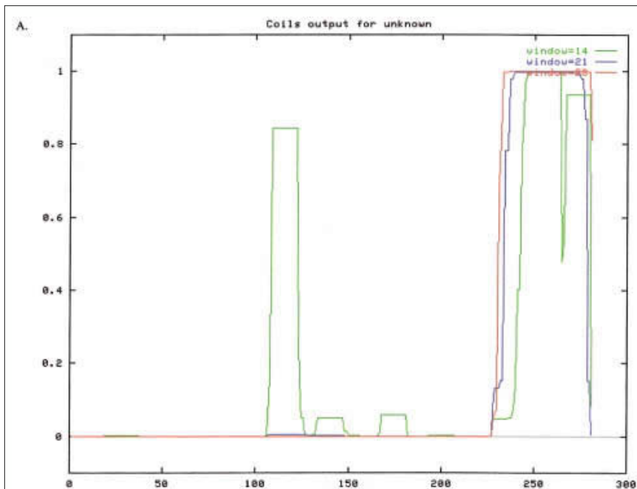
Figure 9.21. Prediction of coiled-coil regions by the COILS2 program. The Gcn4 protein was used as input to a Web page listed in the text. (A) Plot of probability of residue in coiled-coil structure versus residue number obtained from the ISREC server. (B) Partial list of scores by residue number. Analysis obtained from the Predict Protein server. Note that highest probabilities are obtained with a window of 28 amino acids. The expected order of amino acids in the coiled coil is a, b, c, d, e, f, and g. This order does not start until residue 244. Amino acids found at position 243 and at lower numbered positions are characteristically found at other places in the coiled-coil heptad.
