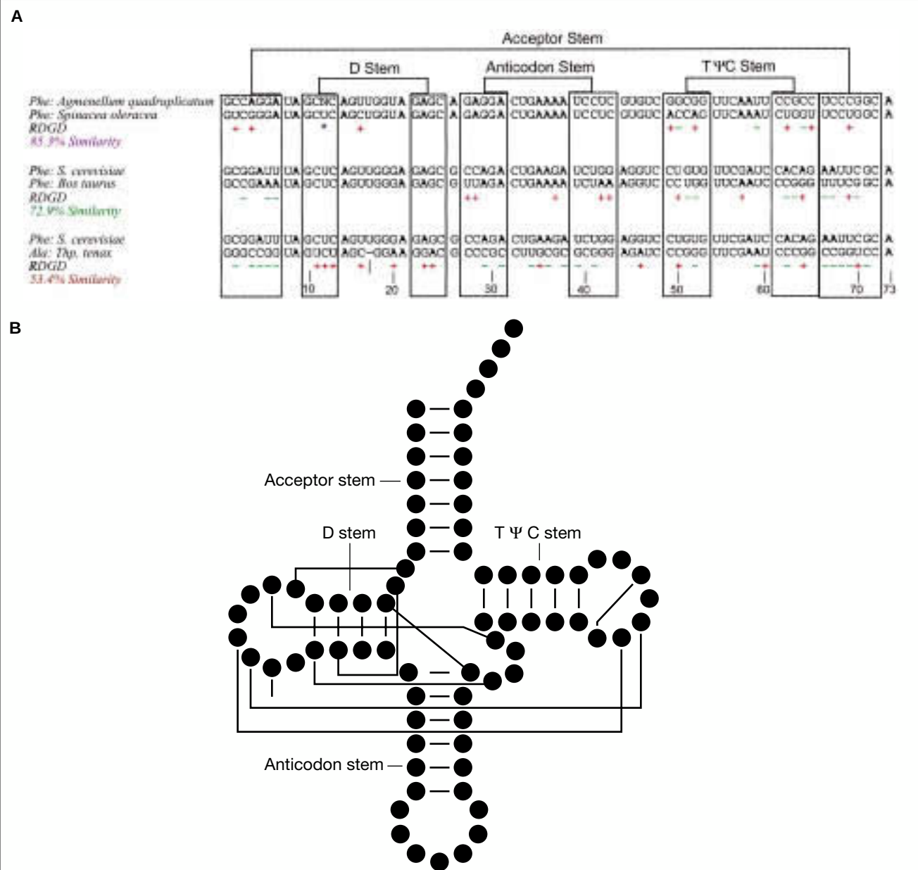
Figure 5.12. Covariation found in tRNA sequences reveals base interactions in tRNA secondary and tertiary structure. (A) Alignment of tRNA sequences showing regions of interacting base pairs. (+) Transition; (−) transversions; (|) deletion; (*) ambiguous nucleotide. (B) Diagram of tRNA structure illustrating base–base interactions revealed by a covariance analysis. Adapted from the Web site of R. Gutell at http://www.rna.icmb.utexas.edu .
