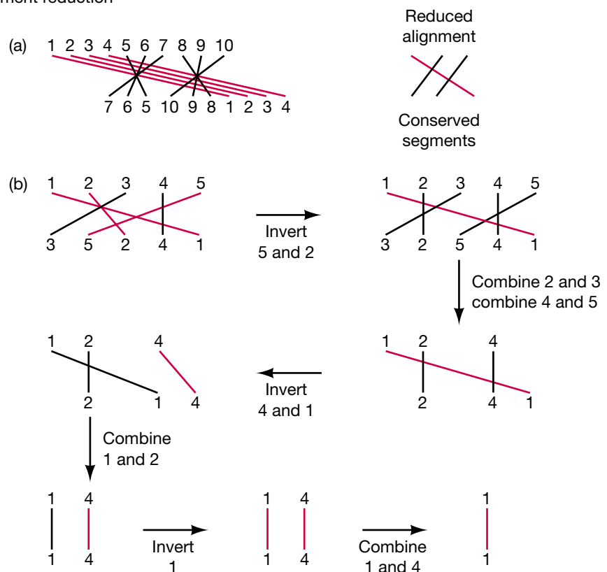
Figure 10.8. Computational analysis of genome arrangements. (A) In aligning two sequences, one sequence is written above the other and the highest number of consecutive matches between the sequences provides an optimal alignment as described in Chapter 3. The alignment includes matches ( solid lines ), mismatches ( dotted lines ), and insertions/deletions in order to produce an optimal number of matches. The matches are in a consecutive order in two sequences such that no rearrangements would be found. (B) Alignments of linear and circular chromosomes that have undergone rearrangements such as those found in mammalian chromosomes and mitochondria. In contrast to sequence alignment, lines indicating homologous positions in linear chromosomes ( left ) now cross, producing points of intersection. The more rearrangements there are, the more intersections will occur. For alignment of circular chromosomes ( right ), depending on how the chromosomes are aligned, there are two ways of showing a moved region. To go from A on the outer genome to A on the inner genome,
