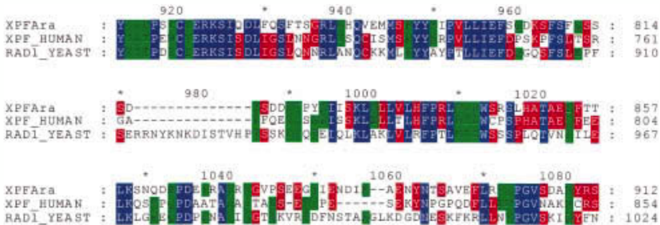
Figure 4.20. GeneDoc, a multiple sequence alignment editor with many useful features. Shown is an illustrative multiple sequence alignment of three DNA repair genes similar to the S. cerevisiae Rad1 gene. The sequences were aligned with CLUSTALW, and the FASTA-formatted alignment (Chapter 2) was imported into GeneDoc on a PC.
