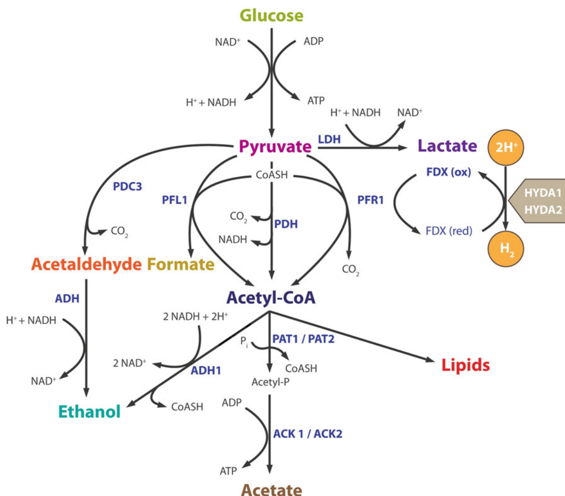
Fig. 3.9 Proposed metabolic pathways leading to the secretion of the indicated metabolites during anoxia. Pyruvate can be metabolized to acetyl-CoA via pyruvate ferredoxin oxidoreductase (PFR) yielding acetyl-CoA, reduced ferredoxin and CO 2 . Alternatively, pyruvate can be cleaved by pyruvate formate lyase (PFL) yielding acetyl-CoA and formate. The [FeFe]-hydrogenases (HYDA1, HYDA2) can then be reduced by FDX, catalyzing H 2 production. Pyruvate may also be decarboxylated by the pyruvate decarboxylase pathway (PDC) result-
