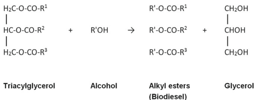
Scheme 12.1 The transesterification reaction. The feedstock, be it a vegetable oil, animal fat or algal oil, is represented by the triacylglycerol
