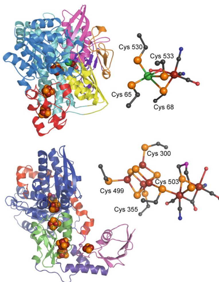
Fig. 3.2 (Top) Ribbon/space filling representation of the [NiFe]-hydrogenase from D. gigas (PDB code 1YQ9) and active site (right) in ball and stick representation. CO and CN - ligands are present at the [NiFe] active site in addition to a bridging species depicted as a peroxide ligand for the oxidized “unready” state of the enzyme. (Bottom) Ribbon/space filling representation of the [FeFe]-hydrogenase Cpl (PDB code 3C8Y) and active site H-cluster (right) in ball and stick representation.
