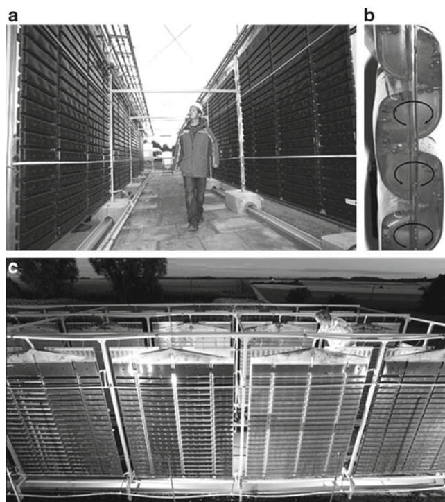
Fig. 7.1 Flat Panel Airlift reactor developed by Subitec GmbH. (a) Pilot plant in Hamburg-Reitbrook developed in cooperation with E.ON Hanse AG. (b) Side view of the panel with inbuilt baffles for induction of vortices (Courtesy of Subitec GmbH, ©Thomas Ernsting) (c) Plant in Eutingen-Weitingen (Stuttgart) developed in cooperation with EnBW AG
