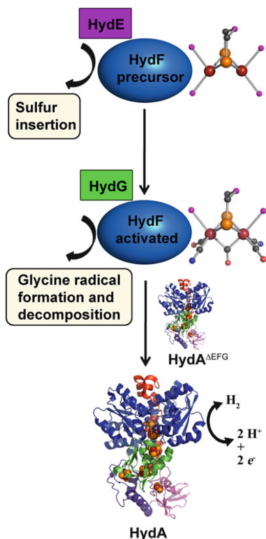
Fig. 3.4 H-cluster biosynthesis process for [FeFe]-hydrogenases. The 2Fe subcluster is proposed to be assembled on HydF which serves as a chemical scaffold for the process. Radical SAM enzyme HydE is proposed to modify a basic [2Fe-2S] cluster with a dithiolate ligand in the first step, followed by further cluster modification with addition of CO and CN - ligands by the radical SAM enzyme HydG from the substrate tyrosine. In the final step, activation and maturation is achieved by transfer of the ligand modified 2Fe subcluster to the immature structural protein (HydA ΔEFG ), which already contains the [4Fe-4S] cluster of the H-cluster
