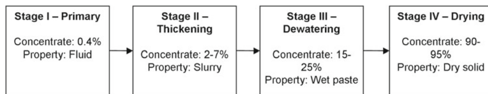
Fig. 10.2 Block flow diagram for the recovery of microalgae biomass, showing typical biomass concentration achieved and the physical state of the output stream
