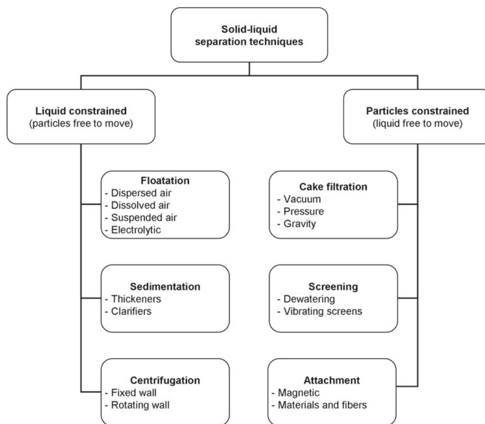
Fig. 10.1 Common industrial solid-liquid separation techniques
