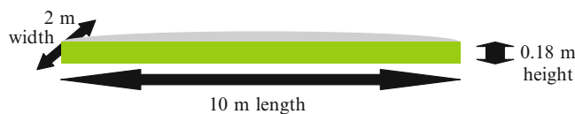
Fig. 14.3 Design and dimensions of one plastic photobioreactor
