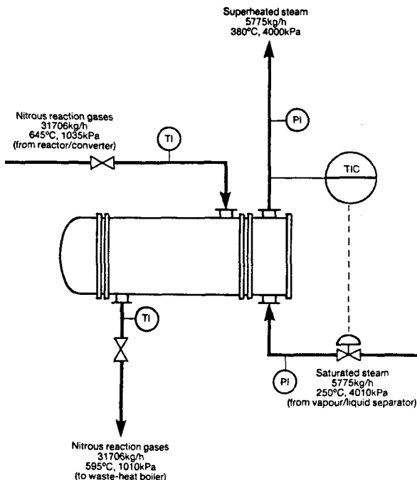
FIGURE 10.2 Steam superheater process-control scheme.
