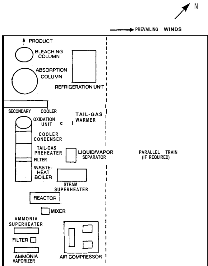
FIGURE 5.5 Nitric acid plant layout.
