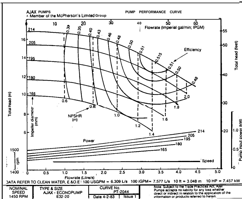
FIGURE 1.2 Pump performance curves for AJAX 'E' range pump E32-20. (Reproduced with permission.)
