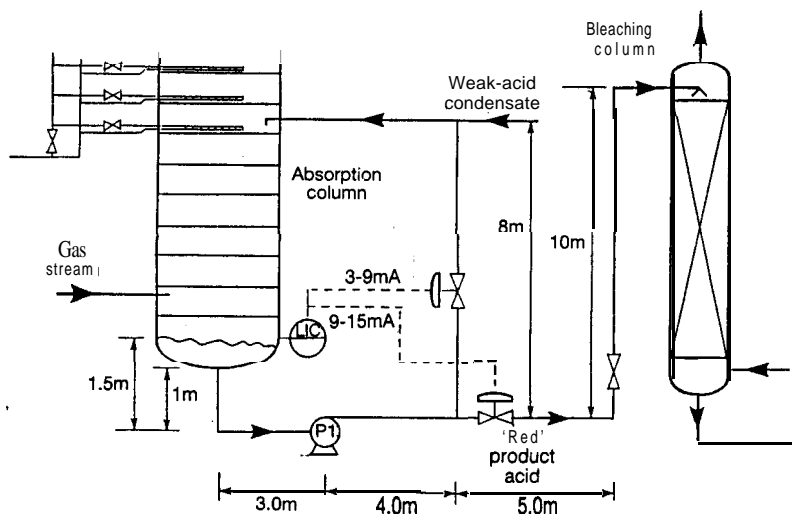
FIGURE 11.1 Flowsheet for pump specification.
