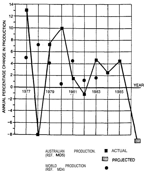
FIGURE B.3 Percentage change in production of nitric acid (100% basis),
