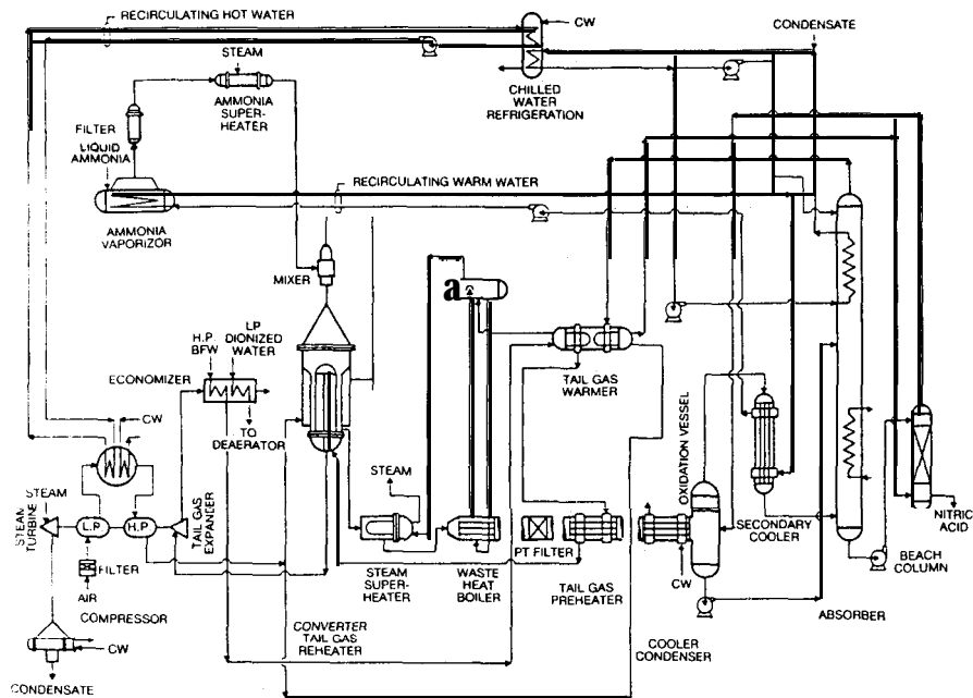
FIGURE 3.2 Flowsheet for single-pressure nitric acid process. (From Ref. PTI, p. 177; reproduced with permission from American Institute of Chemical Engineers.)
