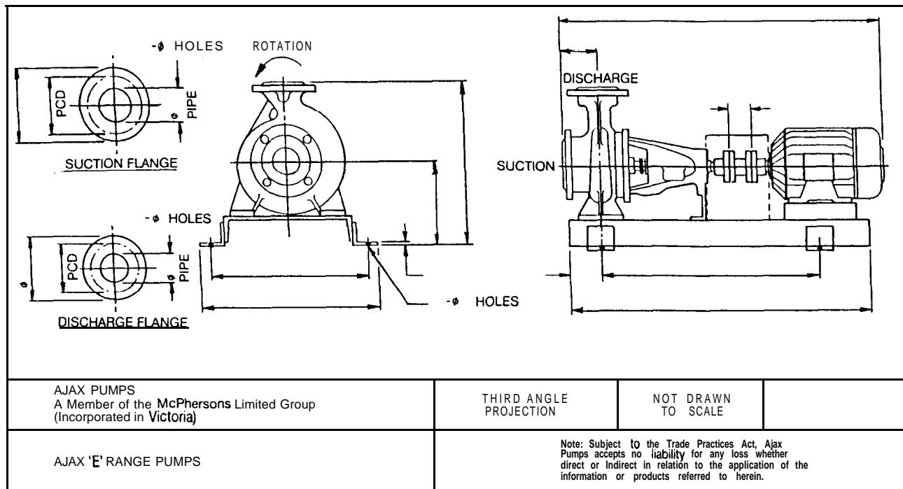
FIGURE 1.1 General drawing of AJAX 'E' range pumps. (From manufacturer's technical catalogue, reproduced with permission.)
