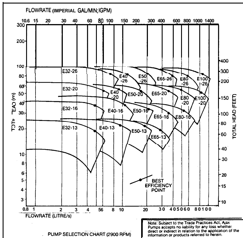
FIGURE I.5 Pump selection chart for AJAX 'E' range pumps.
