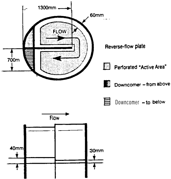
FIGURE 9.3 Sieve-plate specification: Plates above the weak-acid feed plate.
