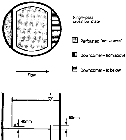
FIGURE 9.2 Sieve-plate specification: Plates at or below the weak-acid feed plate.
