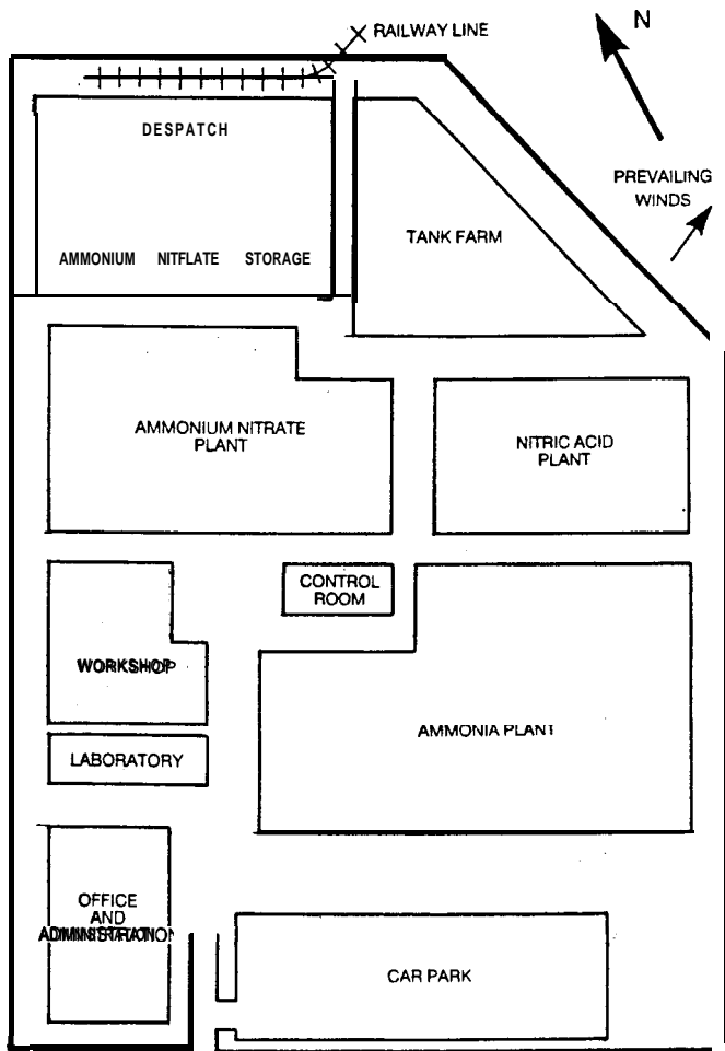
FIGURE 5.4 Overall chemicals-complex layout.
