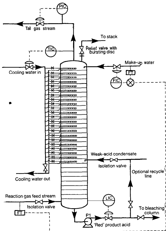
FIGURE 9.6 Control scheme for NO x absorption column.
