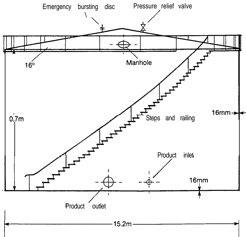
FIGURE 12.1 Nitric acid storage tank.
