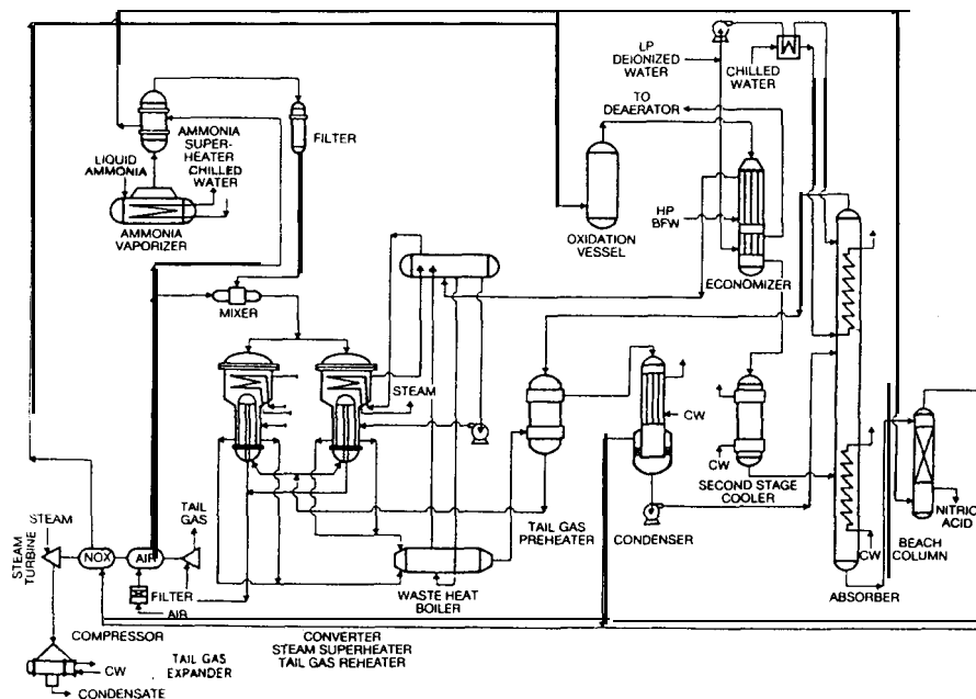
FIGURE 3.1 Flowsheet for dual-pressure nitric acid process. (From Ref. PT I, p. 176; reproduced with permission from American Institute of Chemical Engineers)
