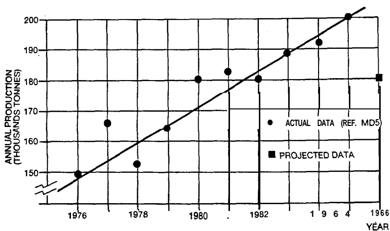
FIGURE B.1 Australian production trend for nitric acid.
