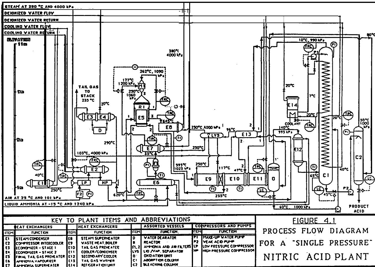
FIGURE 4.1 Process flow diagram for a 'single-pressure' nitric acid plant.
