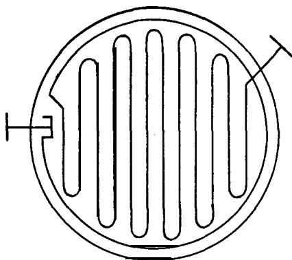
FIGURE 9.4 Herringbone cooling coils (two coils per sieve plate)
