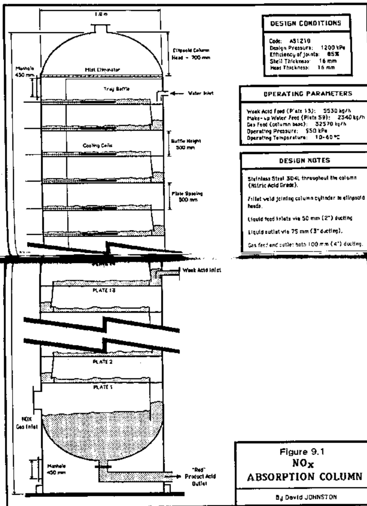
FIGURE 9.1 NO x absorption column
