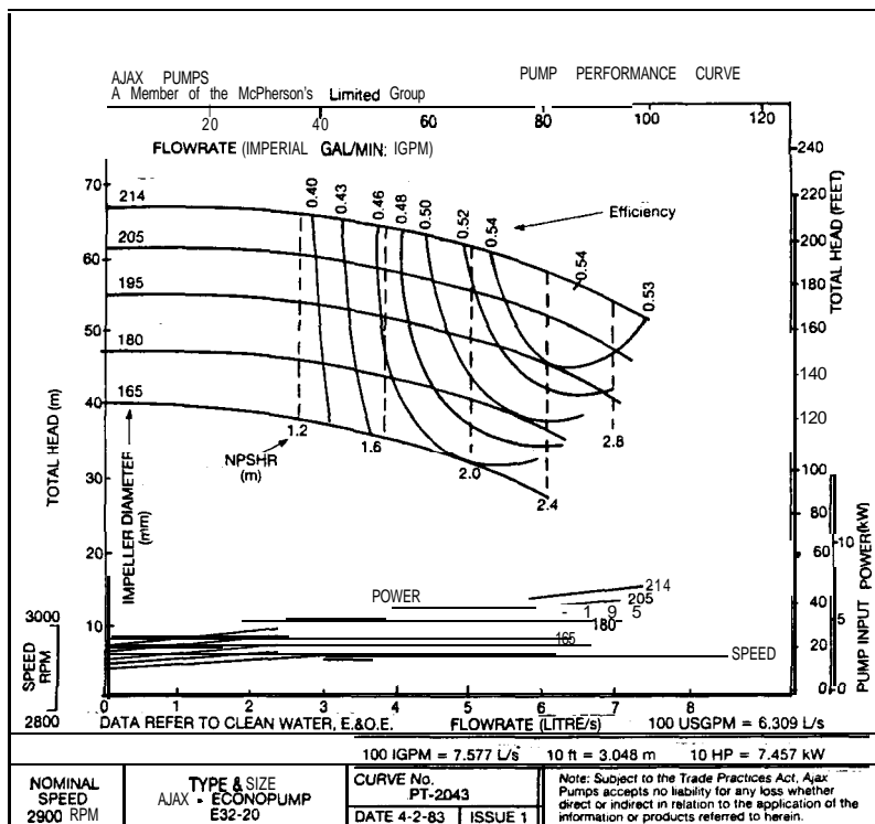
FIGURE I.3 Pump performance curves for Ajax 'E' range pump E32-20. (Reproduced with permission.)
