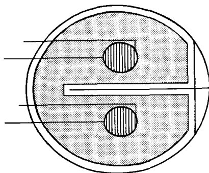
FIGURE 9.4 Herringbone cooling coils (two coils per sieve plate)
