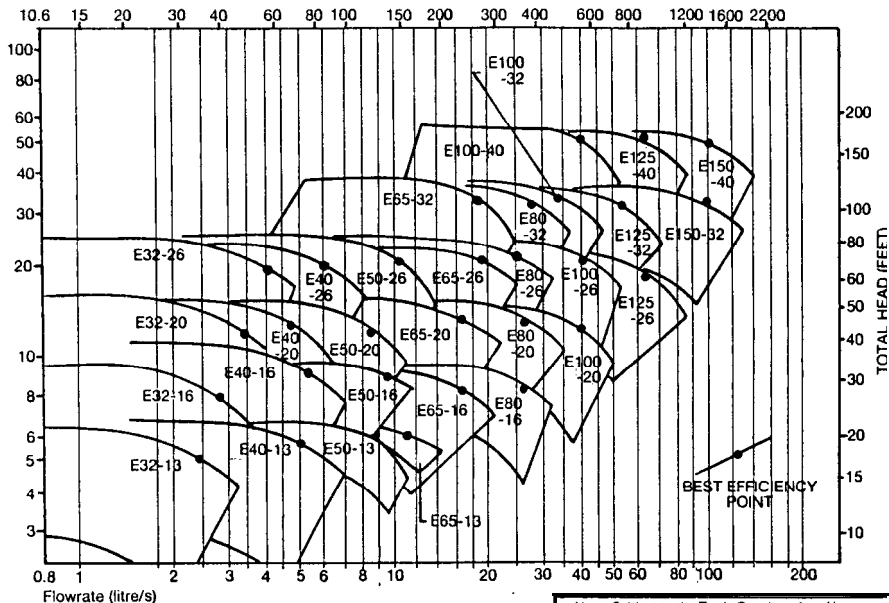
PUMP SELECTION CHART (1450 RPM)
