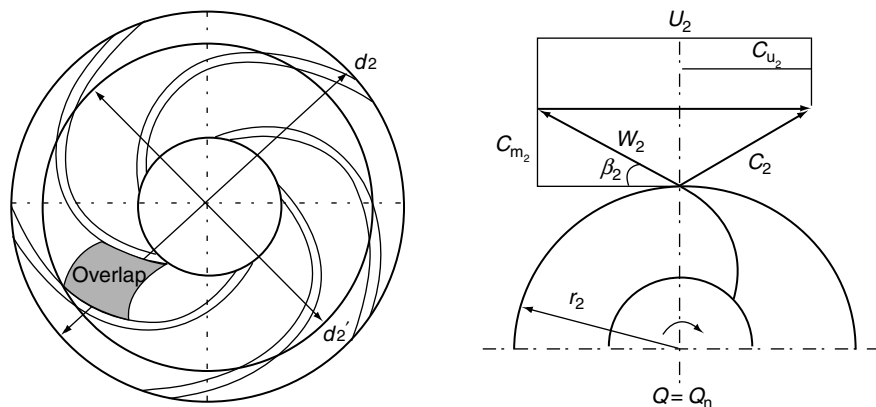
Figure 5.21 Impeller trimming
