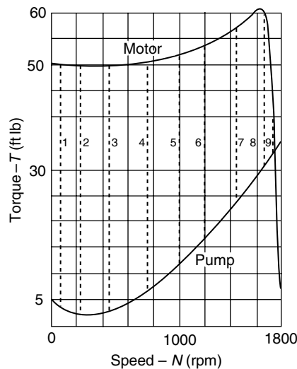
Accelerating torques from Figure 5.20
