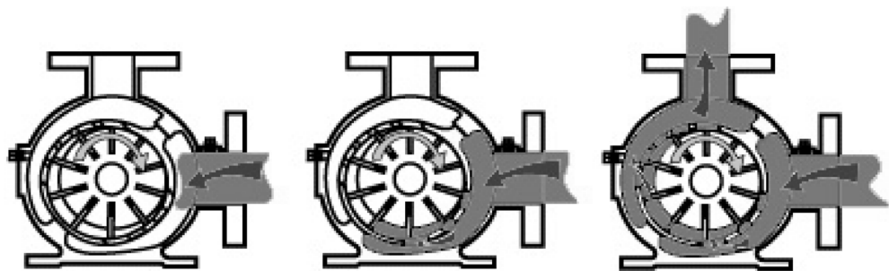
Figure 1.11 Vane pump
