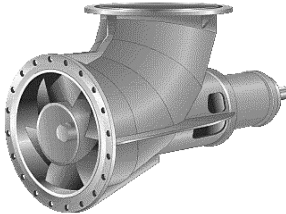
Figure 2.10 Mixed flow impeller and propeller vaned mixed flow type impeller
