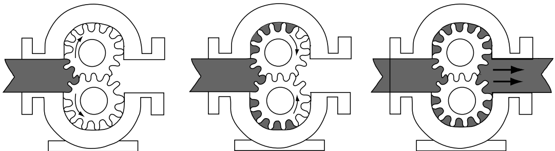
Figure 1.8 External gear pump
