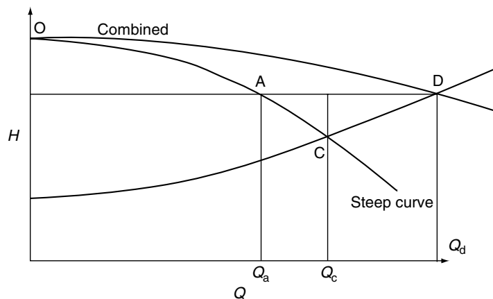
Figure 5.14 Pumps with steep curves
