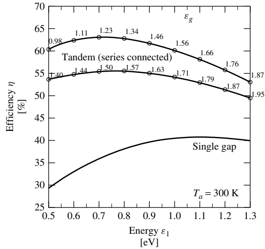
Figure 4.15 Limiting efficiency for the IB solar cell under maximum concentrated sunlight. For comparison, the limiting efficiency of single-gap solar cells (in this case, \varepsilon_l \equiv \varepsilon_g ) and a tandem of two cells that are series-connected are also shown (in this case, \varepsilon_l labels the lowest band gap of the cells and the figures on the curve correspond to the highest of the band gaps). (Reproduced from Increasing the Efficiency of Ideal Solar Cells by Photon Induced Transitions at Intermediate Levels , Luque A. and Martí A., Physical Review Letters V. 78 N. 34, 5014–5017, by permission of American Physical Society © 1997)
