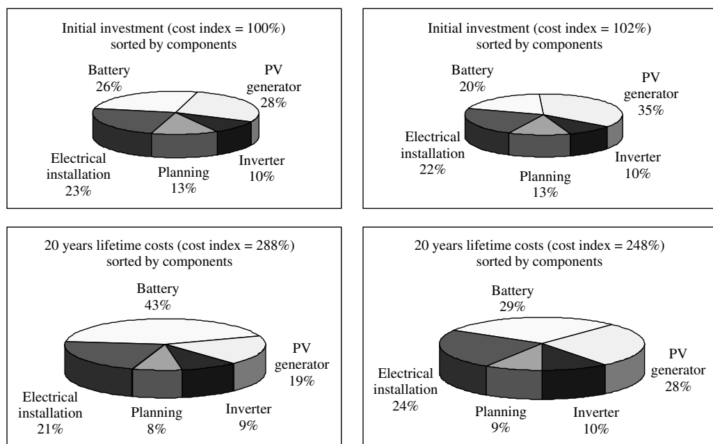
Figure 18.31 Comparison of costs for a PV battery system derived under different assumptions. Left-side graphs show the costs for the system optimised by initial investment costs, right-side graphs show the costs for a system optimised by lifetime costs. The overall costs for the initial investments (upper graphs) and the overall lifetime costs (lower graphs) calculated according to the annuity method are normalised to the initial investment costs for the system optimised by initial investment (cost index = 100%). Location, Mexico; annual power consumption, 1500 kWh; effective interest rate, 6%; lifetime of components: PV generator 20 years, electronic components 15 years, battery according to sizing and operating conditions, calculations and optimisation done with the simulation tool TALCO[42]
