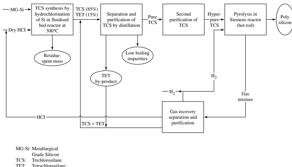
Figure 5.2 Schematic representation of the Siemens process
