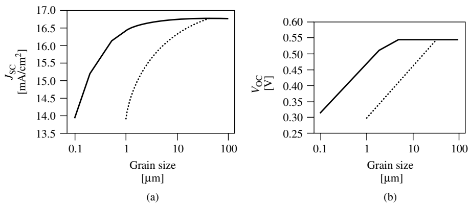
Figure 8.24 Calculated dependence of (a) J_{sc} ; and (b) V_{oc} on the grain size of the 10- \mu\text{m} -thick cell for two values of interface recombination velocity, 100 \text{cm/s} (solid lines) and 1000 \text{cm/s} (dotted lines)
