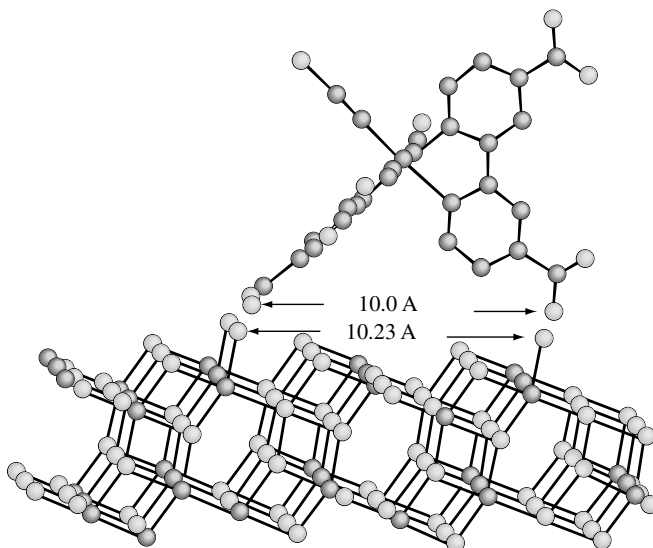
Figure 15.5 Anchoring structure of N3 dye adsorbed on the (101) surface of TiO 2 : the top is N3 dye and the bottom is TiO 2 . Reprinted with permission from © (2002) American Chemical Society
