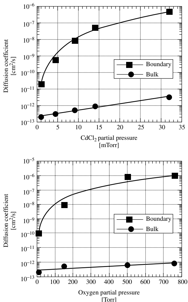
Figure 14.18 Sensitivity of bulk and grain-boundary diffusion coefficients (a) to \text{pCdCl}_2 at constant \text{pO}_2 \sim 125 Torr, at T = 420^\circ\text{C} , and (b) to \text{pO}_2 at constant \text{pCdCl}_2 = 9 mTorr, at T = 420^\circ\text{C}
