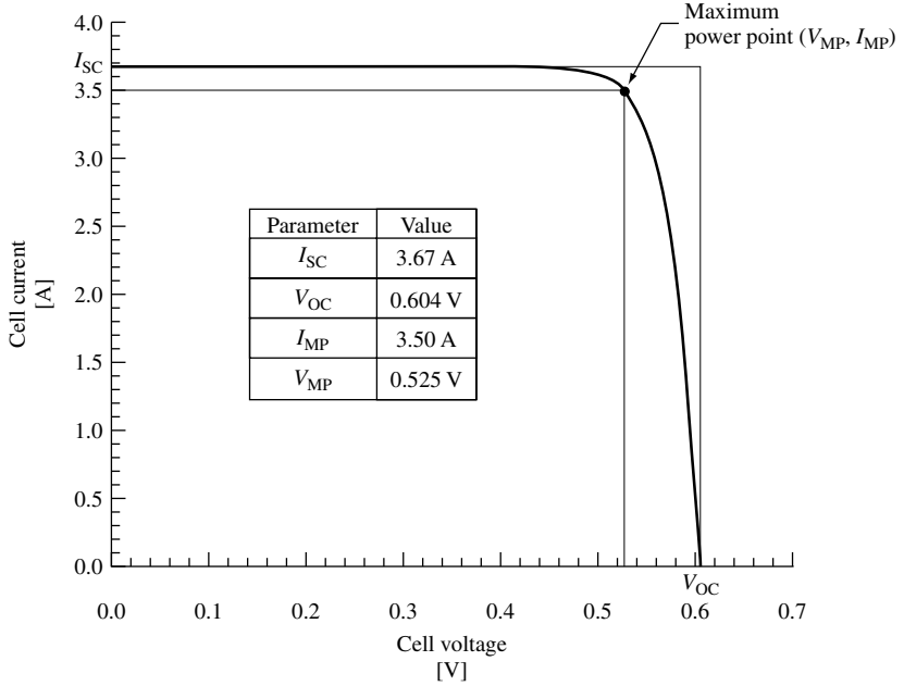
Figure 3.16 Current–voltage characteristic of the silicon solar cell defined by Table 3.2
