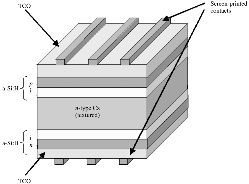
Figure 7.14 Structure of the HIT cell
