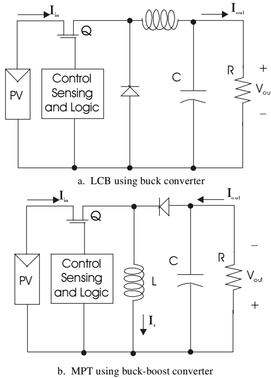
Figure 3.28 Maximum power tracker and linear current booster.
