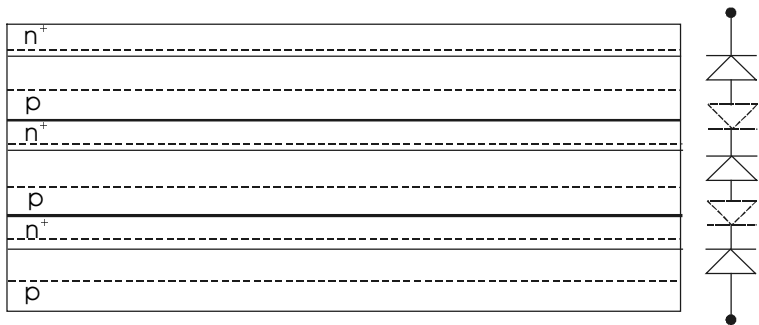
Figure 10.19 Three junctions in tandem (series), showing opposing pn junctions.
