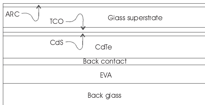
Figure 11.15 Basic structure of a CdTe PV cell [35]. (Adapted from Ullal et al., Proc 26th IEEE PV Spec Conf , 1997, 301, © 1997 IEEE.)
