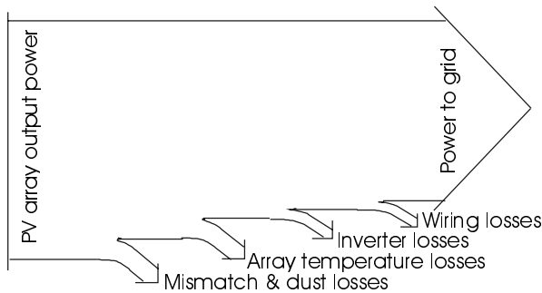
Figure 8.5 Loss mechanisms between module output and inverter output.
