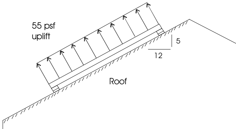
Figure 6.13 Standoff-mounted array with an uplifting pressure distribution.
