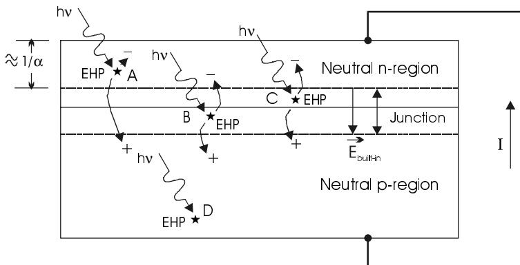
Figure 10.8 The illuminated pn junction showing desirable geometry and the creation of electron-hole pairs.
