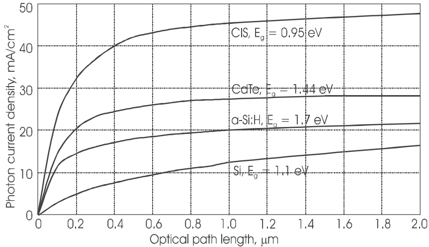
Figure 11.1 Photon current vs. optical path length for thin film materials, compared with crystalline silicon, standard test conditions [2].
