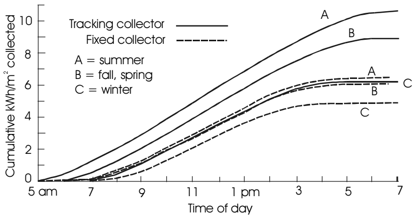
Figure 2.10 Cumulative daily irradiation received by fixed and tracking collectors for different seasons, direct beam contribution only.
