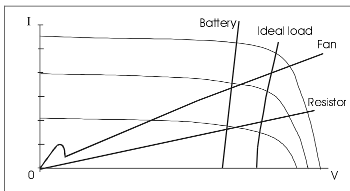
Figure 3.15 I-V characteristics for several common loads along with ideal load I-V characteristic for maximum power operation of a PV system.
