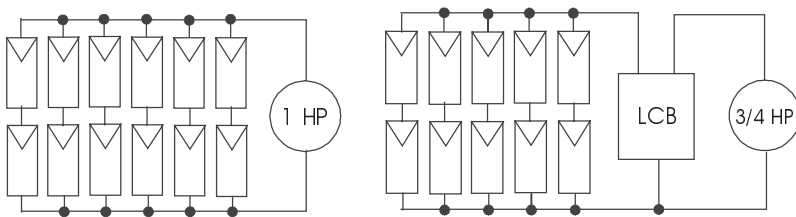
Figure 4.6 24 V dc water pumping systems.
