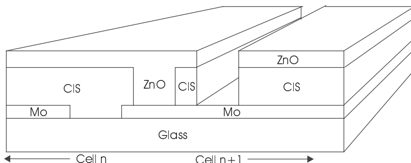
Figure 11.14 Siemens monolithic method of series cell connection [37].
