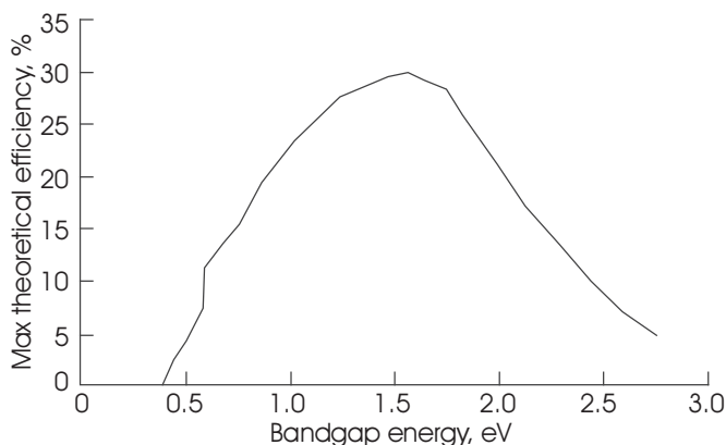
Figure 11.17 Theoretical maximum PV cell efficiency vs. bandgap [53].
