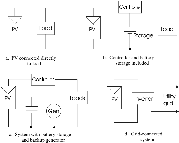
Figure 3.2 Examples of PV systems.
