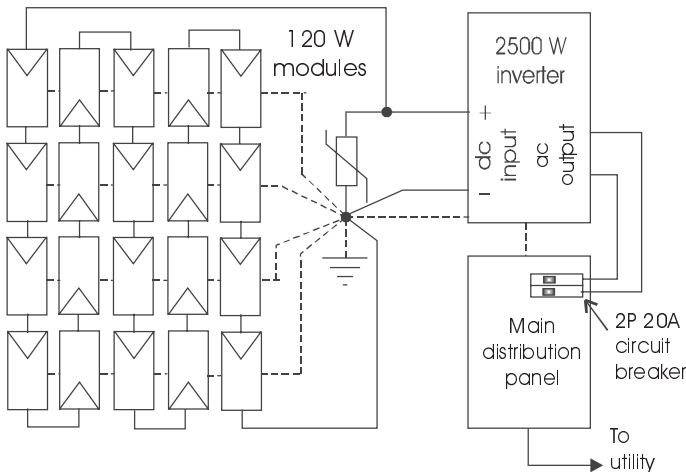
Figure 4.11 A 2.4-kW utility interactive system connected on the customer side of the utility meter.
