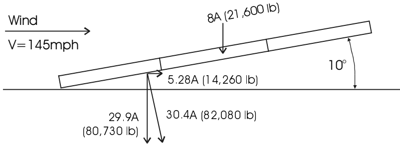
Figure 8.17 Mechanical forces acting on the PV array. The values in parentheses are for a 20-parking-space canopy.
