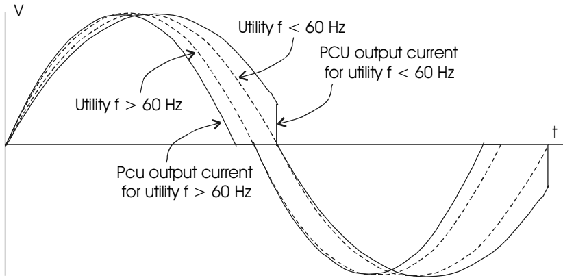
Figure 8.1 Comparison of utility voltage and PCU current for under-frequency and over-frequency utility voltage.
