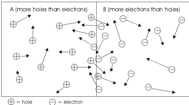
Figure 10.6 Random thermal motion and diffusion for electrons and holes.
