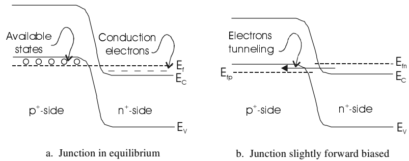
Figure 10.20 Tunnel junction showing conditions necessary for tunneling.
