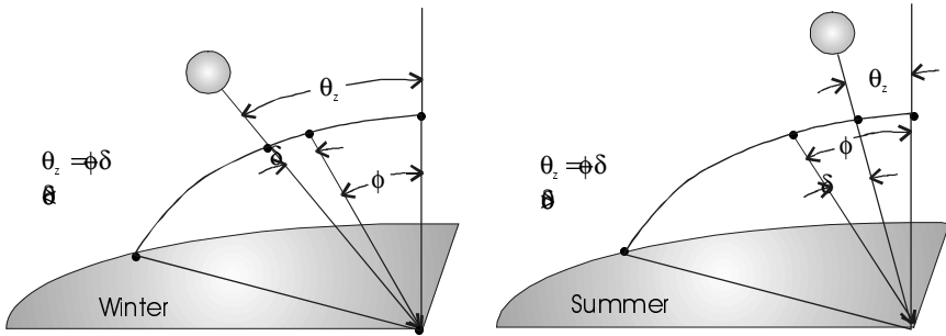
Figure 2.4 Relationships among \theta_z , \phi , and \delta at solar noon in winter and summer.
