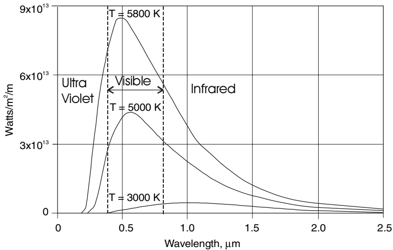
Figure 2.1 Blackbody radiation spectra for temperatures of 3000 K, 5000 K and 5800 K.
