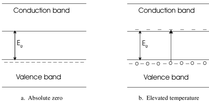
Figure 10.1 Illustration of availability of states in valence band and conduction band for semiconductor material.
