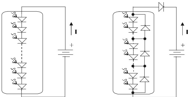
a. Module without blocking or bypass diodes b. Module with blocking and bypass diodes
