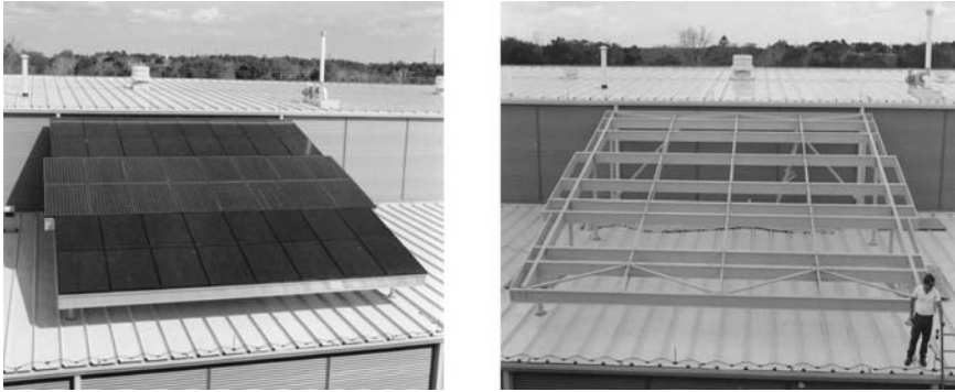
Figure 6.16 A rack-mounted array at the Florida Solar Energy Center. The robust structural system is designed to withstand category 3 hurricanes.
