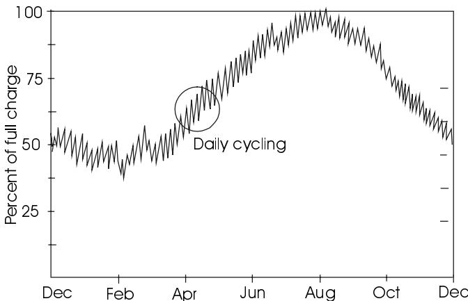
Figure 3.20 Seasonal battery cycling.
