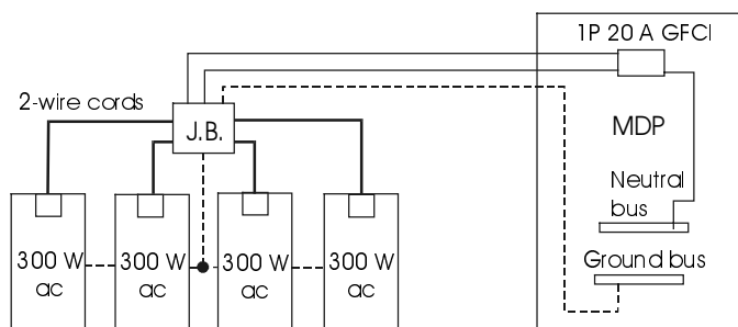
Figure 8.8 Residential rooftop system with ac modules.
