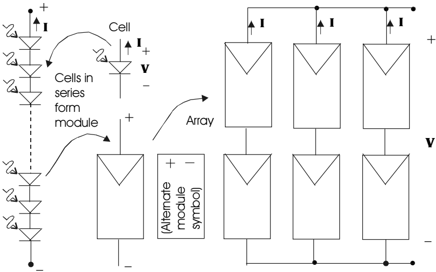
Figure 3.1 Cells, modules and arrays.
