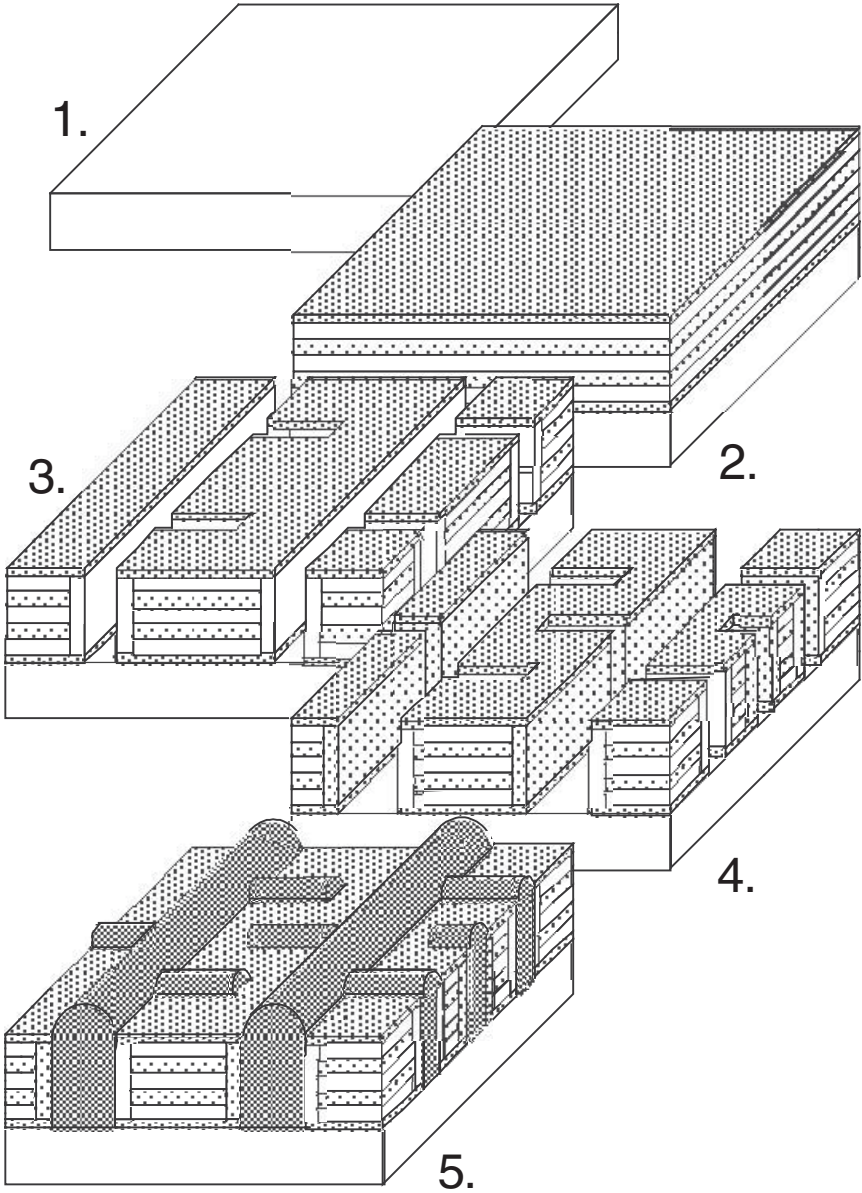
Figure 11.6 Processing sequence for buried contact thin Si cell. (Courtesy of M. Green.)
