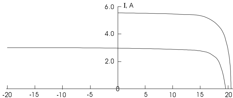
Figure P3.1 I-V characteristics of two modules, one shaded and one fully illuminated.
