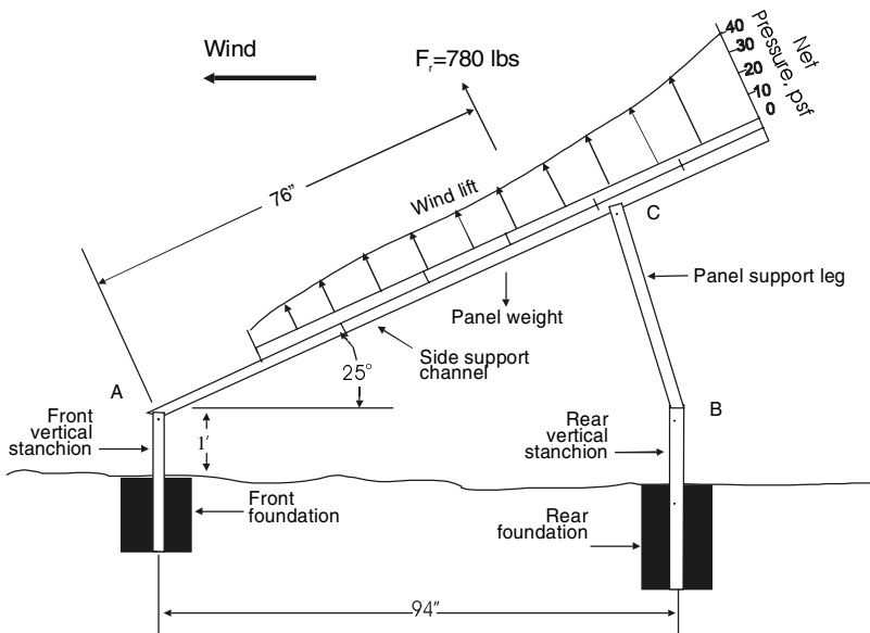
Figure 6.12 Net pressure distribution due to 100-mph winds toward the back of the array. Structural member BC is in tension.
