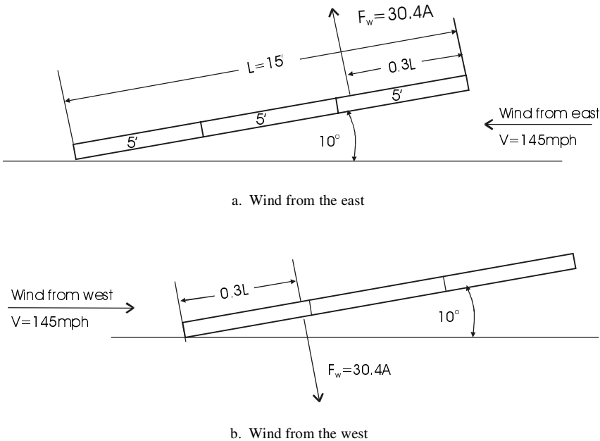
Figure 8.16 Resultant forces and their centers of pressure for winds from the east and winds from the west.
