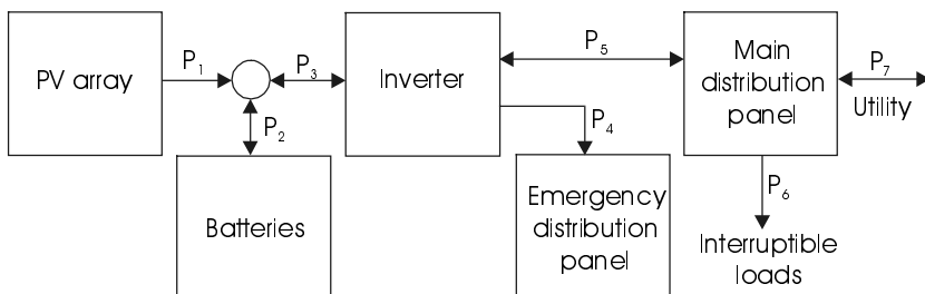
Figure 8.9 Possible power flow directions in utility interactive PV system with battery backup.
