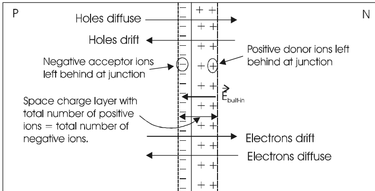
Figure 10.7 The pn junction showing electron and hole drift and diffusion.
