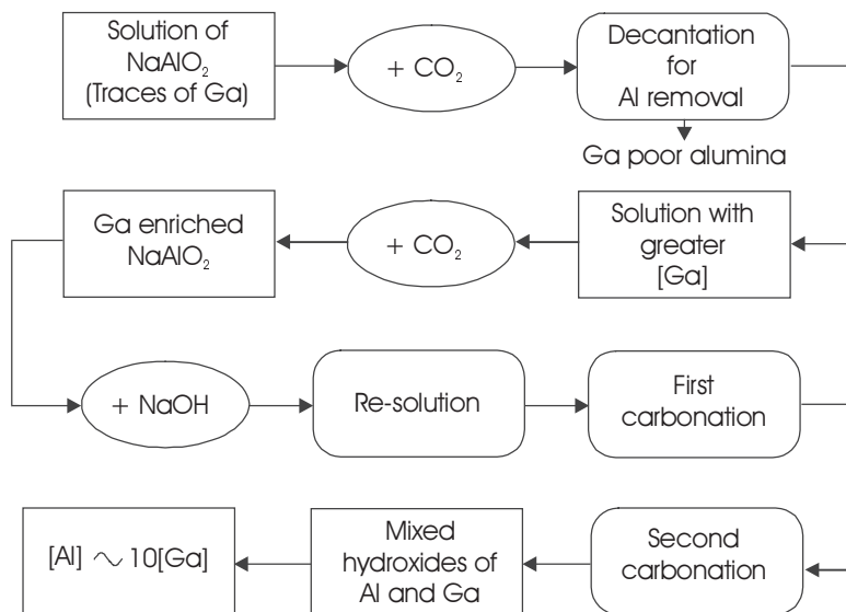
Figure 11.10 The Beja process (Pechiney) for the manufacture of gallium [20]. (Adapted from Kirk-Othmer Encyclopedia of Chemical Technology , 2nd Ed. © 1968 John Wiley & Sons, Inc. Adapted by permission of John Wiley & Sons, Inc.)
