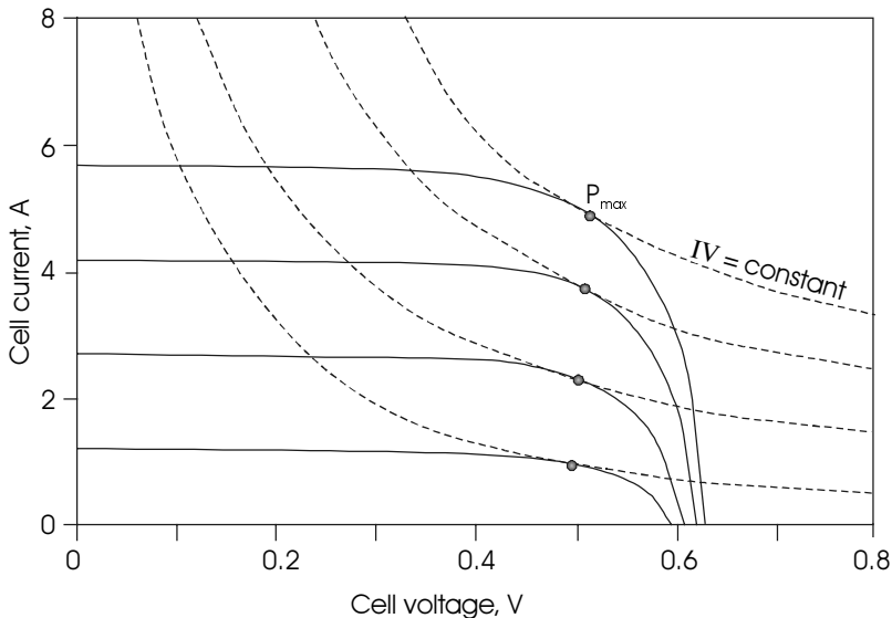
Figure 3.4 Determination of the maximum power point on a PV cell operating characteristic.
