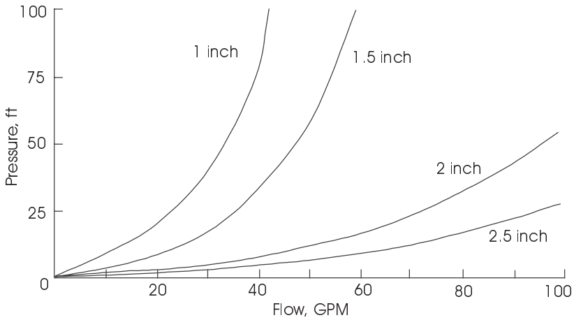
Figure 4.4 Pressure vs. flow curves for equal lengths of piping of different diameters.
