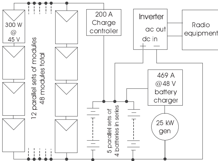
Figure 4.9 Hybrid radio repeater system. Disconnects, fusing and grounding not shown.
