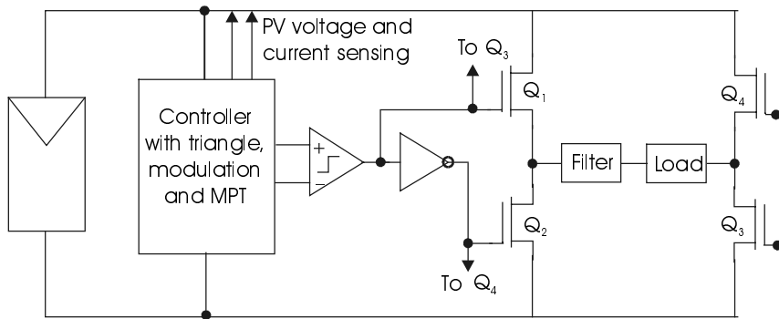
Figure 3.35 Full-bridge PWM converter showing controller and PV connections.
