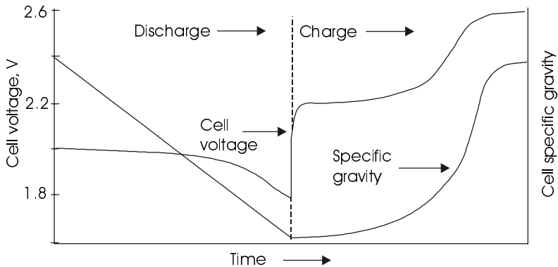
Figure 3.14 Variation of cell electrolyte specific gravity and cell voltage during charge and discharge at constant rate [1].
