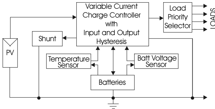
Figure 3.26 Block diagram of a fancy charge controller.
