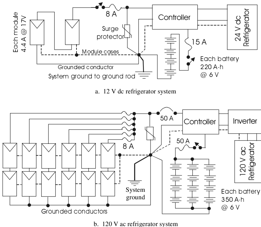
Figure 7.1 Block diagrams of dc and ac refrigerator systems.
