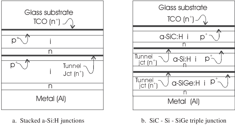
Figure 11.8 Stacked a-Si:H with Si only and with SiGe and SiC layers.
