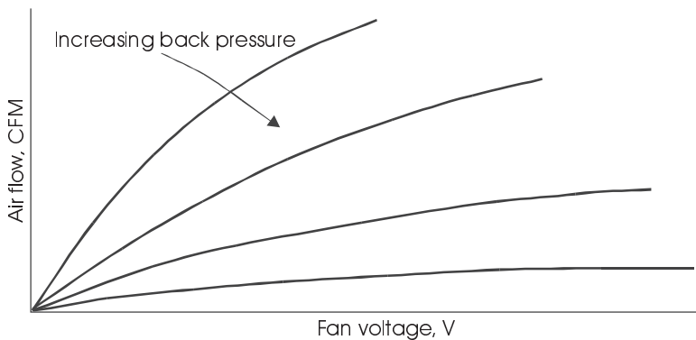
Figure 4.2 Air flow vs. fan motor voltage with pressure developed as a parameter.
