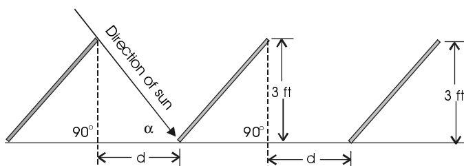
Figure P2.1 Rows of rack-mounted modules.
