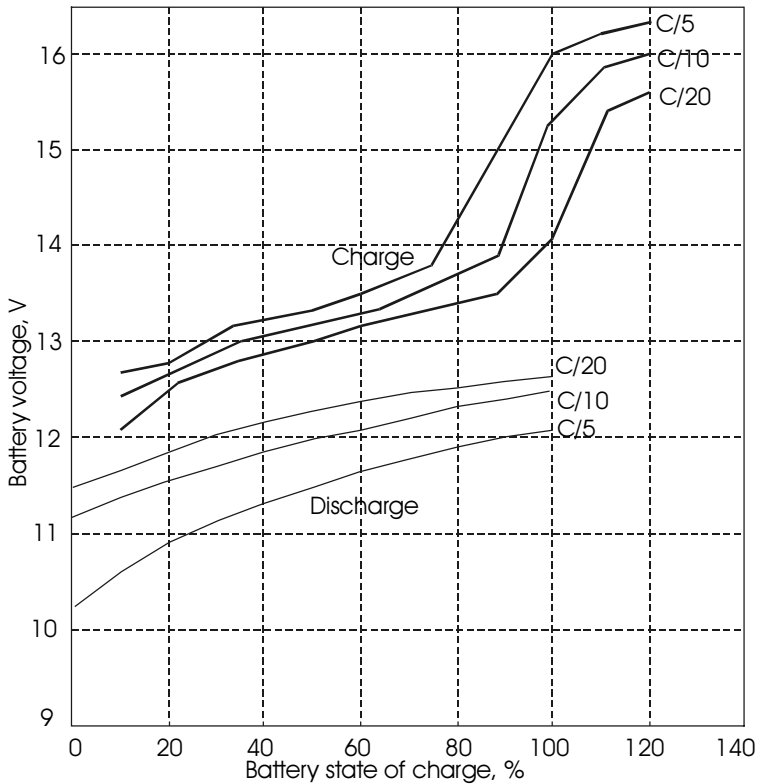
Figure 3.23 Terminal voltage as a function of charging or discharging rate and state of charge [1].
