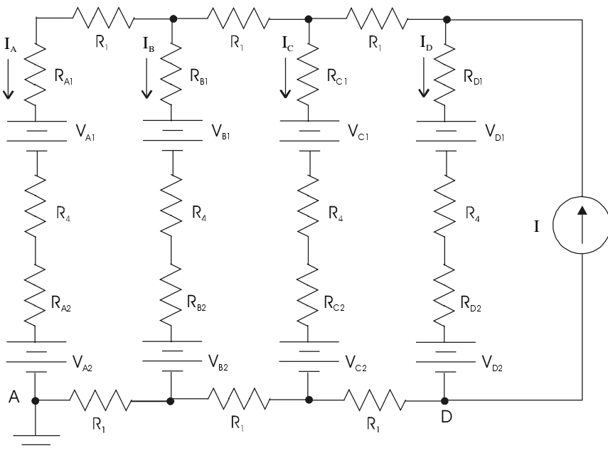
Figure 7.7 Equivalent circuit for battery connection Option 1.
