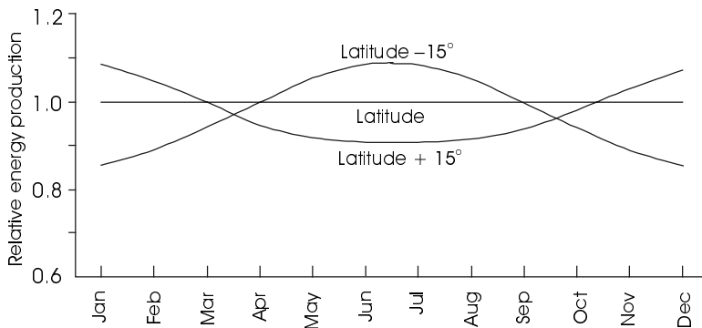
Figure 2.12 Monthly collector performance as a function of collector tilt angle.
