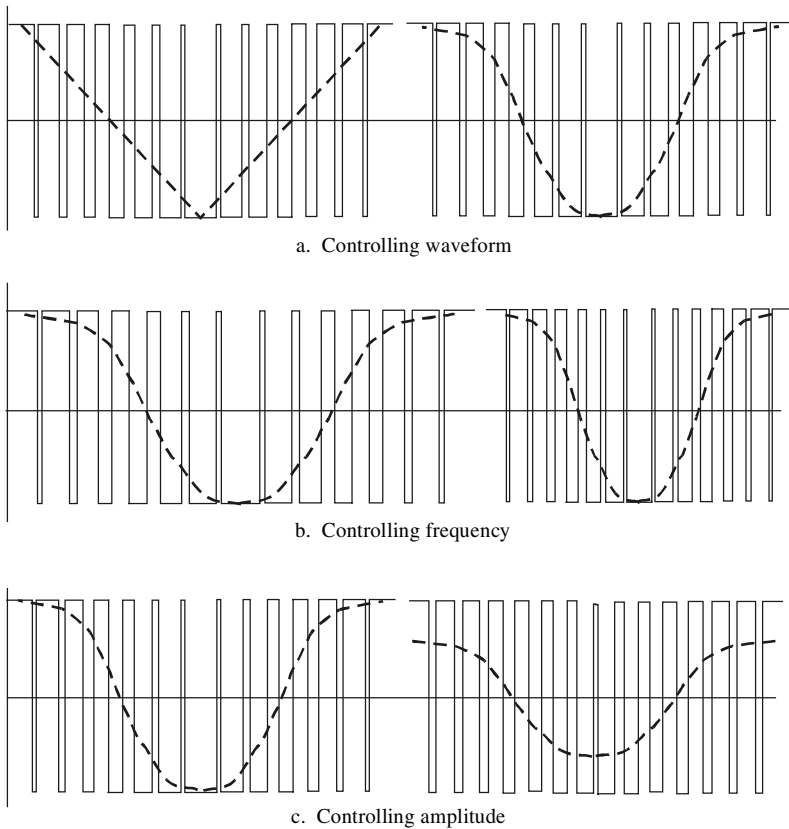
Figure 3.32 PWM control of waveform, frequency and amplitude.
