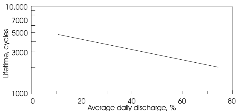
Figure 3.13 Lead-acid battery lifetime in cycles vs. depth of discharge per cycle [1].
