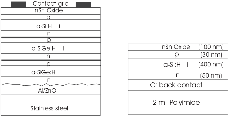
Figure 11.9 a-Si:H cell on stainless steel and polymer substrates [16, 17]. (Adapted from Guha et al., 607, and Huang et al., 699, Proc. 26th IEEE PV Spec. Conf. , 1997, ©1997 IEEE.)
