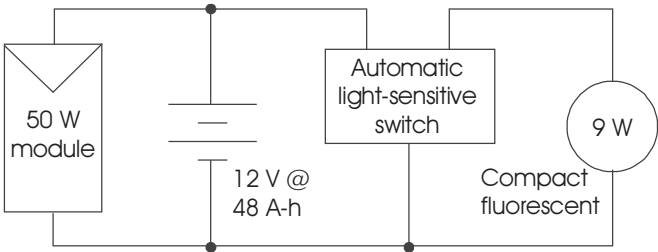
Figure 4.7 PV outdoor walkway lighting system.
