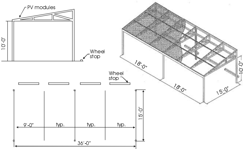
Figure 8.20 Sketch of a section of a covered parking canopy showing a typical configuration for four spaces.
