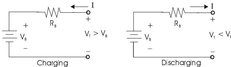
Figure 3.22 Thevenin equivalent circuit for a battery under charging and discharging conditions.
