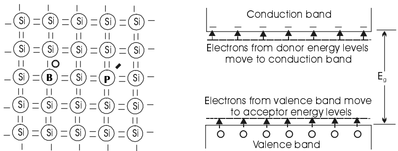
Figure 10.5 Acceptor and donor impurities in Si.
