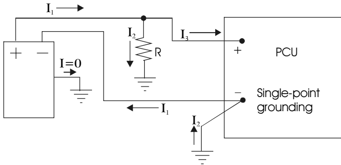
Figure 8.3 Example of ground fault.
