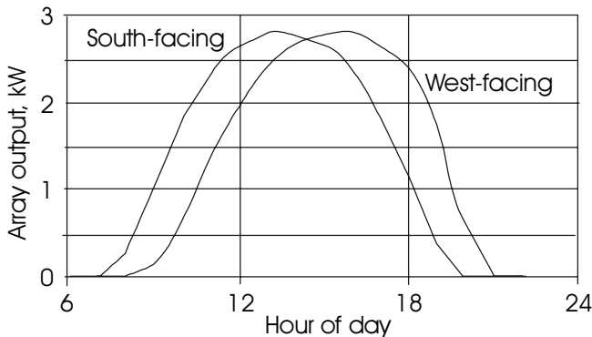
Figure 2.14 Comparison of power and energy output for south-facing and west-facing PV systems in Sacramento, CA, in summer. The south-facing system produced 22,417 Wh and the west-facing system produced 22,192 Wh. (Courtesy of Collier [4]).
