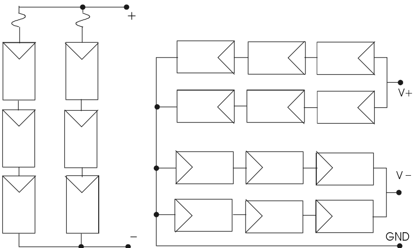
b. Series-Parallel with center grounded to provide + and - supplies (fuses and diodes not shown)
