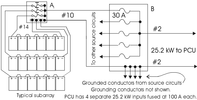
Figure 8.15 Grouping, sizing and fusing of string, source and output conductors for 20-parking-space canopies.
