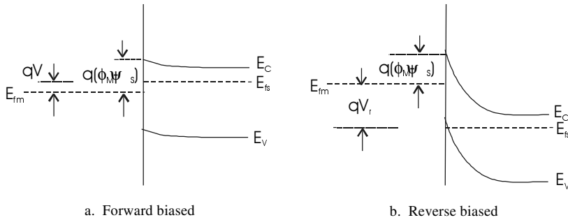
Figure 10.18 The rectifying metal-n-type semiconductor junction under forward biased and reverse biased conditions.
