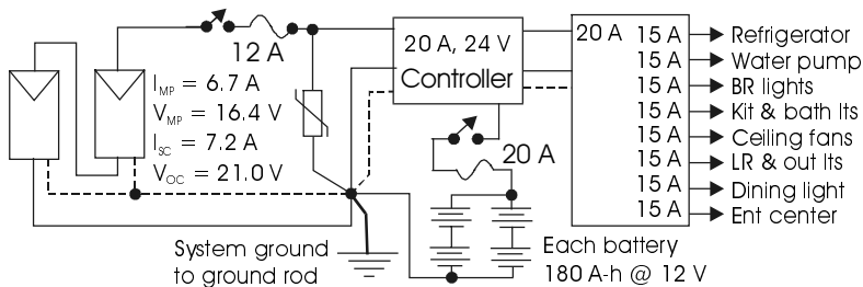
Figure 7.3 Cabin electrical system schematic wiring diagram.
