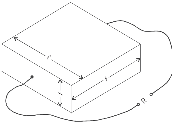
Figure 11.4 Determination of resistance per square.
