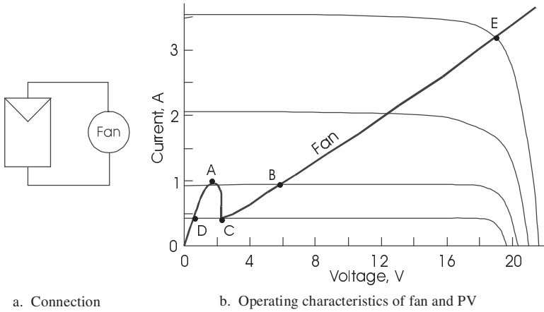
Figure 4.1 A simple PV-powered fan, showing performance characteristics for fan and PV module.
