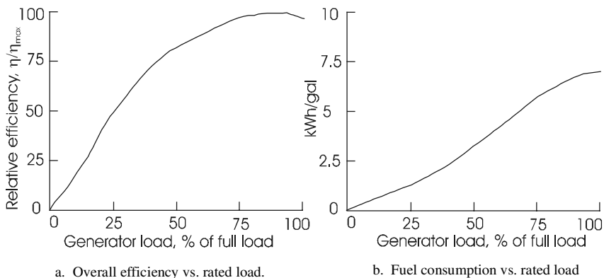
Figure 3.36 Two means of characterizing generator efficiency.
