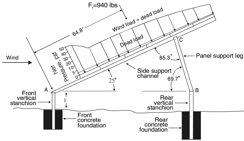
Figure 6.11 Net pressure on the array due to 100-mph winds toward the front of the array. Structural member BC is in compression.
