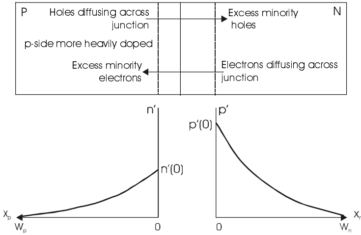
Figure 10.10 Excess minority carrier concentrations in neutral regions of pn junction device.
