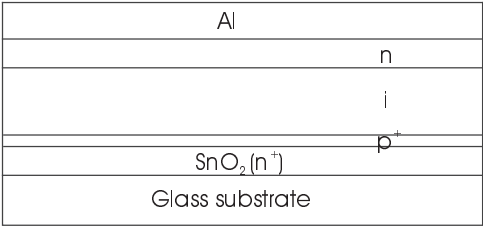
Figure 11.7 Basic a-Si:H cell structure.
