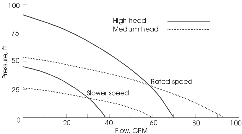
Figure 4.5 High head and medium head pump performance characteristics at two operating speeds.
