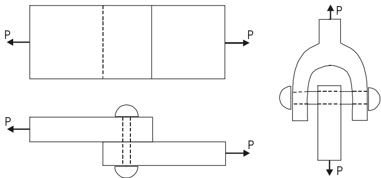
Figure 6.4 Two examples of shear loading.
