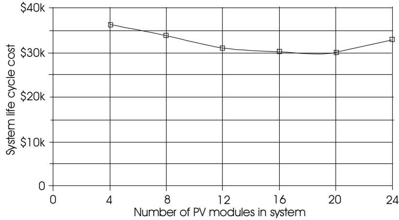
Figure 7.4a Hybrid system LCC vs. number of PV modules in system.
