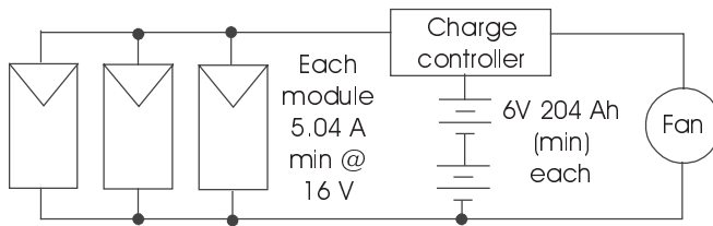
Figure 4.3 PV fan with battery storage.
