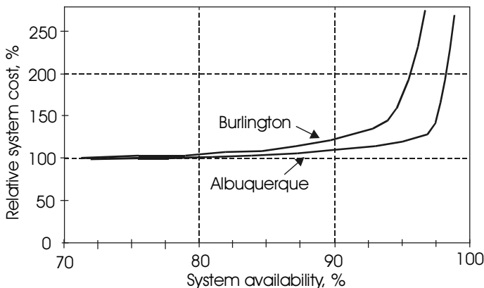
Figure 3.21 Relative cost vs. availability for PV systems in Burlington, VT, and Albuquerque, NM [8].
