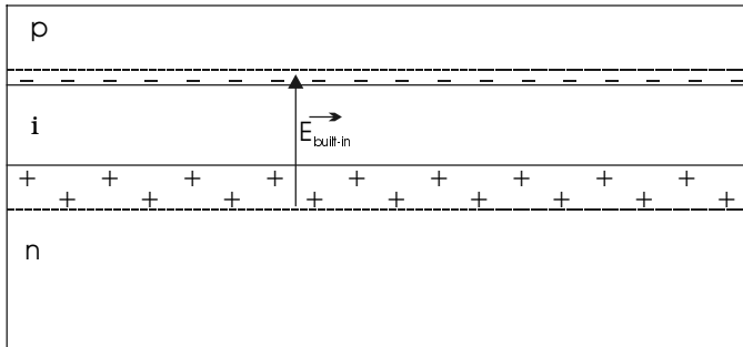
Figure 10.12 The pin junction.
