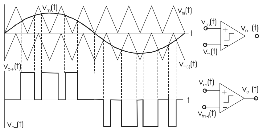
Figure 3.34 Three-level PWM inverter configuration and output signal.
