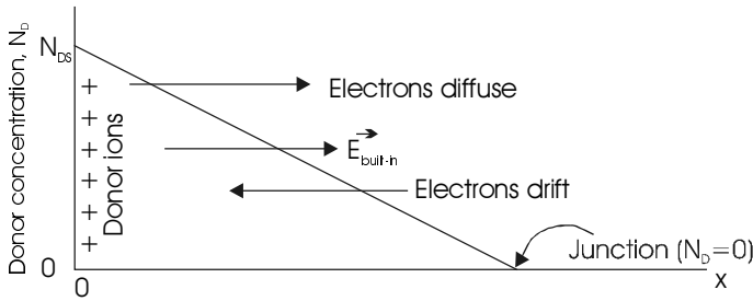
Figure 10.16 Diffusion and drift directions and electric field resulting from linearly decreasing impurity profile.
