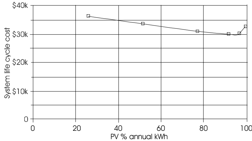
Figure 7.4b Hybrid system LCC vs. percent of annual kWh supplied by PV array.
