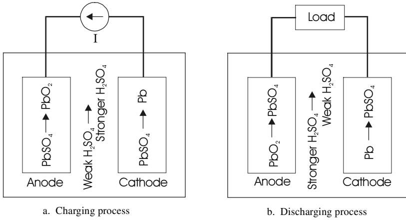
Figure 3.10 Charge and discharge of the lead-acid cell.
