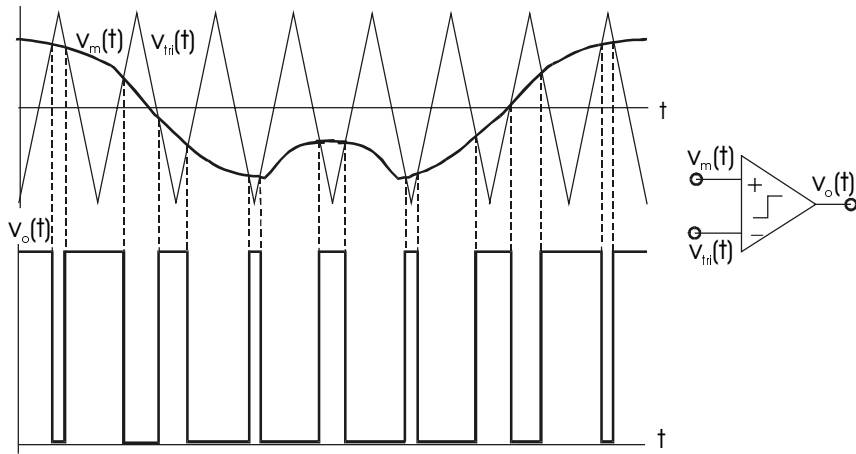
Figure 3.33 Generation of a PWM waveform.
