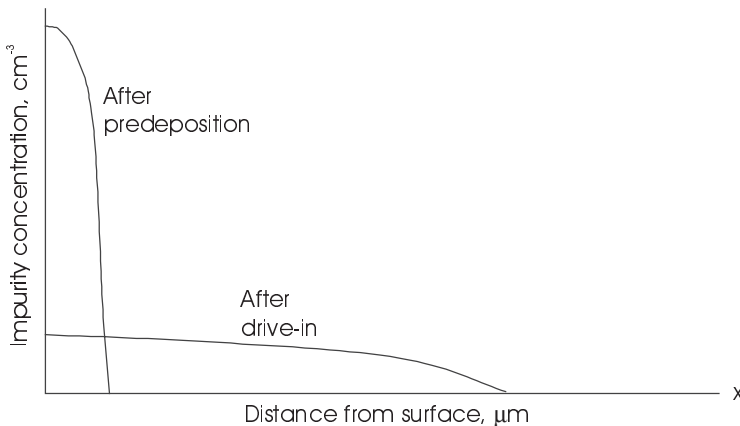
Figure 11.3 Concentrations of impurities after two diffusion steps.
