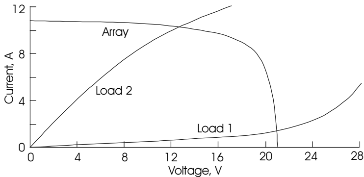
Figure P3.2 I-V characteristic for PV array and 2 loads.
