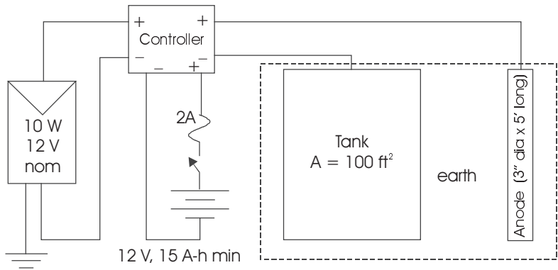
Figure 4.13 Cathodic protection system.
