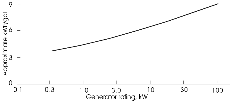
Figure 3.37 Approximate efficiency vs. generator size at rated output.
