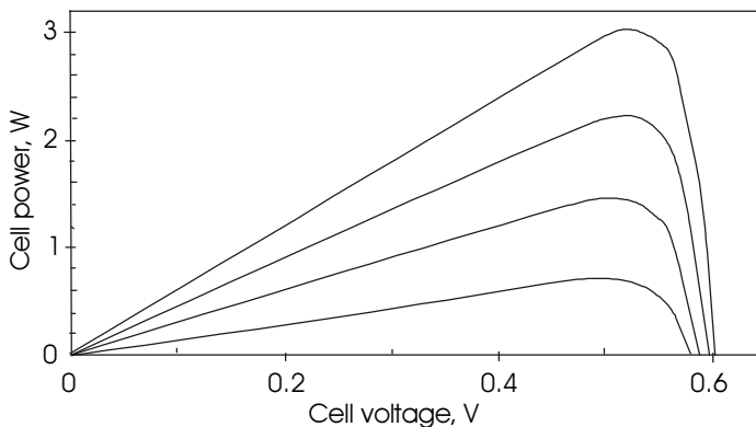
Figure 3.5 Power vs. voltage for a PV cell for 4 illumination levels.
