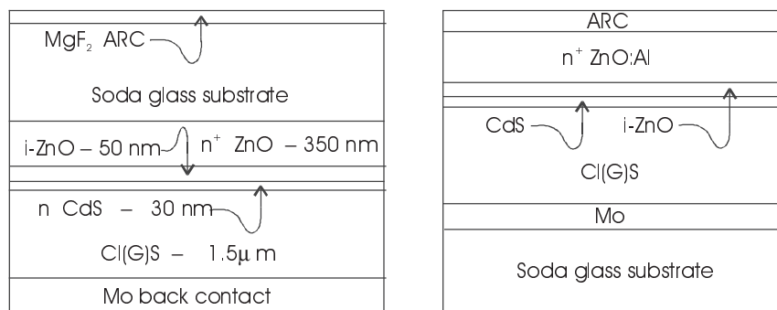
Figure 11.13 Typical CIGS thin-film structures [35, 36]. (Adapted from Ullal et al., Proc 36th IEEE PV Spec Conf , 1997, 301, ©IEEE.)
