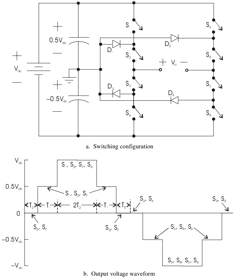
Figure 3.31 Multilevel H-bridge modified sine wave inverter..
