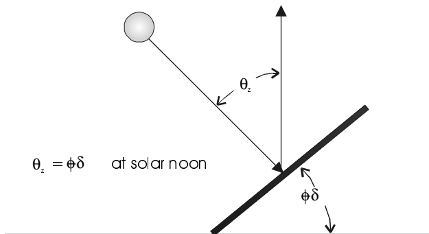
Figure 2.11 Optimizing the mounting angle of a fixed collector.
