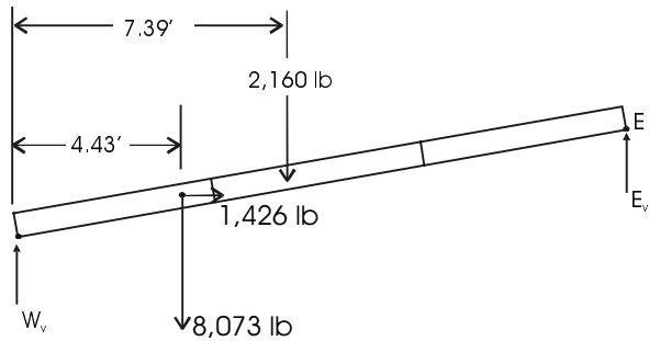
Figure 8.19 Forces acting on nine modules covering two parking spaces.
