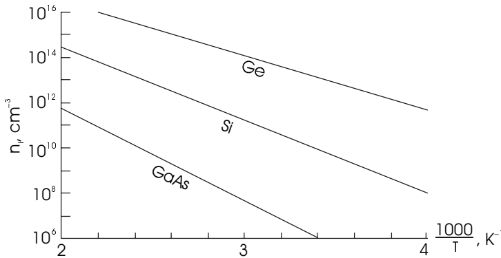
Figure 10.4 Temperature dependence of intrinsic carrier concentration for several common semiconductors [2]. (Adapted from Streetman, B., Solid State Electronic Devices , 4th Ed., 1995, Prentice-Hall. Reproduced with permission.)
