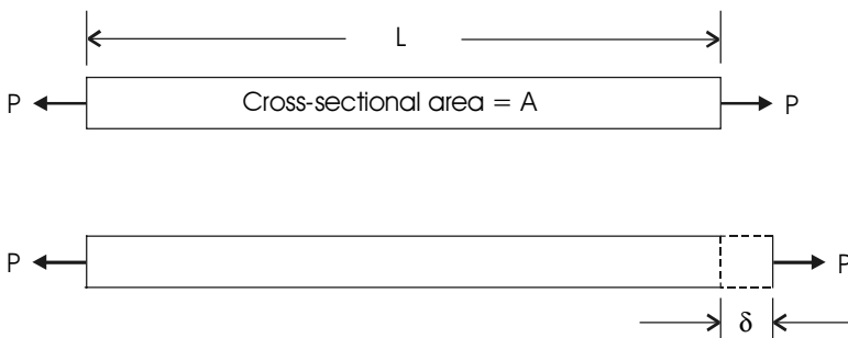
Figure 6.2 Simple pull test of a bar showing the resulting elongation.
