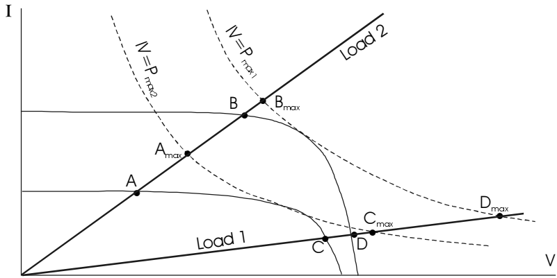
Figure 3.16 Operation of the MPT.
