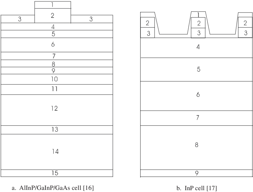
Figure 11.12 Cascaded AlInP/GaInP/GaAs cell and InP cell. Properties of the regions of the cells are summarized in Table 11.1. (Adapted from Lammasniemi, et al., 823, and Hoffman, et al., 815, Proc 26th IEEE PV Spec Conf , 1997. © 1997 IEEE.)
