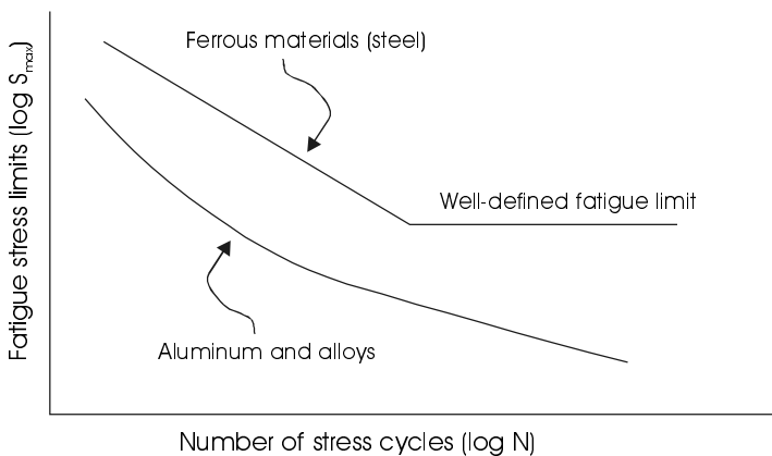
Figure 6.1 Fatigue stress vs. cycles showing a well-defined fatigue limit for ferrous metals [2].
