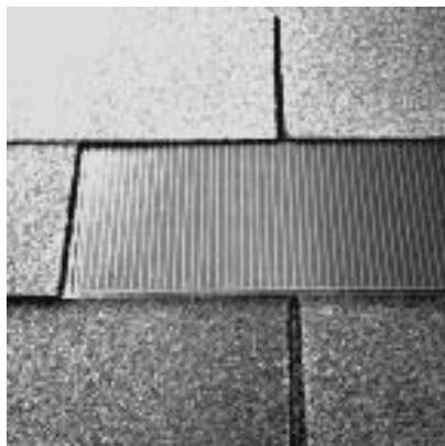
Figure 6.18 The solar shingle is installed directly on the roofing underlayment, with no air circulation below the PV laminate. It is one of a variety of new products that replaces conventional roofing materials.
