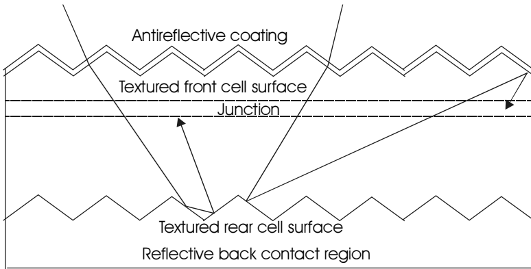
Figure 10.14 Maximizing photon capture with textured surfaces.
