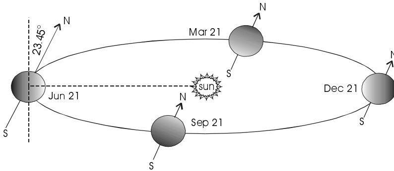
Figure 2.3 The orbit of the earth and the declination at different times of the year.
