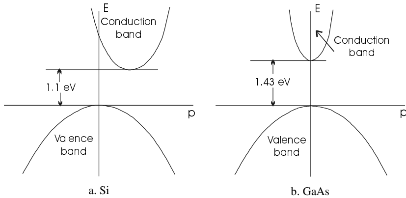
Figure 10.2 The energy and momentum diagram for valence and conduction bands in Si and GaAs.
