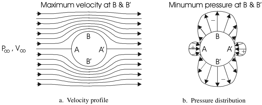
Figure 6.6 Idealized flow of air over a cylinder and the corresponding pressure distribution [10].
