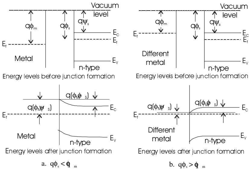
Figure 10.17 Energy levels in metal semiconductor junctions.
