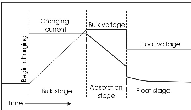
Figure 3.25 Three-stage battery charge control.
