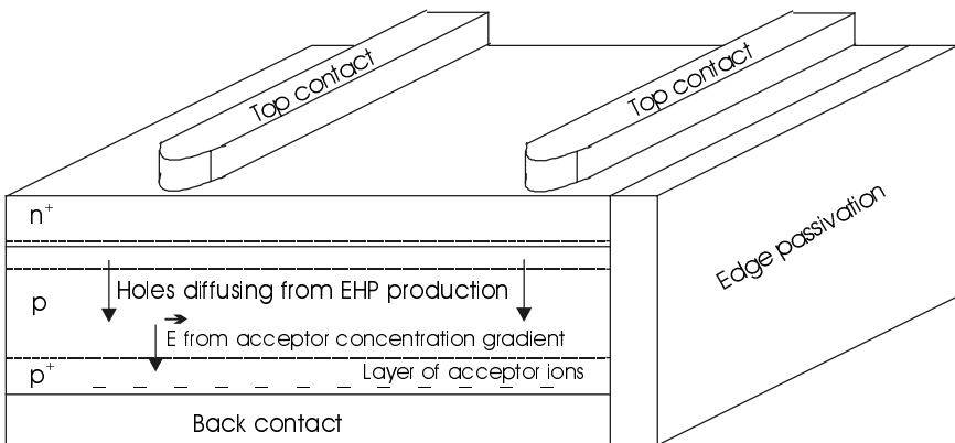
Figure 10.15 PV cell geometry for minimizing losses from cell series and shunt resistance..
