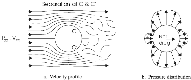
Figure 6.7 Actual air flow over a cylinder and pressure distribution, showing separation at C and C' [10].
