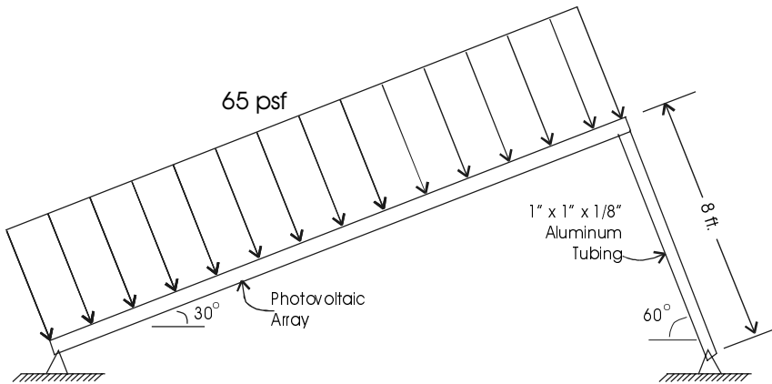
Figure 6.22 Rack-mounted array with rear support column in compression.
