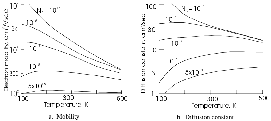
Figure 10.11 Temperature and impurity dependence of electron mobility and diffusion constant in silicon.
