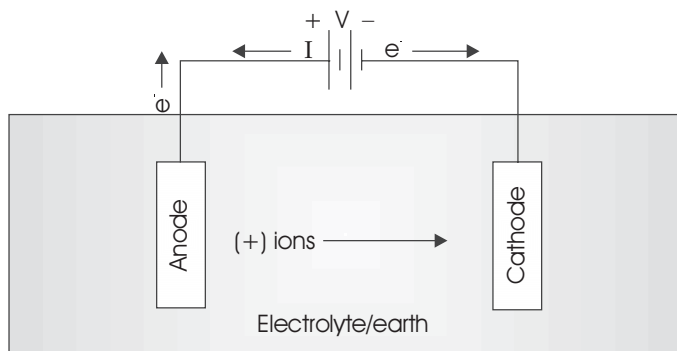
Figure 4.12 Schematic diagram of flow of current and charge carriers in an electrolyte system.
