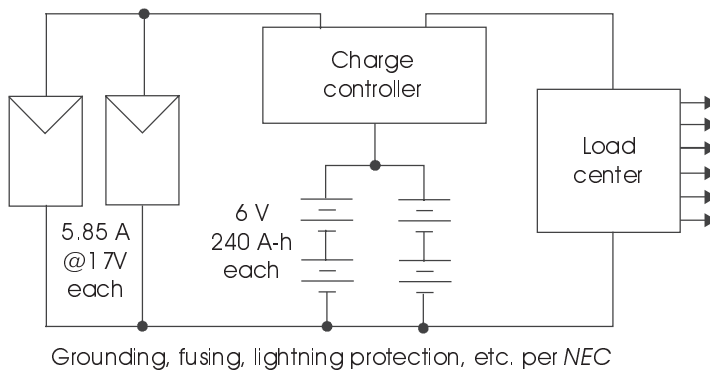
Figure 4.8 PV-powered remote cabin.
