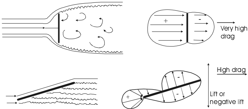
Figure 6.9 Flow over flat plates at different angles of attack to the airflow. The flat plate on the bottom may experience either an uplift or a downward force, depending on the angle of attack.
