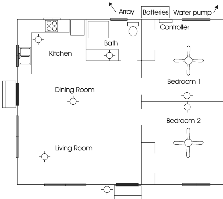
Figure 7.2 Mountain cabin floor plan and electrical layout.
