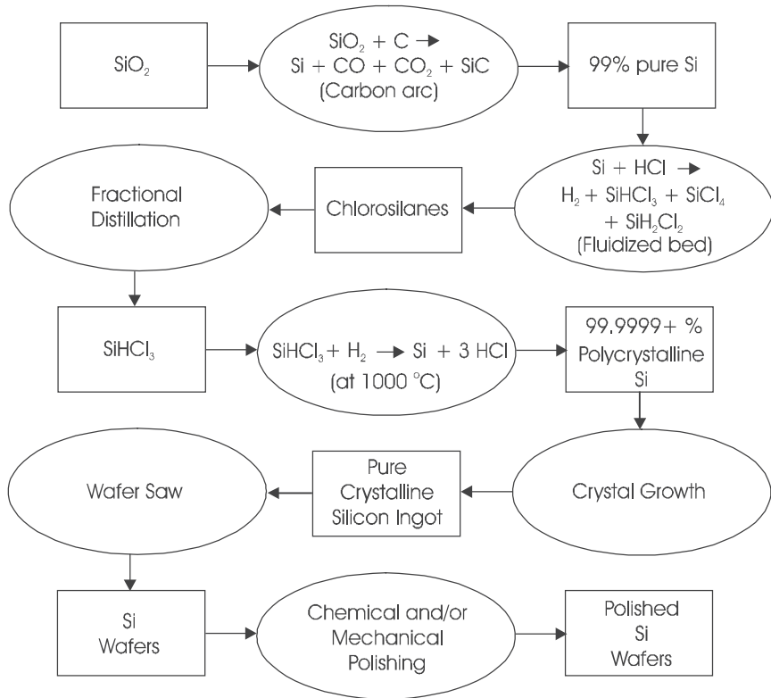
Figure 11.2 Production of single crystal silicon wafers from sand [5]. (Adapted from Ciszek, T. F., 1988, © IEEE.)
