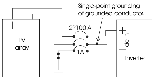
Figure 8.4 Example of ground fault detection and interruption device external to inverter.
