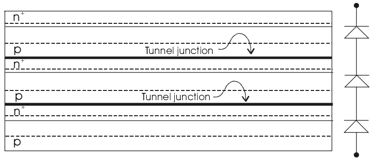
Figure 10.21 Separation of multiple pn junctions with tunnel junctions.
