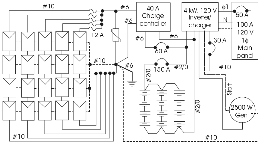
Figure 7.5 Block diagram of hybrid residence electrical system.
