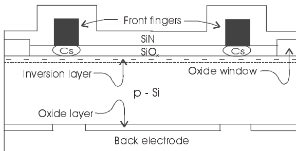
Figure 11.16 Structure of an MIS-inversion layer Si cell [47]. (Adapted from Metz, et al., Proc 26th IEEE PV Spec Conf , 1997, 31, ©1997 IEEE.)
