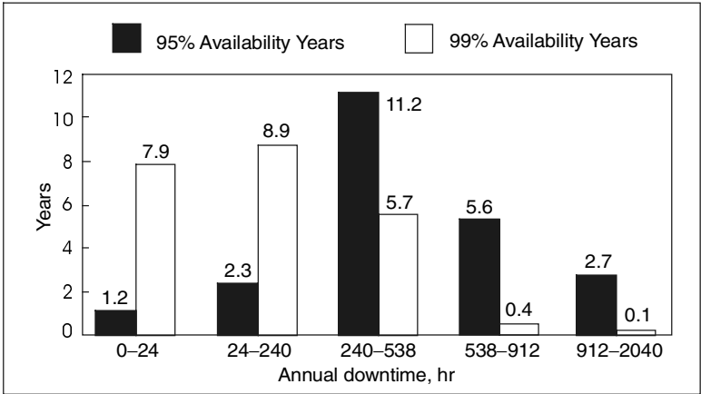
Figure 3.18 Statistical distribution of annual downtime for critical and noncritical PV systems over a 23-year system lifetime. [8]
