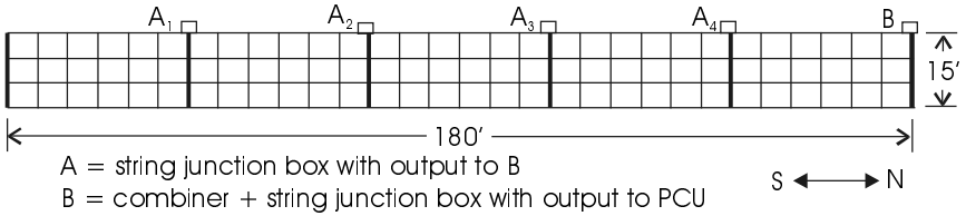
Figure 8.14 Grouping of modules in 20-parking-space canopy.
