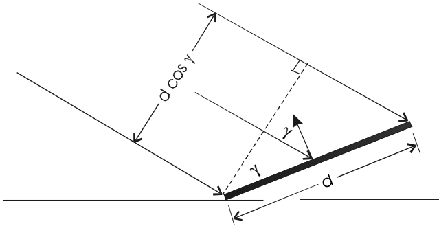
Figure 2.9 Two-dimensional illustration of effect of collector tilt on effective area presented to beam component of radiation.
