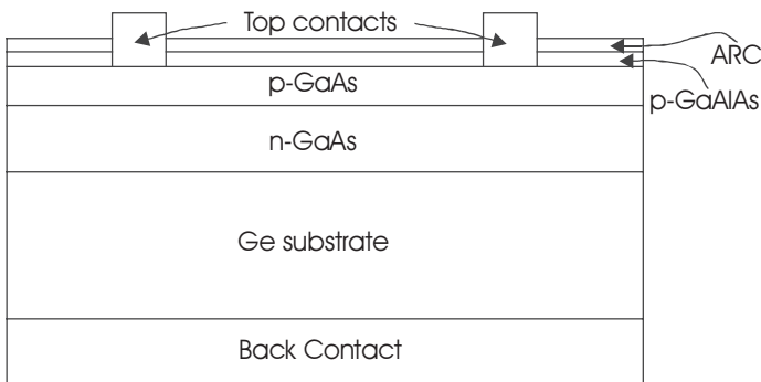
Figure 11.11 Structure of a basic GaAs cell with GaAlAs window and passive Ge substrate.
