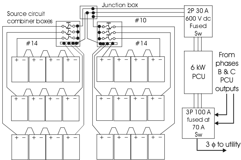
Figure 8.12 Wiring diagram for the nominal 16 kW PV system. Only phase A is shown. Phases B and C are identical to phase A and connect to the utility at the 3P 100A disconnect.
