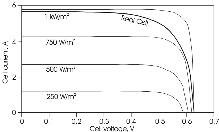
Figure 3.3 I-V characteristics of real and ideal PV cells under different illumination levels.
