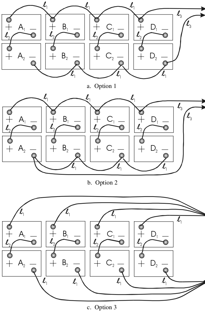
Figure 7.6 Three possible battery hookup configurations.
