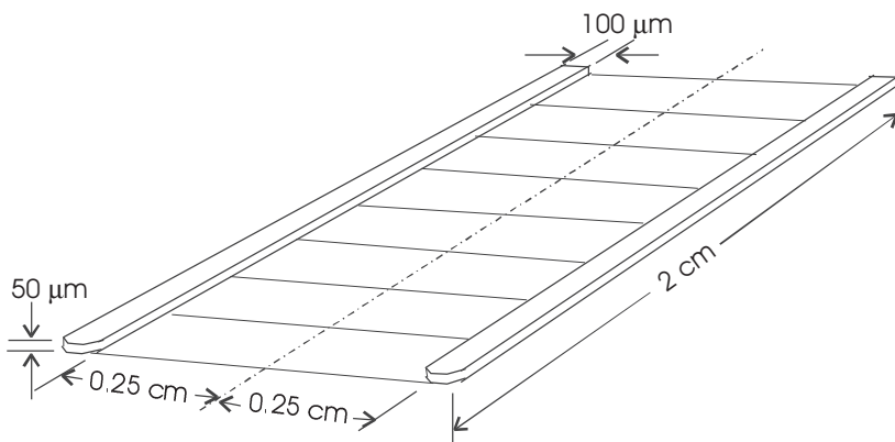
Figure 11.5 Determination of resistance between bulk and contacts.
