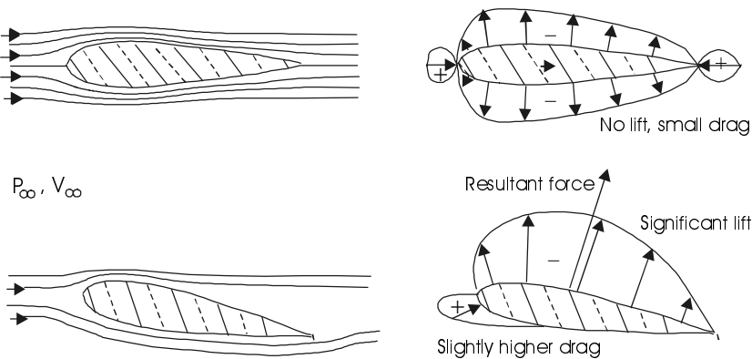
Figure 6.8 Airflow over symmetrical airfoils. The lower airfoil, which is at a positive angle of attack to the airflow, experiences significant lift [10].
