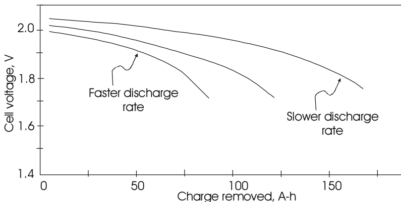
Figure 3.11 Effect of discharge rate on available energy from a lead-acid battery.
