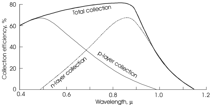
Figure 10.13 Photon collection efficiency vs. wavelength and location in cell for a typical PV cell with p-layer at the surface [1]. (Adapted from Yang, E. S., Microelectronic Devices , 1988, McGraw-Hill. Reproduced with permission of the McGraw-Hill Companies.)
