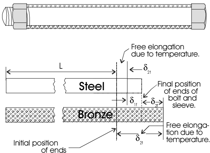
Figure 6.5 Elongations in steel and bronze due to a change in temperature.
