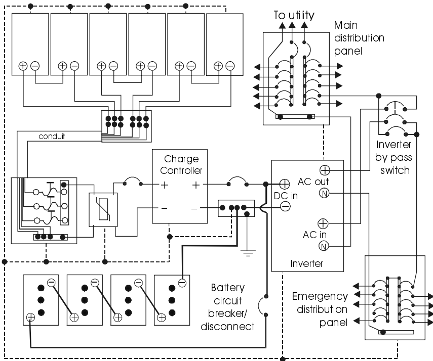
Figure P8.1 Utility interactive PV system with battery backup.
