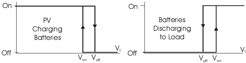
Figure 3.24 Hysteresis loops in charge controller using regenerative comparator for voltage sensing.
