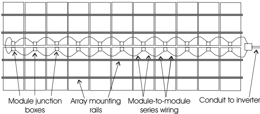
Figure 8.6 Array layout and wiring for 2.5 kW residential rooftop PV system.
