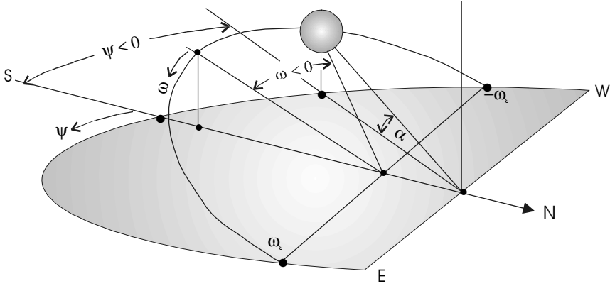
Figure 2.5 Sun angles, showing altitude, azimuth and hour angle.
