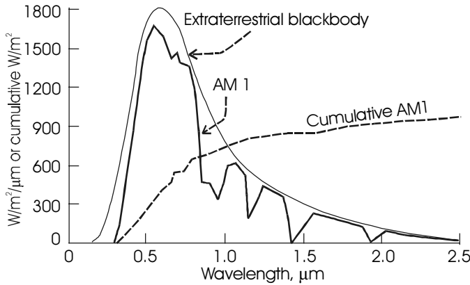
Figure 2.2 AM 1 solar spectrum after atmospheric absorption effects, including plots of extraterrestrial blackbody spectrum plus cumulative incident energy vs. wavelength.
