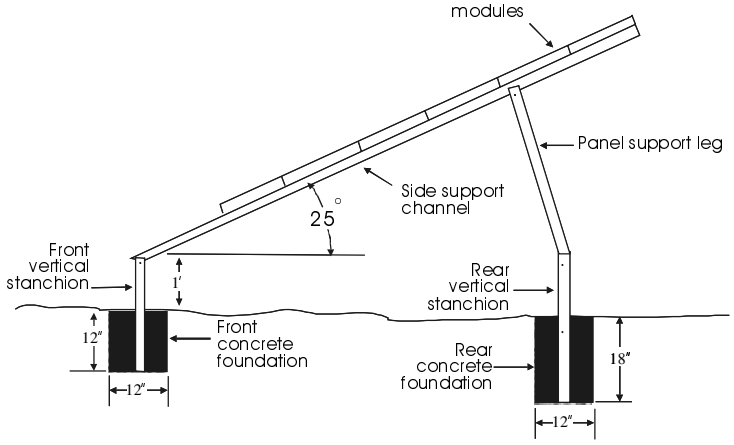
Figure 6.10 Sketch of the Hughes modular array field. This design was developed for Sandia National Laboratories [11].
