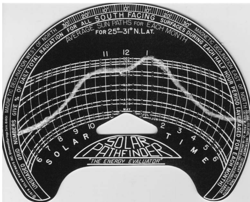
Figure 2.13 Solar Pathfinder showing region of shading. Shading occurs at points above the white line on the pattern. (Florida Solar Energy Center Photo.)
