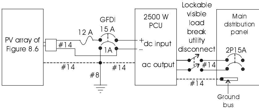
Figure 8.7 A 2 kW utility interactive residential rooftop PV system.
