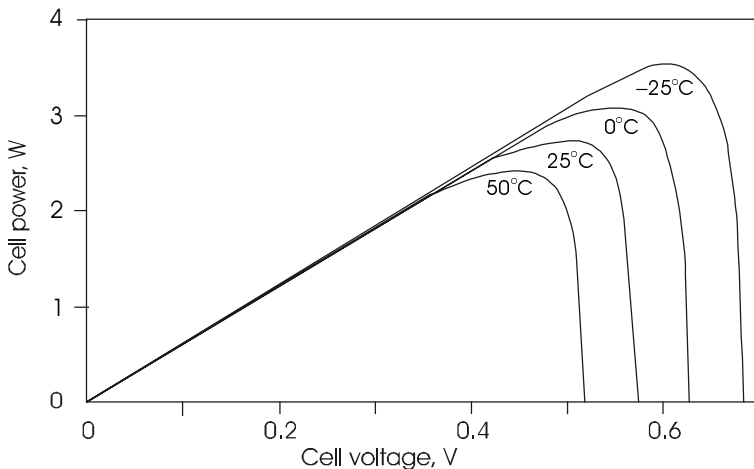
Figure 3.6 Temperature dependence of the power vs. voltage curve for a PV cell.
