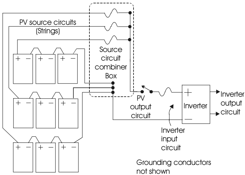
Figure 8.2 Recommended switching and fusing in PV source and output circuits.
