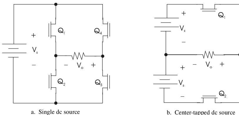
Figure 3.29 Converting dc sources to square waves.
