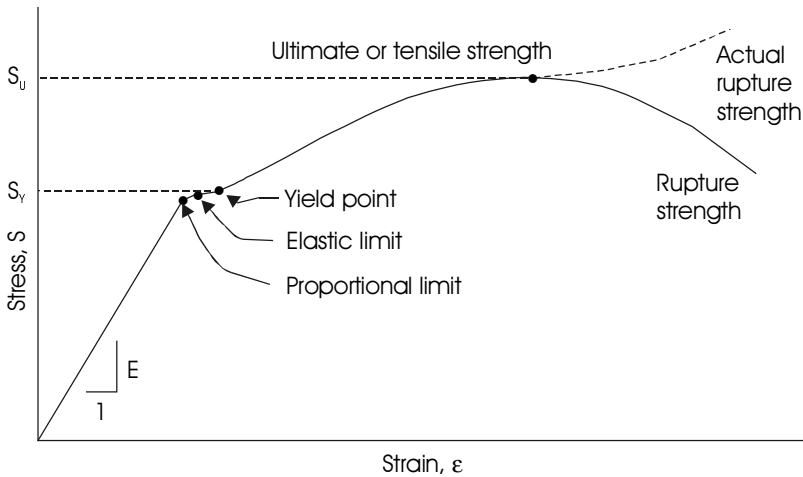
Figure 6.3 Stress-strain curve for steel.
