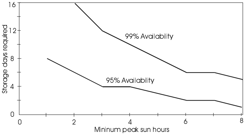
Figure 3.19 Necessary days of autonomy for critical and noncritical PV systems operation vs. minimum available peak sun hours [8].
