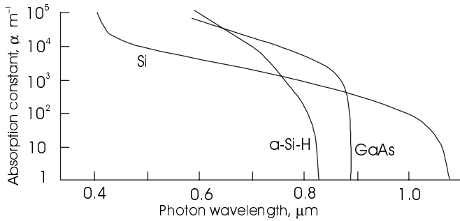
Figure 10.3 Dependence of absorption constant on wavelength for several semiconductors [1]. (Adapted from Yang, E. S., Microelectronic Devices , 1988, McGraw-Hill. Reproduced with permission of the McGraw-Hill Companies.)
