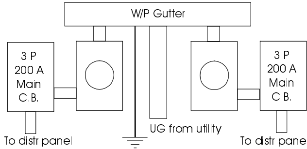
Figure 8.11 Existing electrical service diagram for 16 kW PV addition.
