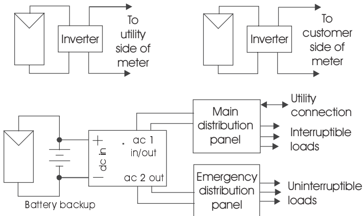
Figure 4.10 Three possible configurations for utility interactive PV systems.
