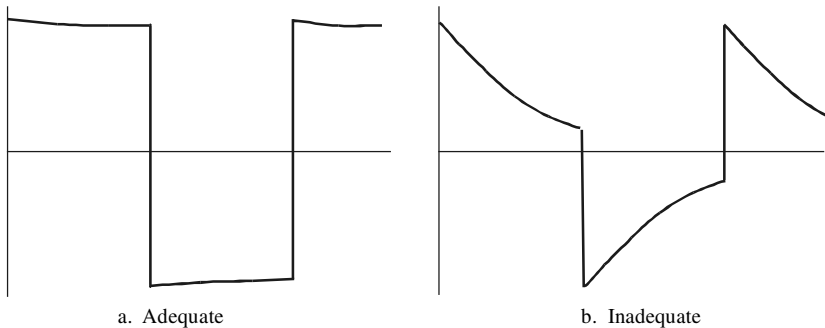
Figure 3.30 Output waveforms for square wave inverter with adequate and with inadequate number of transformer turns.
