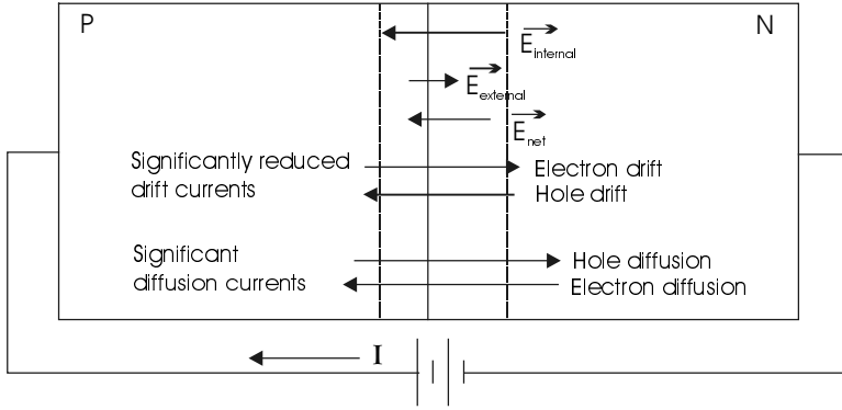
Figure 10.9 The pn junction with external bias.
