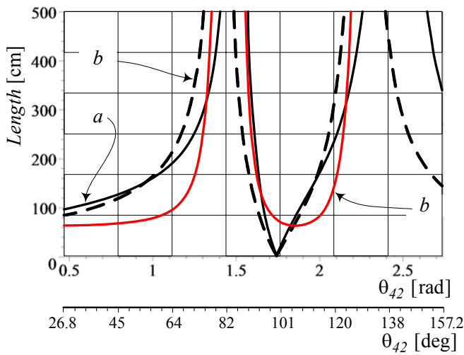
FIGURE 6.11. The length of links a , b , and c as functions of \theta_{42} .
