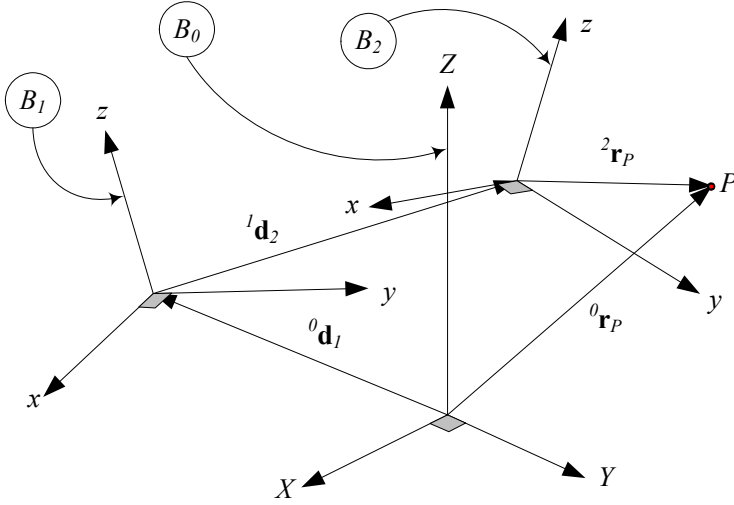
FIGURE 5.14. A rigid body coordinate frame B_2 is moving in a frame B_1 that is moving in the base coordinate frame B_0 .
