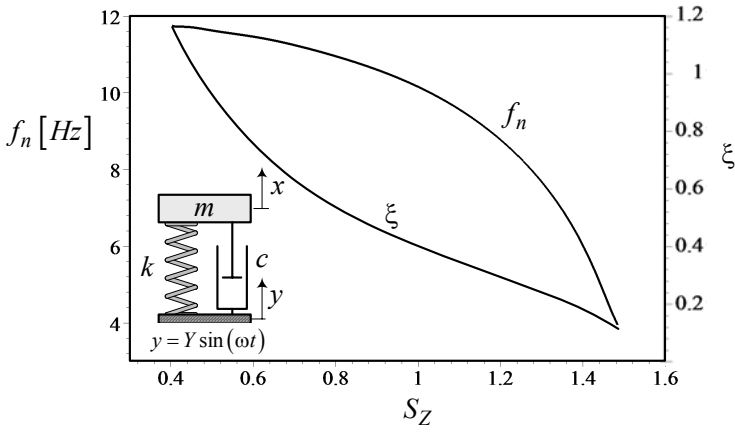
FIGURE 14.19. The optimal f_n and \xi versus S_Z .
