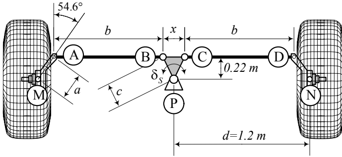
FIGURE 7.43. A multi-link steering mechanism that must be optimized by varying x .
