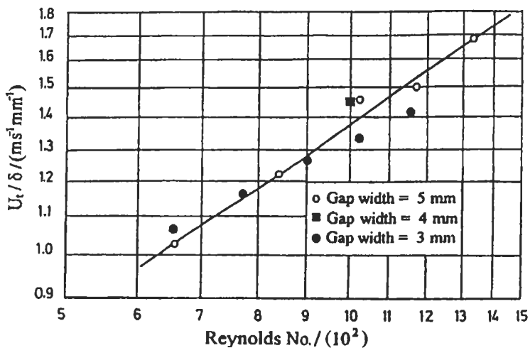
Fig. 3.72 : Variation of (U_t/\delta) with Reynolds number [531].
