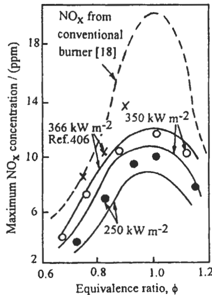
Fig. 2.94: Experimental (●, O) and predicted (full curves) [108], maximum \text{NO}_x concentration versus equivalence ratio at two firing rates. Experimental values, x, were taken from Ref. 406.
