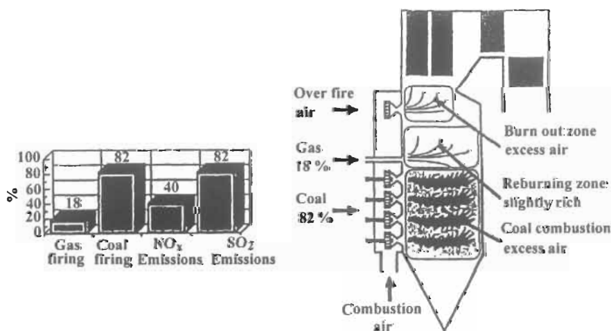
Fig. 5.95: \text{NO}_x re-burning [915]. Reproduced by permission of EPRI.
