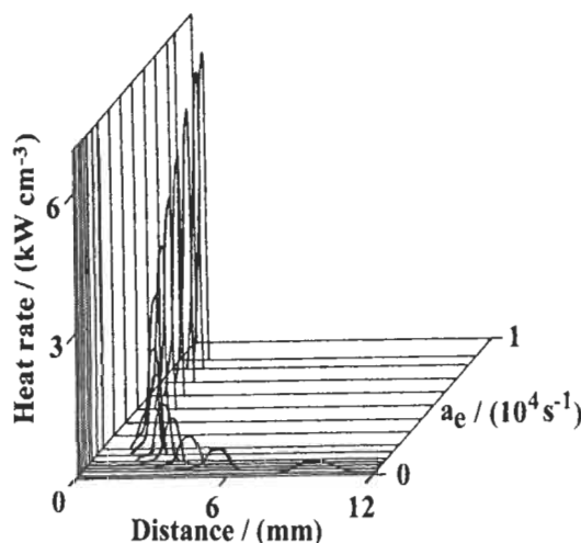
Fig. 3.8: Computed heat release profiles in counter flow diffusion flame of equimolar H_2/N_2 with air at applied stresses of 100, 300, 500, 750, 1000, 1500, 2000, 3000, 4000, 5000, 6000, 7000, 8000 and 8600 s^{-1} (extinction limit, Dixon-Lewis and Missaghi [100]) [65]. Reproduced by permission of The Combustion Institute.
