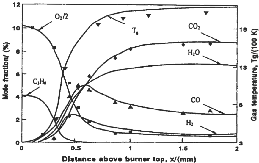
Fig. 2.45(a): Experimental species and gas temperature (■ O 2 , ▲ CO, ◆ CO 2 , and ▼ Tg). Full curves are the computed species and gas temperature for propane-air flame at P a = 1 atm., T u = 300 K and \phi = 1 [207].
