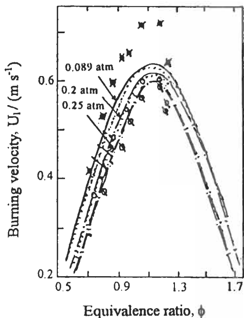
Fig. 2.32: Comparison between computed (full and dotted curves) and experimental values (ringed points \times , \circ , and \diamond at P = 0.089 , 0.2 and 0.25 atm, respectively) of laminar burning velocities for \text{CH}_3\text{OH} -air flames at different equivalence ratios and at T_u = 323 K, chain dotted curves for scheme A_1 , dotted curves for scheme B_1 ( Z = 0.4 ) and full curves for scheme C_1 [154].
