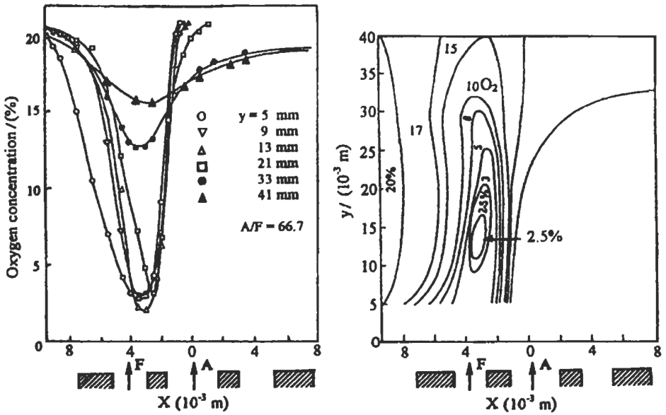
Fig. 3.98: Distribution and constant concentration contours of oxygen in the flame for single fuel jet arrangement ( A/F = 66.7 ) [576].
