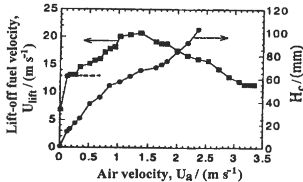
Fig. 3.31: Dependence of the critical lift-off height, H_c , on air velocity, U_a , with bluff-body diameter D_b = 45 mm. Corresponding fuel lift-off velocity U_{lift} is also plotted. Dashed line indicates lift-off velocity of pure jet flame at 13 m s -1 [496]. Reproduced by permission of Elsevier Science.
