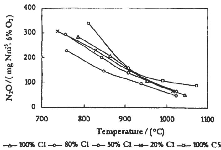
Fig. 5. 190: \text{N}_2\text{O} emissions of the different composition mixtures tested for blend \text{B}_2 versus temperature. Ibrahim Gulyurtlu et al [1149], reproduced by permission.
