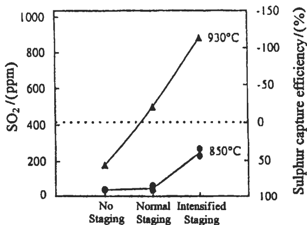
Fig. 5.196: \text{SO}_2 emission (or desulphurization efficiency \eta_s ) for three cases of air supply at 850 °C and 930 °C at a constant total excess-air ratio of 1.2 and \text{Ca/S} = 3 . Negative desulphurization efficiency means excess sulphur emission [1130]. Cited by Leckner [1047].
