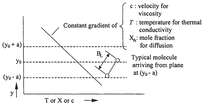
Fig. 1.13: Constant gradient assumed in the kinetic theory derivation of the transport properties, viscosity, thermal conductivity and ordinary diffusion [52]. Reproduced by permission of John Wiley and Sons Inc.
