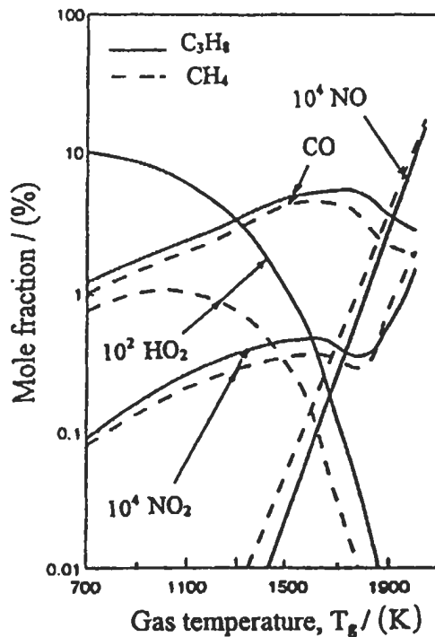
Fig. 2.82 (a): Comparison between the maximum mole fractions of \text{NO} , \text{NO}_2 , \text{CO} and \text{HO}_2 for both \text{CH}_4 -air and \text{C}_3\text{H}_8 -air flames, at \phi = 1 , 300 K and 1 atm [19].
