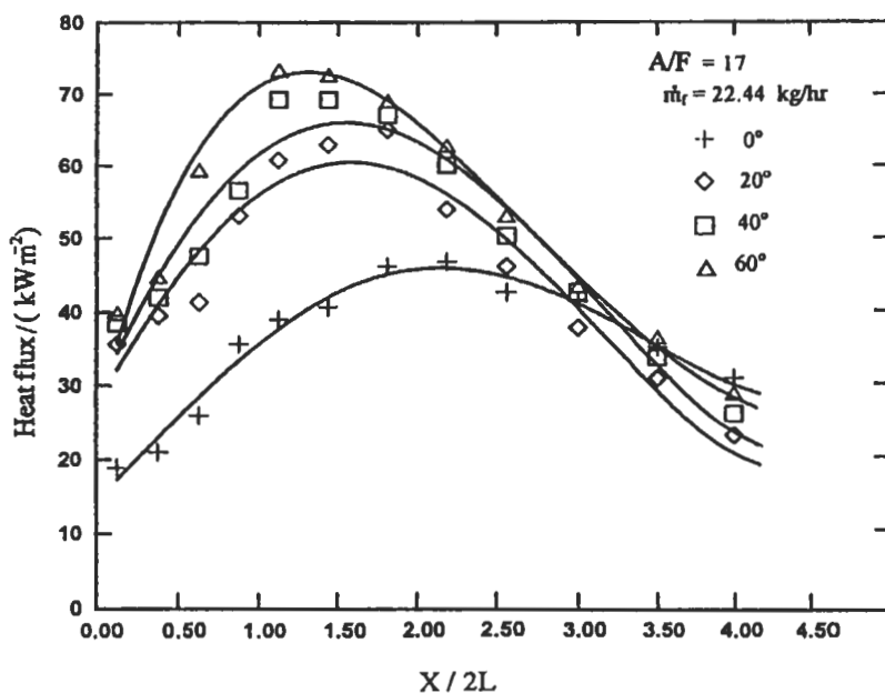
Fig. 5.41: Effect of variation of swirl angle on the distribution of the total heat transfer along the flame tube, 2L = 0.4 \text{ m} [804].
