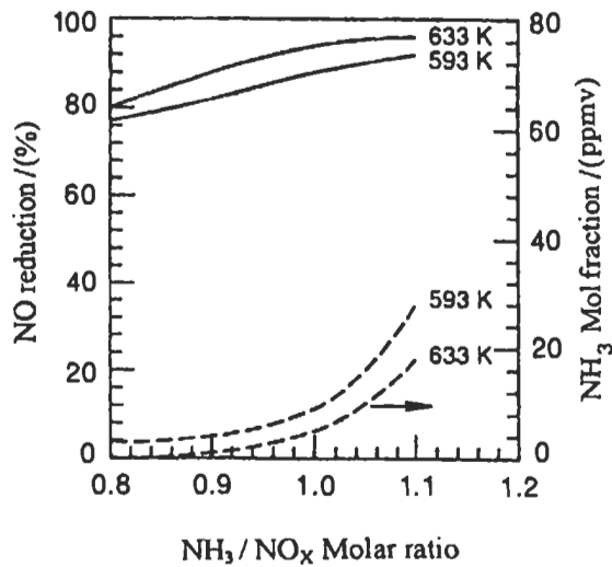
Fig. 5.90: Representative NO x -removal efficiency and NH 3 slip for the selective catalytic reduction process [118, 913]. Reproduced by permission of The Combustion Institute.
