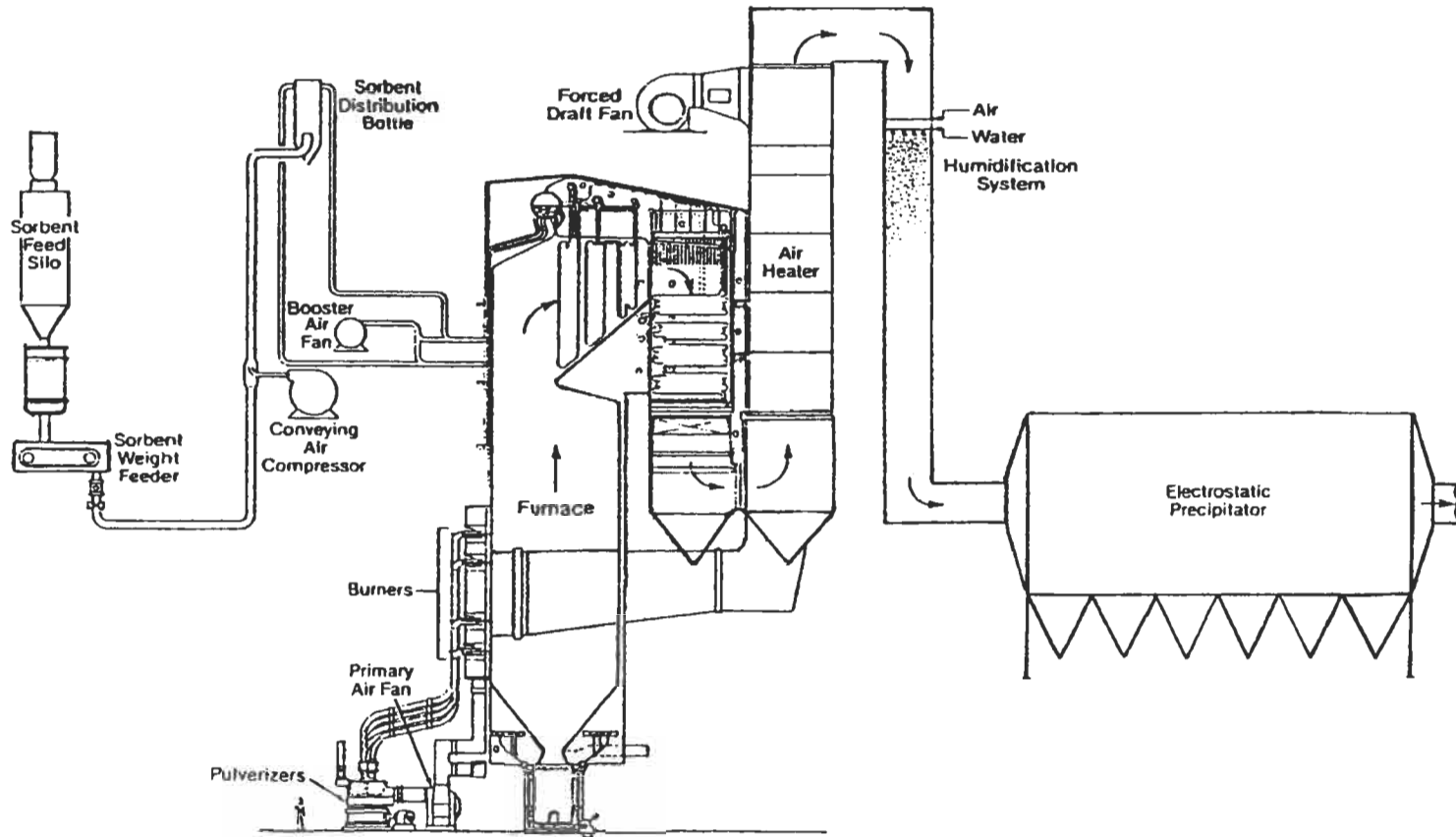
Fig. 5.94 (d): furnace sorbent injection system for \text{SO}_2 control – includes humidifier system to enhance particulate collection and \text{SO}_2 removal efficiency [126]. Reproduced by permission of the Babcock & Wilcox Company
