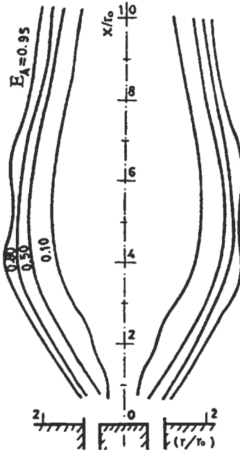
Fig. 3.54: Burned fuel contours, burner diameter ratio of 30/17, relative A/F = 0.6 [525].
