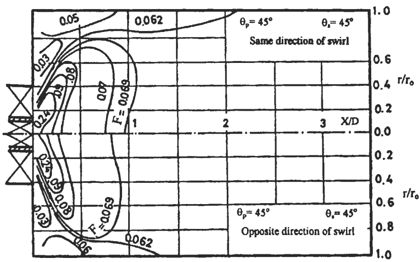
Fig. 4.28: Effect of the relative direction of swirl on the constant concentration contours ( m_s = 250 \text{ kg h}^{-1} , MR = 13.5 ) [605].
