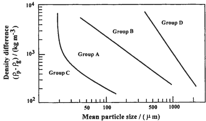
Fig. 5. 154: Powder classification diagram for fluidization by air at ambient conditions [1997]. Reproduced by permission of Taylor & Francis Books, Inc.
