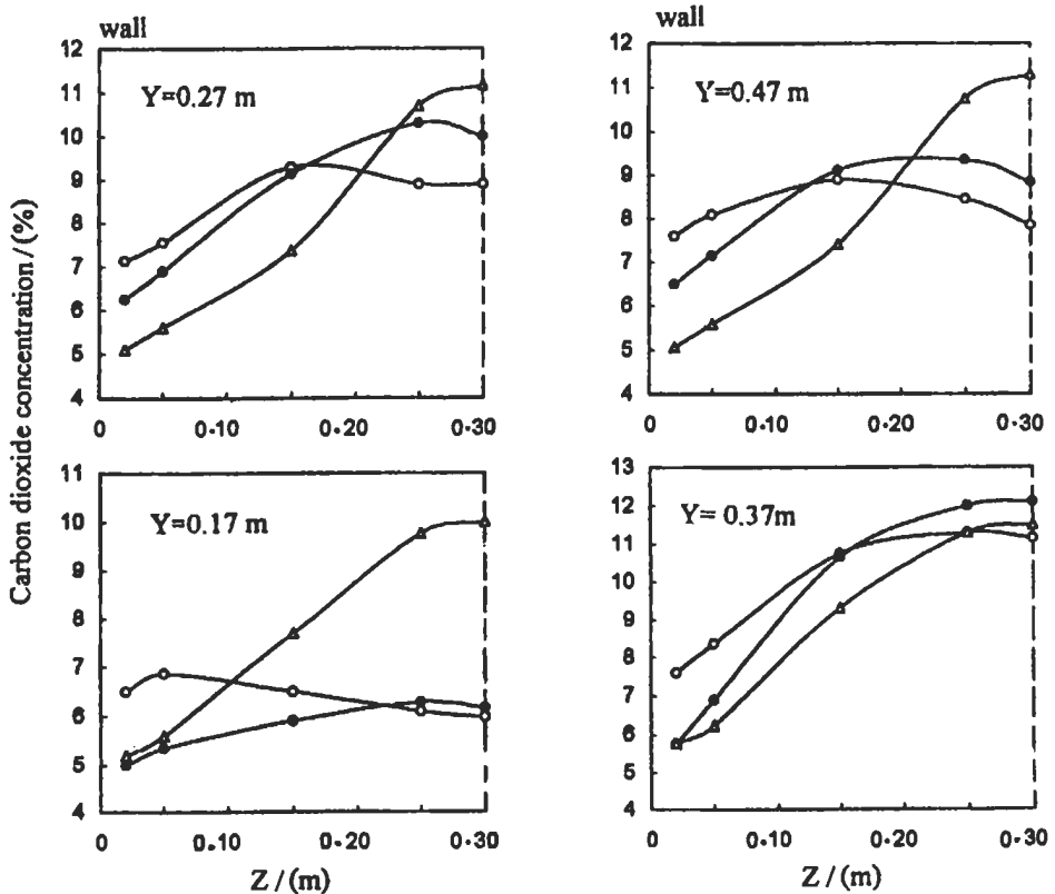
Fig. 5.117: Effect of inclination angle on the average carbon dioxide distribution at different levels of the model furnace ○ 8^\circ , ● 6^\circ , △ 0^\circ [932].
