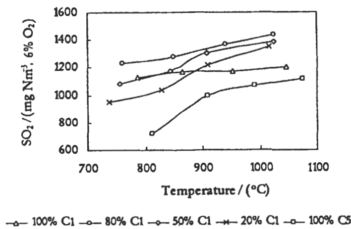
Fig. 5. 191: \text{SO}_2 emission of the different composition mixtures tested for blend \text{B}_2 versus temperature. Ibrahim Gulyurtlu et al [1149], reproduced by permission.
