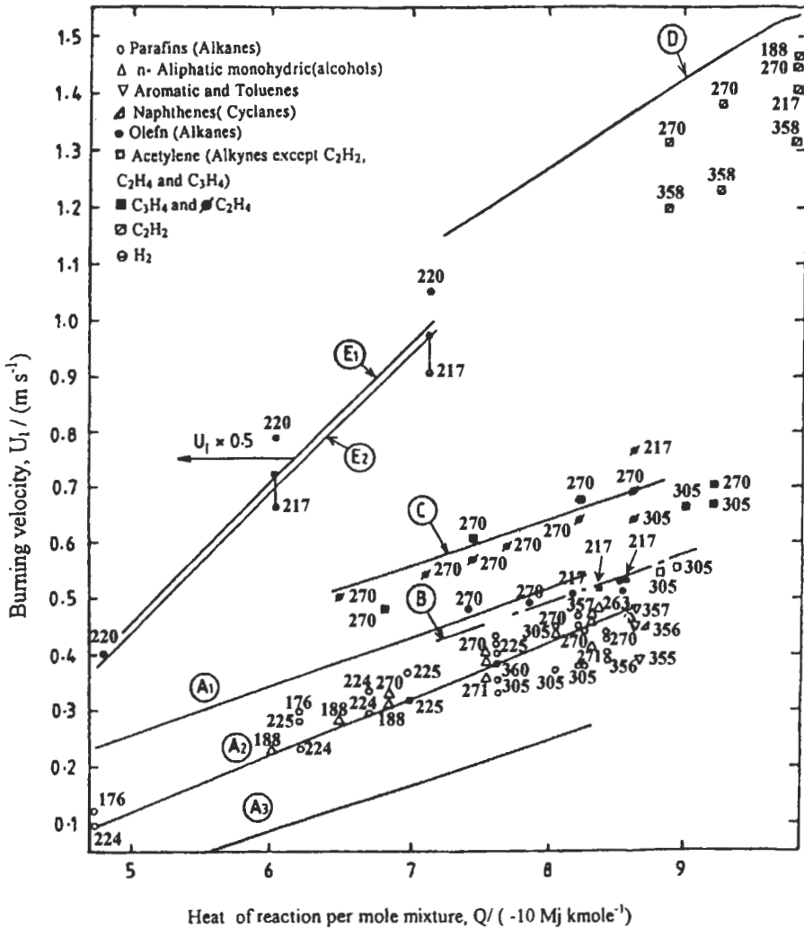
Fig. 2.67: Burning velocities of lean mixtures of different fuels at 300 K. Full lines are computed A1: CH 4 and CH 3 OH at 0.1 atm [44, 153, 154 & 156], A2: CH 4 and CH 3 OH at 1 atm [44, 153 & 156] and A3: CH 4 and CH 3 OH at 10 atm [44, 153 & 156], C: C 2 H 4 at 1 atm [537], D: C 2 H 2 at 1 atm [537], E1: H 2 at 1 atm [537], E2: H 2 at 1 atm [94, 97]. Experimental points references are given. B is through alkene experimental points at 1 atm, but not C 2 H 2 and C 2 H 4 [45]. Reproduced by permission of Elsevier Science.
