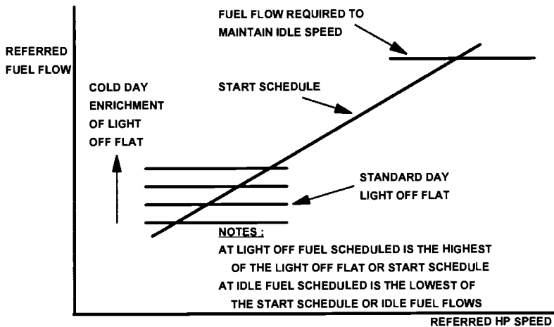
Fig. 9.5 Referred fuel flow versus referred speed start fuel schedule.
