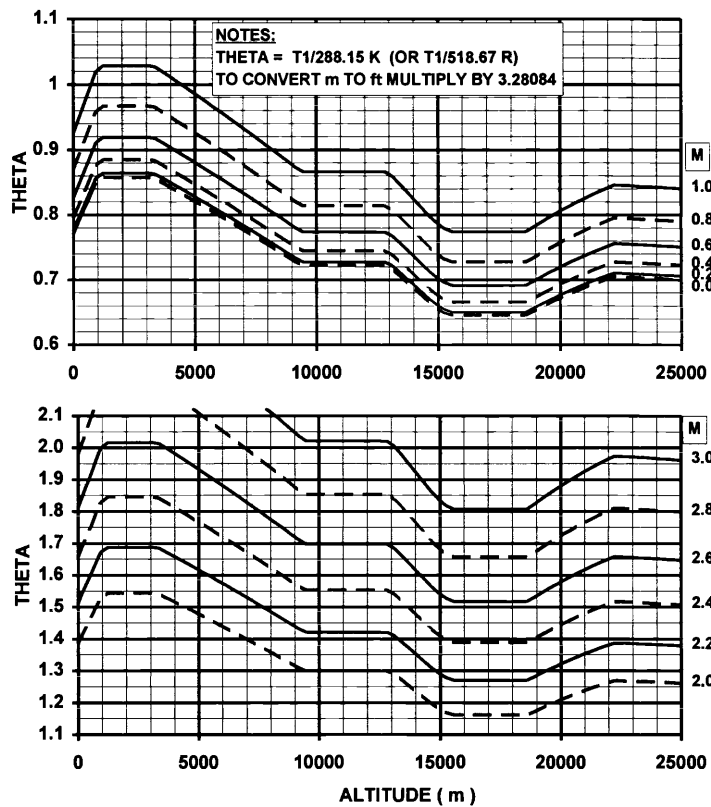
(a) For MILSTD 210 cold day
