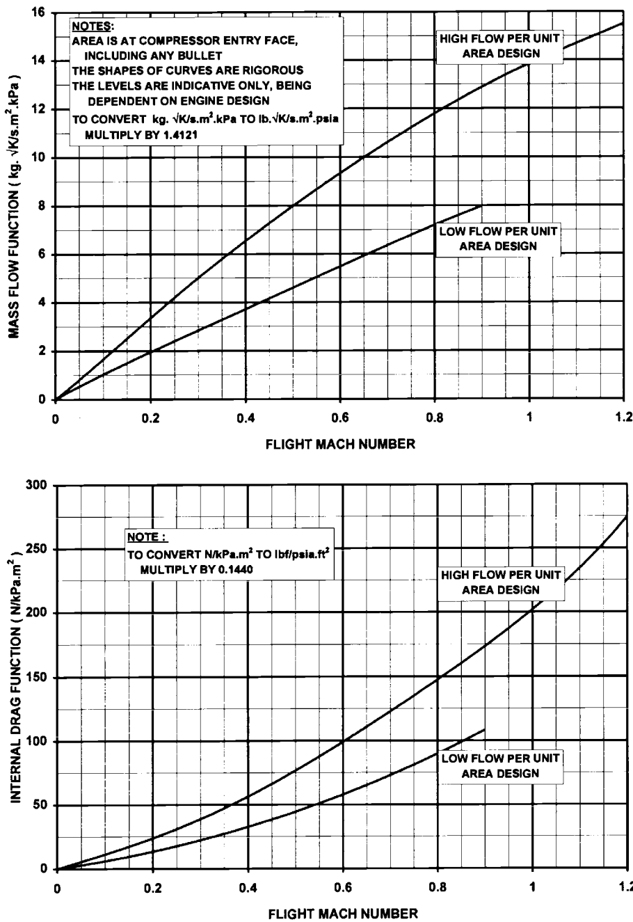
Chart 10.3 Turbojet windmilling: mass flow and internal drag versus flight Mach number.
