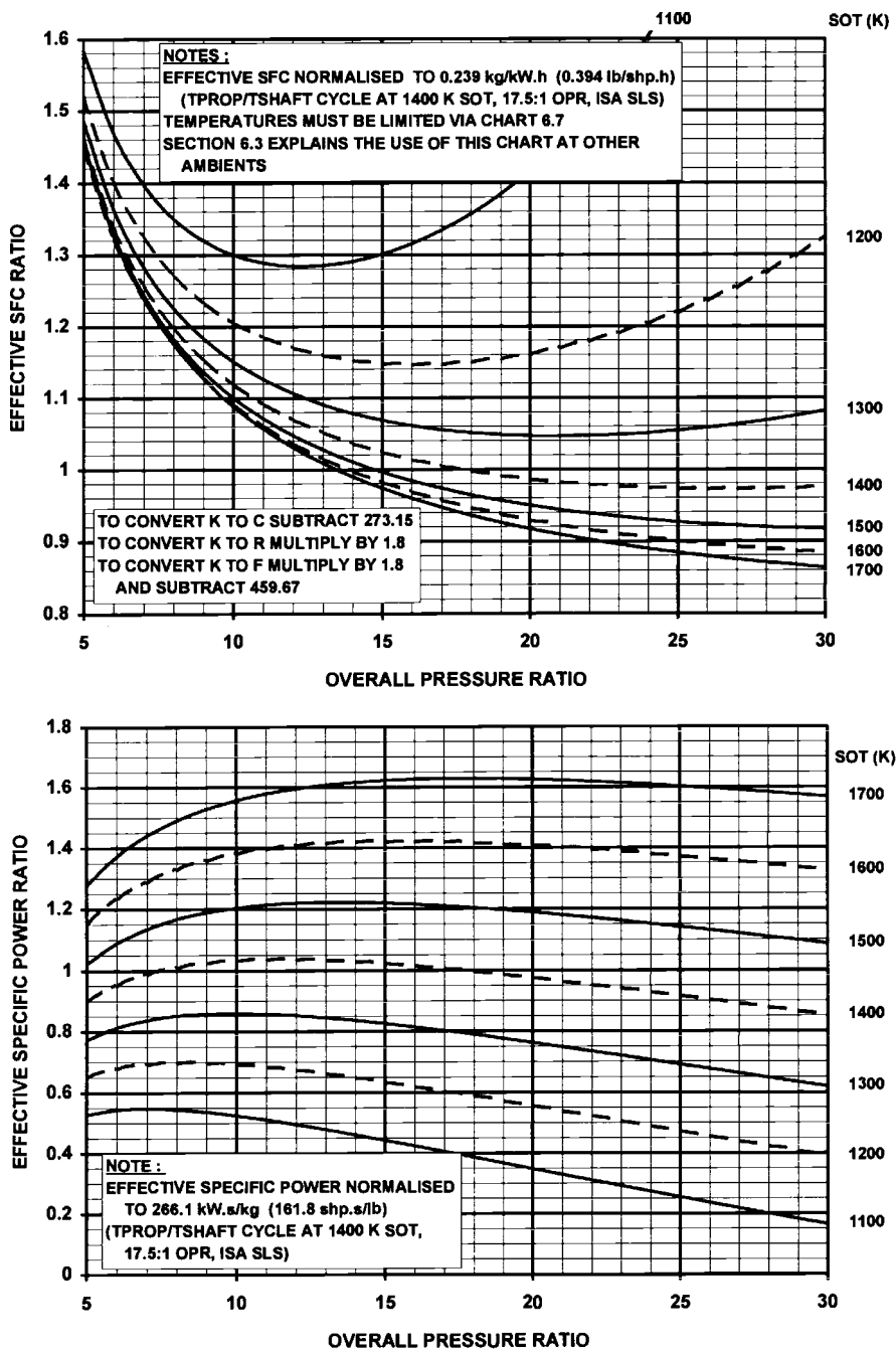
Chart 6.14 Turboshaft and turboprop cycles: SFC and specific power versus overall pressure ratio and SOT at ISA SLS (design point diagrams).
