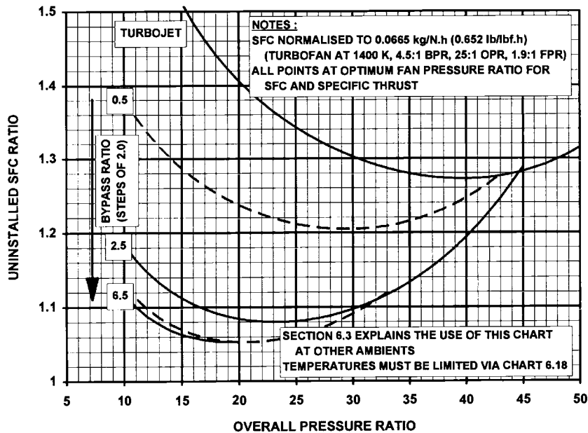
Chart 6.22 Turbopan cycles: SFC versus overall PR and bypass ratio at optimum fan PR at 11 000 m, ISA, 0.8 M (design point diagrams).
