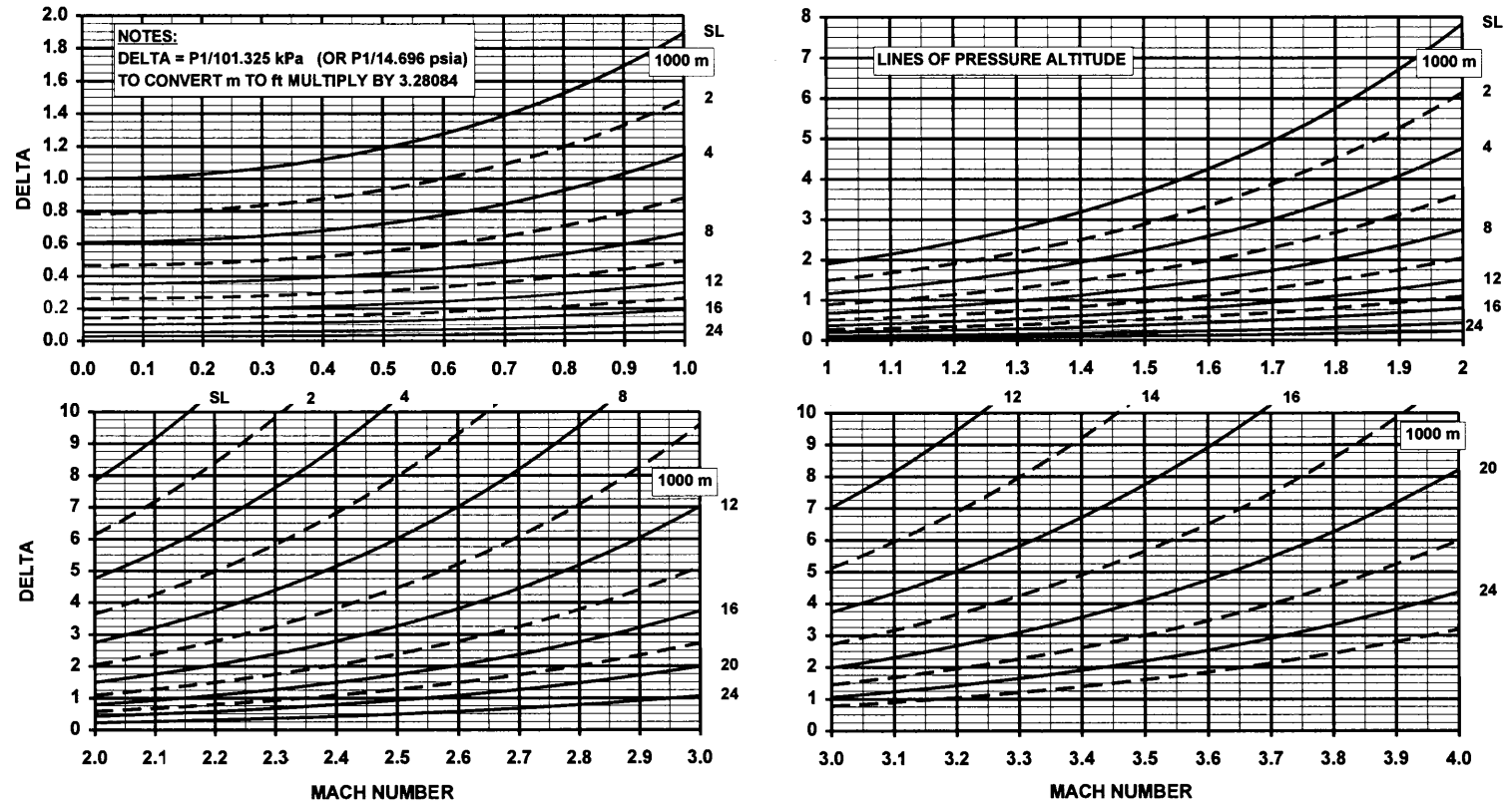
Chart 2.10 Delta versus altitude and Mach number.
