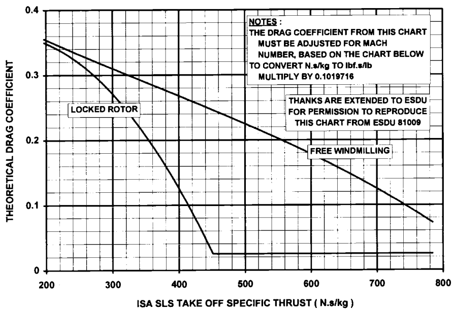
(a) Theoretical drag coefficient
