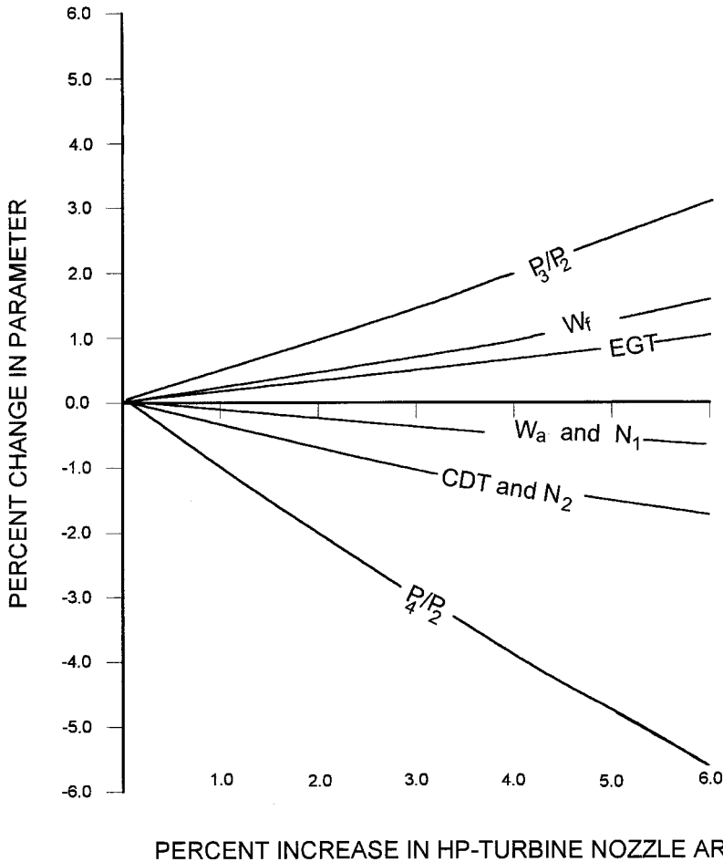
Figure 12-2. Dual spool gas turbine estimated parameter changes with high pressure-turbine nozzle area change.
