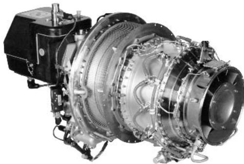
Figure 11-2. Courtesy of United Technologies Corporation, Pratt & Whitney Aircraft. The PW206 turboprop engine is a 700 shaft horsepower engine used primarily in helicopter applications. Current applications include the Agusta A109E Power , Bell M427, Eurocopter EC135P1/P2, and the MDHI MD900/902.
