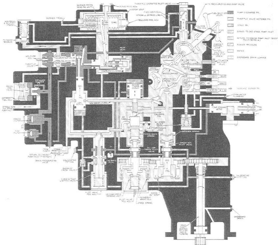
Figure 5-4. Courtesy of United Technologies Corporation, Pratt & Whitney Aircraft. Cutaway drawing of a typical hydromechanical control. This sketch shows the basic fuel-control functions. This type of control was state-of-the-art in the 1960s.
