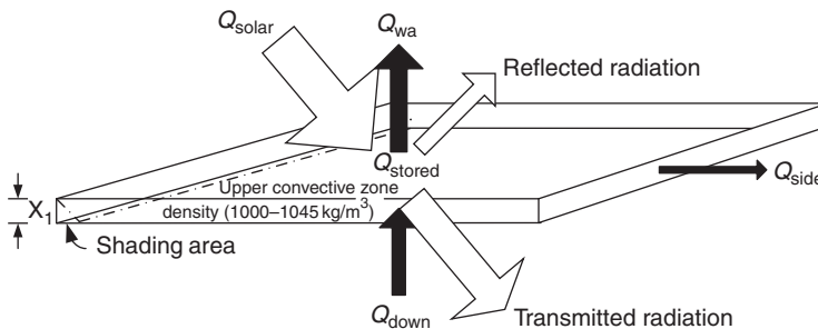
Fig. 10.9. UCZ of the solar pond.
