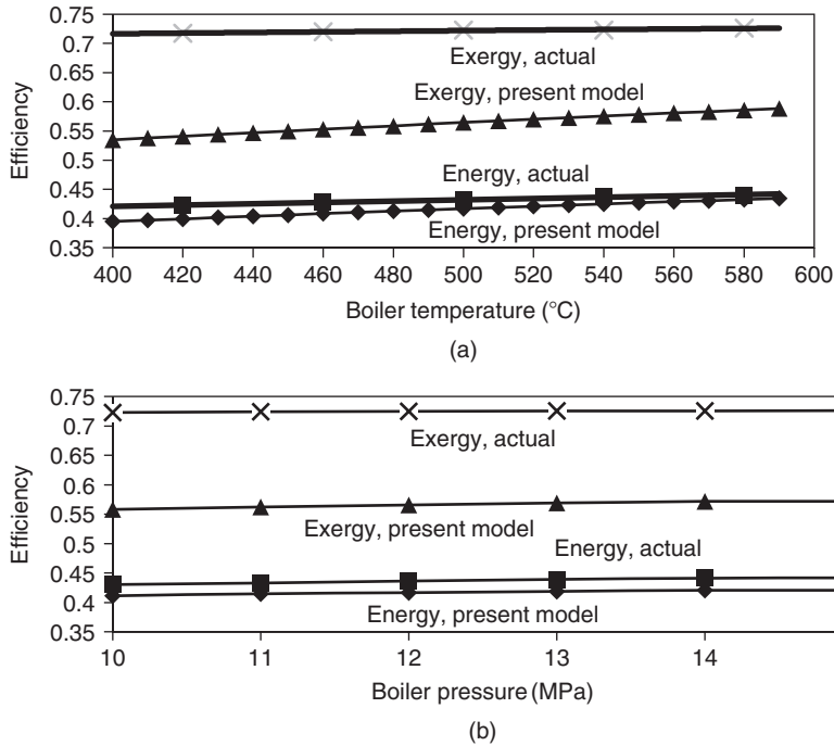
Fig. 11.4. Comparison of the energy and exergy efficiencies for the Ghazlan Power Plant with (a) boiler temperature and (b) boiler pressure, for the actual data presented by Al-Bagawi (1994) and the values calculated with the present model discussed in the text.
