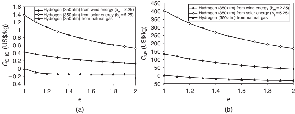
Fig. 19.9. Unit cost of (a) GHG and (b) AP emissions reduction as a result of hydrogen substitution for gasoline, as a function of the ratio in efficiencies \epsilon of internal combustion (gasoline powered) and fuel cell (hydrogen powered) vehicles.
