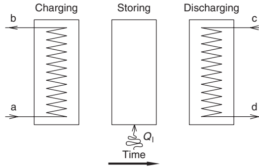
Fig. 9.10. The three processes in a general CTES system: charging (left), storing (middle) and discharging (right). The heat leakage into the system Q_1 is illustrated for the storing process, but can occur in all three processes.
