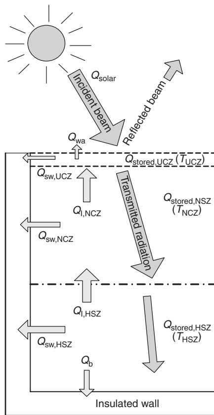
Fig. 10.7. Half-cut view of an insulated solar pond.
