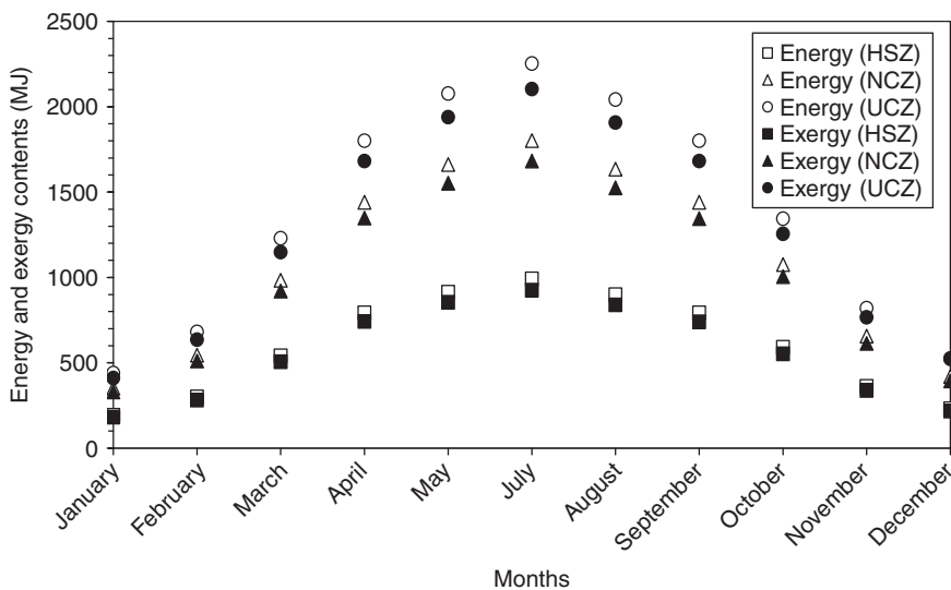
Fig. 10.20. Energy and exergy content distributions of the solar pond zones.
