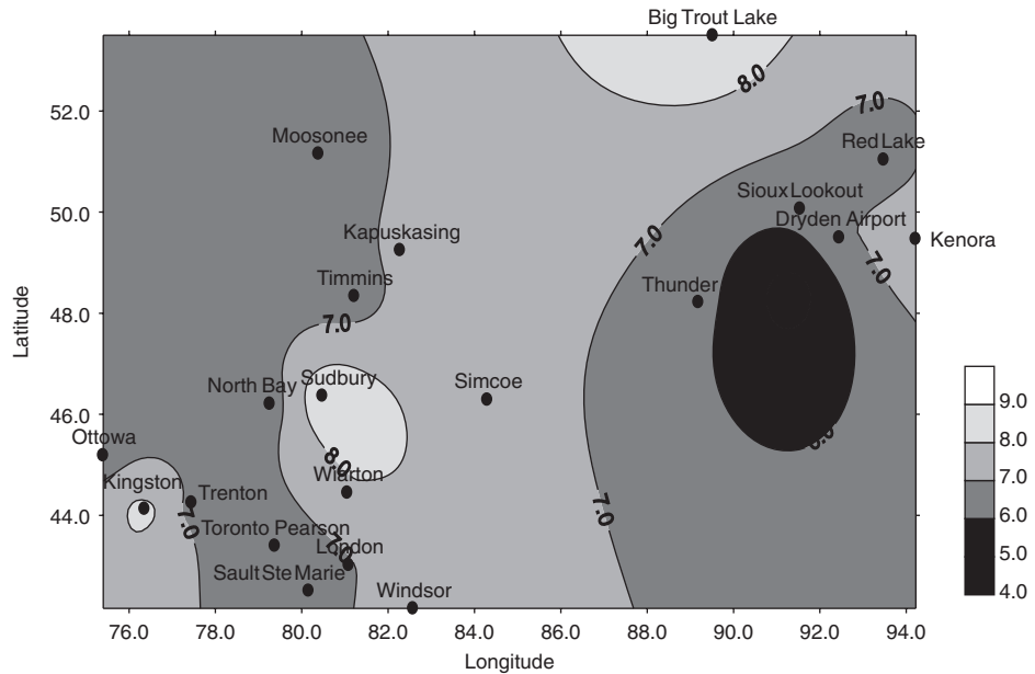
Fig. 10.35a. October wind speed map for 30 m for Ontario.
