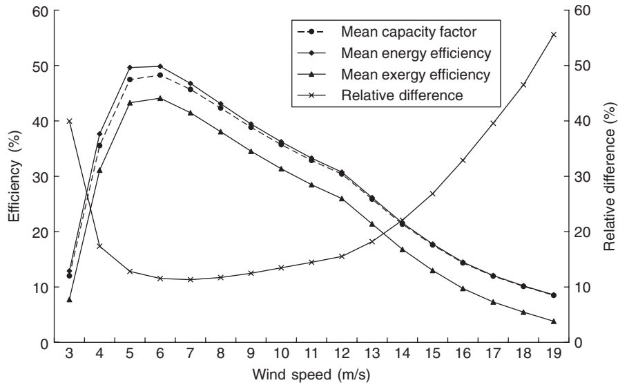
Fig. 10.31. Mean exergy and energy efficiencies, and percent differences between these values, as a function of wind speed. Mean capacity factor is also shown.
