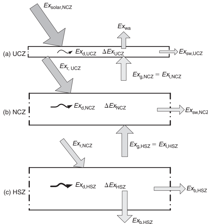
Fig. 10.19. Energy and exergy flows in the inner zones of the solar pond.
