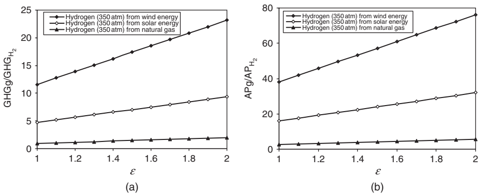
Fig. 19.10. Reductions of (a) GHG and (b) AP emissions as a result of hydrogen substitution for gasoline, as a function of the ratio in efficiencies \epsilon of internal combustion (gasoline powered) and fuel cell (hydrogen powered) vehicles.
