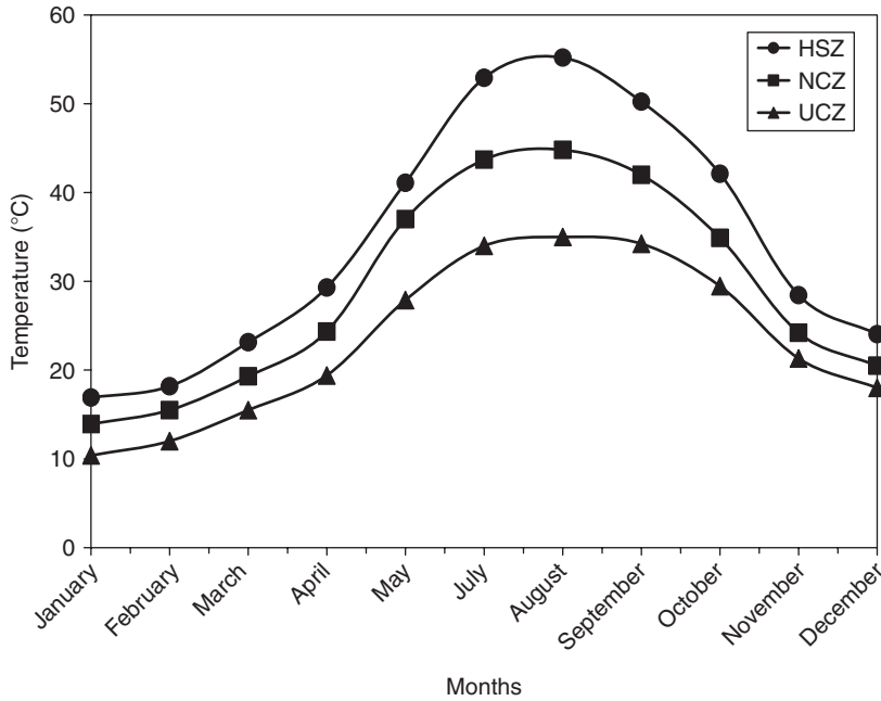
Fig. 10.13. Monthly average temperatures for the inner zones of the pond.
