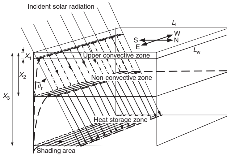
Fig. 10.8. Schematic of the insulated solar pond.
