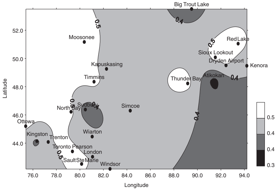
Fig. 10.35b. October energy efficiency map for Ontario.
