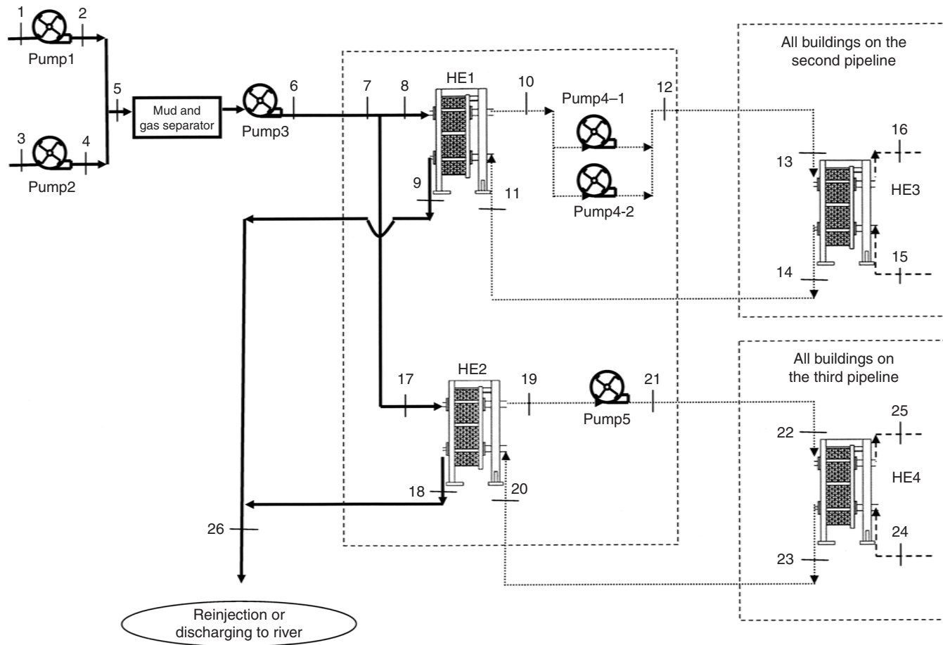
Fig. 10.36. Schematic of the Bigadic GDHS.
