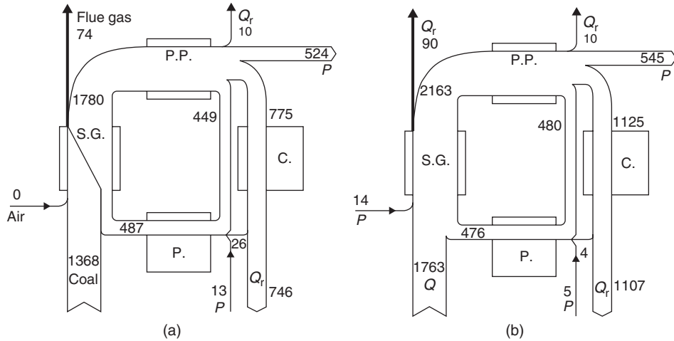
Fig. 11.6. Simplified process diagrams for single units of (a) NGS and (b) PNGS, indicating net energy flow rates (MW) for streams. Stream widths are proportional to energy flow rates. Sections of stations shown are steam generation (S.G.), power production (P.P.), condensation (C.) and preheating (P.). Streams shown are electrical power ( P ), heat input ( Q ) and heat rejected ( Q_r ).
