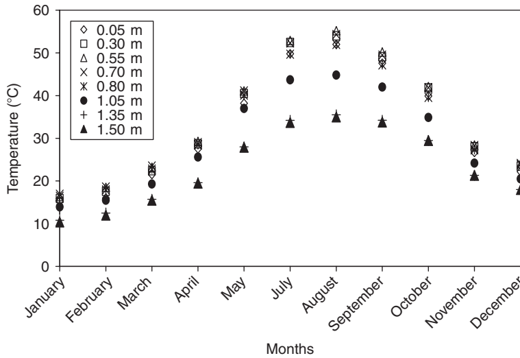
Fig. 10.14. Experimental zone temperature distributions in the inner zones of the solar pond.
