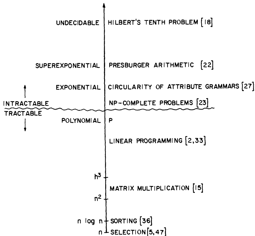
FIG. 1.3. The spectrum of computational complexity.
