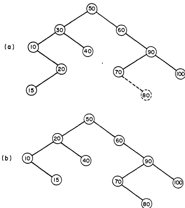
FIG. 4.1. Insertion and deletion in a binary search tree. External nodes are omitted. (a) Insertion of item with key 80. (b) Deletion of item with key 30. It is replaced by its predecessor, with key 20, which is in turn replaced by its left child, with key 15.
