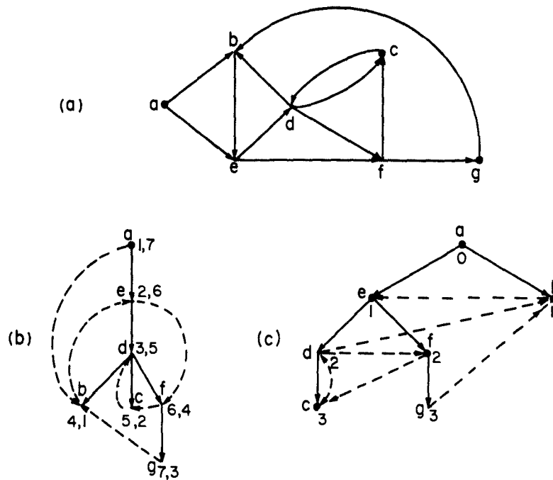
FIG 1.10. Graph search. (a) Graph. (b) Depth-first search. Edges of spanning tree are solid, other edges dashed. Vertices are numbered in preorder and postorder. If edges [b, e] and [c, d] are deleted, graph becomes acyclic, and postorder is a reverse topological order. (c) Breadth-first search. Vertex numbers are levels.
