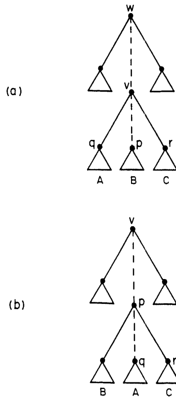
FIG. 5.6. Effect of a splice on a virtual tree. (a) Relevant part of virtual tree after operation \text{findpath}(v) . Triangles denote solid subtrees. Vertex v is now the root of its solid tree. (b) After completing the splice.
