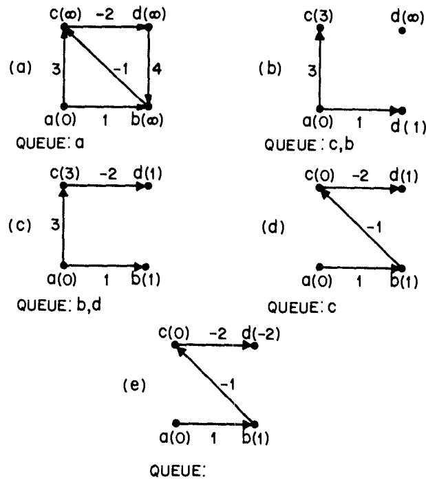
FIG. 7.6. Breadth-first scanning. (a) Input graph with initial queue of labeled vertices. (b) After scanning vertex a. (c) After scanning vertex c. (d) After scanning vertices b and d. (e) After rescanning vertices c and d, the method stops.
