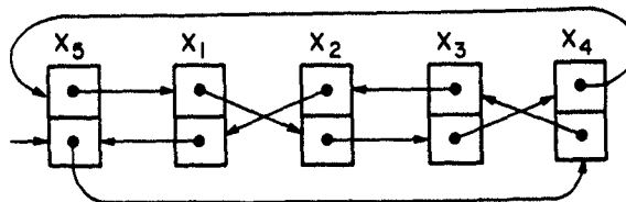
FIG. 1.8. Endogenous representation of a reversible list.
