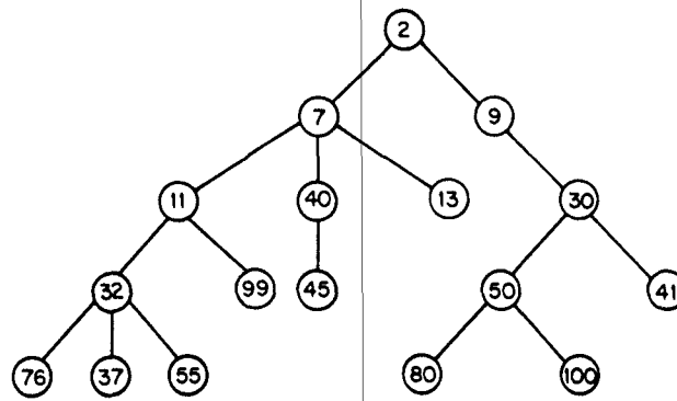
FIG. 3.1. A heap-ordered tree. Numbers in nodes are keys. (To simplify this and subsequent figures, we treat the keys as if they themselves are the items.)
