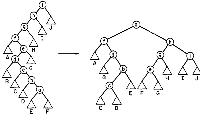
FIG. 4.10. Splay at node a .
