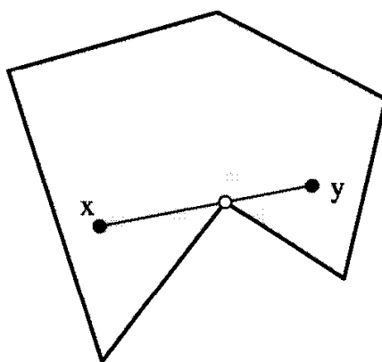
FIGURE 1.2 Grazing contact of line of sight.
