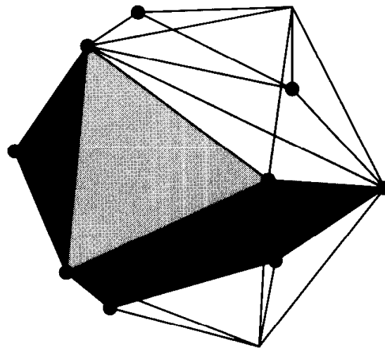
FIGURE 7.23 P_1 : 9 vertices, 14 faces (Figure 7.21(c)).
