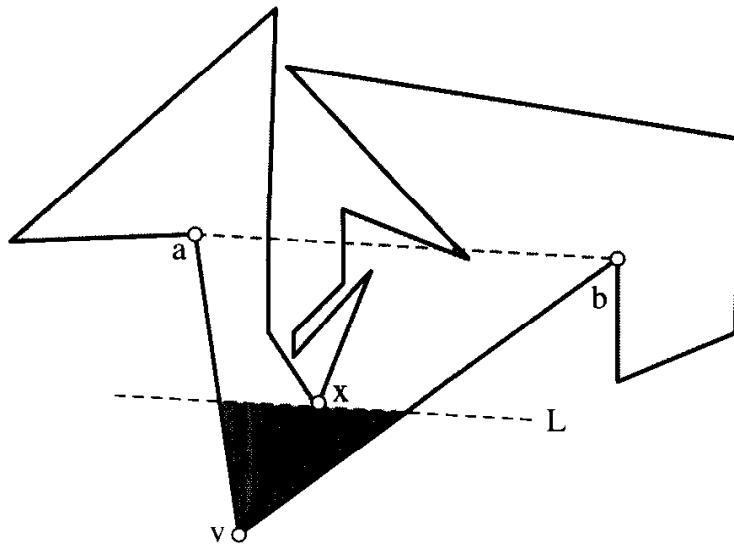
FIGURE 1.12 vx must be a diagonal.
