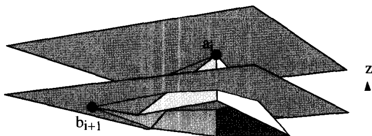
FIGURE 7.27 Highest point a_i of P_i .
