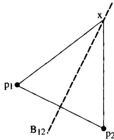
FIGURE 5.2 Two sites: |p_1x| = |p_2x| .
