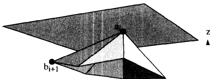
FIGURE 7.27 Highest point a_i of P_i .
