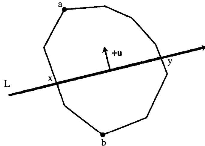
FIGURE 7.20 Stabbing a convex polygon.
