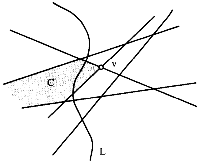
FIGURE 6.14 Vertex v is sweepable.
