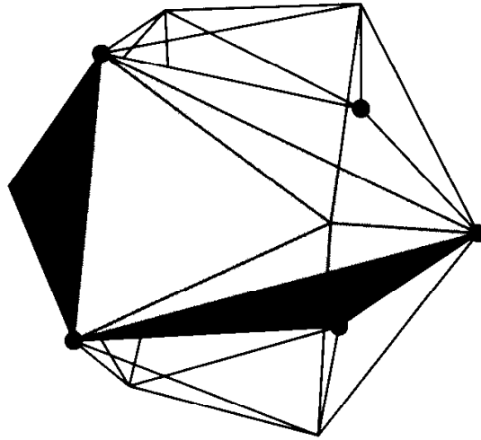
FIGURE 7.24 P_2 : an octahedron (Figure 7.21(e)).
