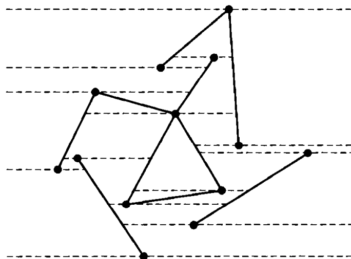
FIGURE 7.33 The trapezoid decomposition induced by n = 10 segments.
