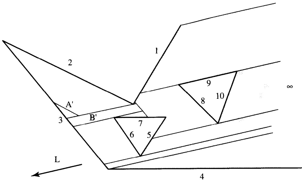
FIGURE 8.13 Cell decomposition, with ladder tilted.
