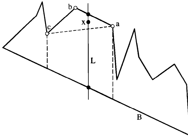
FIGURE 2.6 A monotone mountain with base B ; b is an ear tip.
