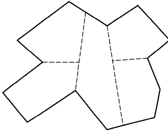
FIGURE 2.10 r + 1 convex pieces: r = 4 ; 5 pieces.
