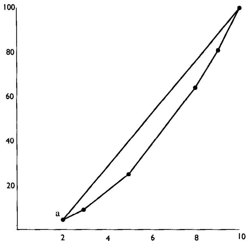
FIGURE 3.9 Parabola construction for sorting (2, 3, 5, 8, 9, 10).
