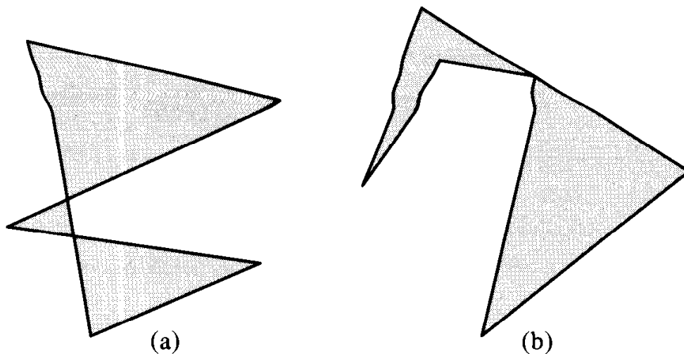
FIGURE 1.1 Nonsimple polygons.
