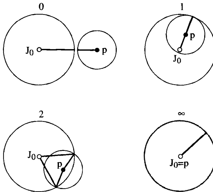
FIGURE 8.21 2-Link reachability: number of solutions shown.
