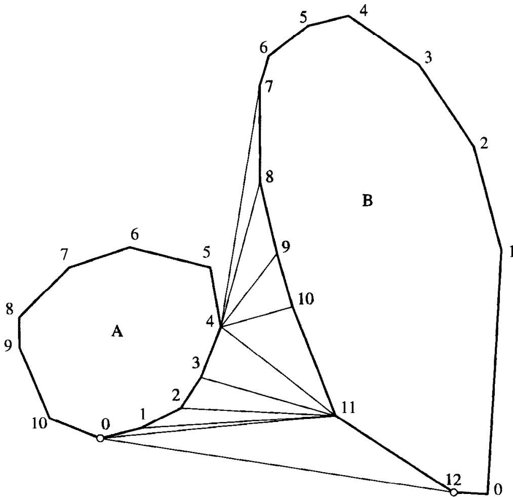
FIGURE 3.11 Finding the lower tangent: from (4, 7) to (0, 12).
