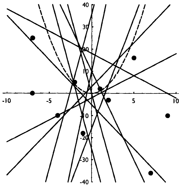
FIGURE 6.7 The duals of the lines in Figure 6.1.
