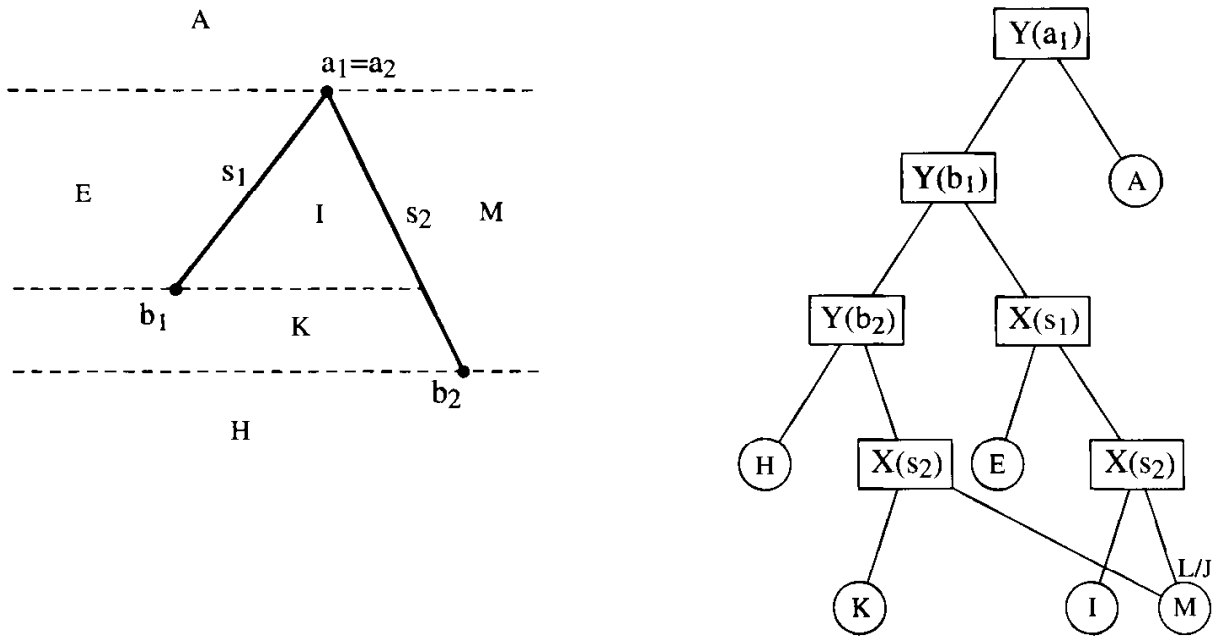
FIGURE 7.37 Search tree after merging regions along s_2 .
