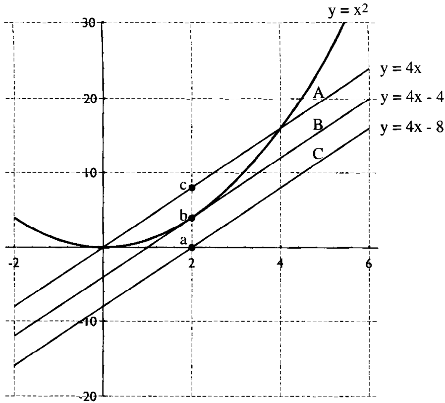
FIGURE 6.6 \mathbb{D}(a) = A , \mathbb{D}(b) = B , \mathbb{D}(c) = C .
