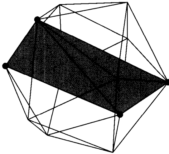
FIGURE 7.25 P_3 : a flat tetrahedron (Figure 7.21(g)).
