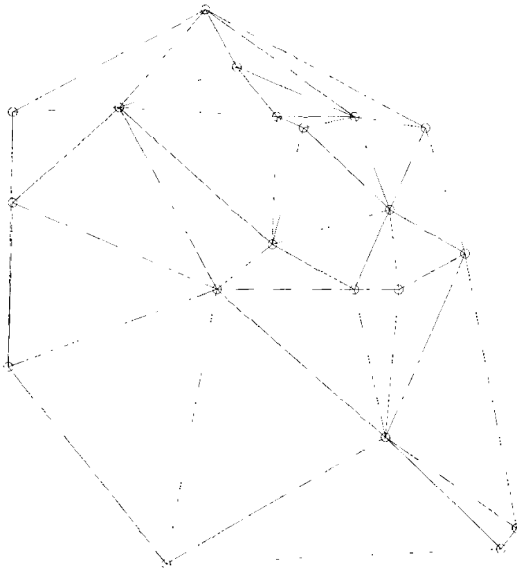
FIGURE 5.6 Delaunay triangulation for the sites in Figure 5.5.
