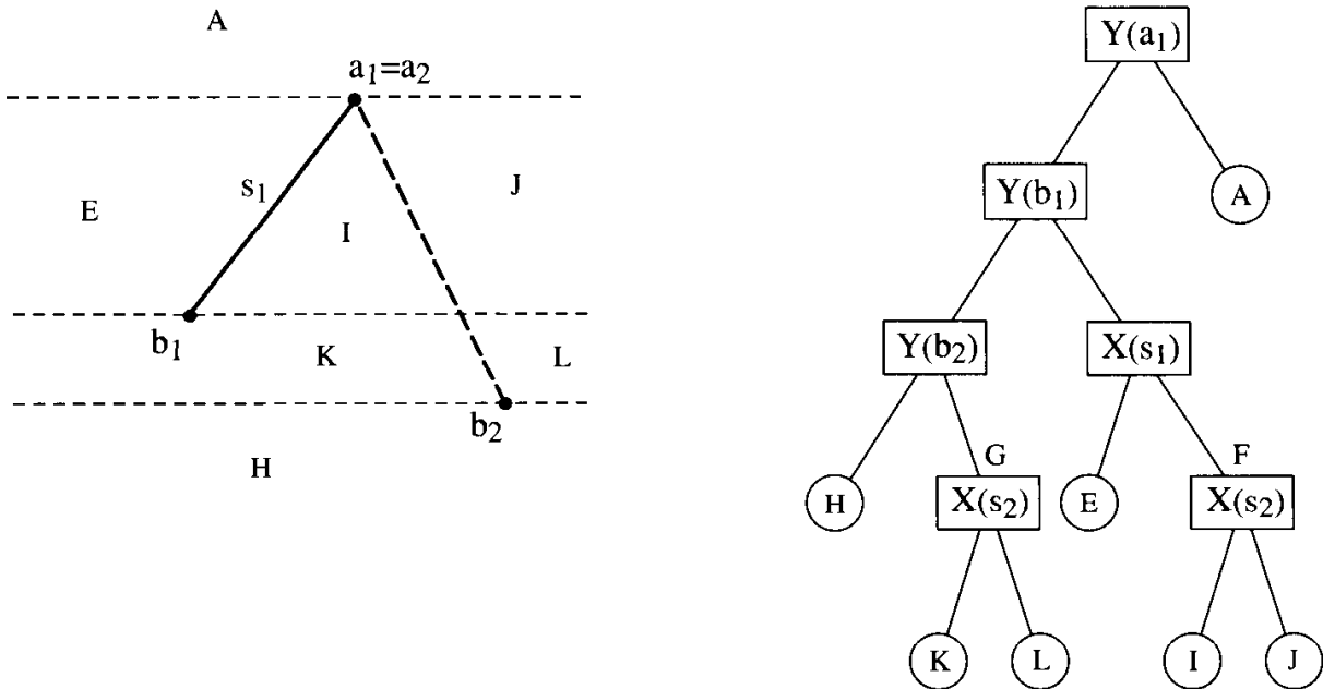
FIGURE 7.36 Search tree after threading s_2 .
