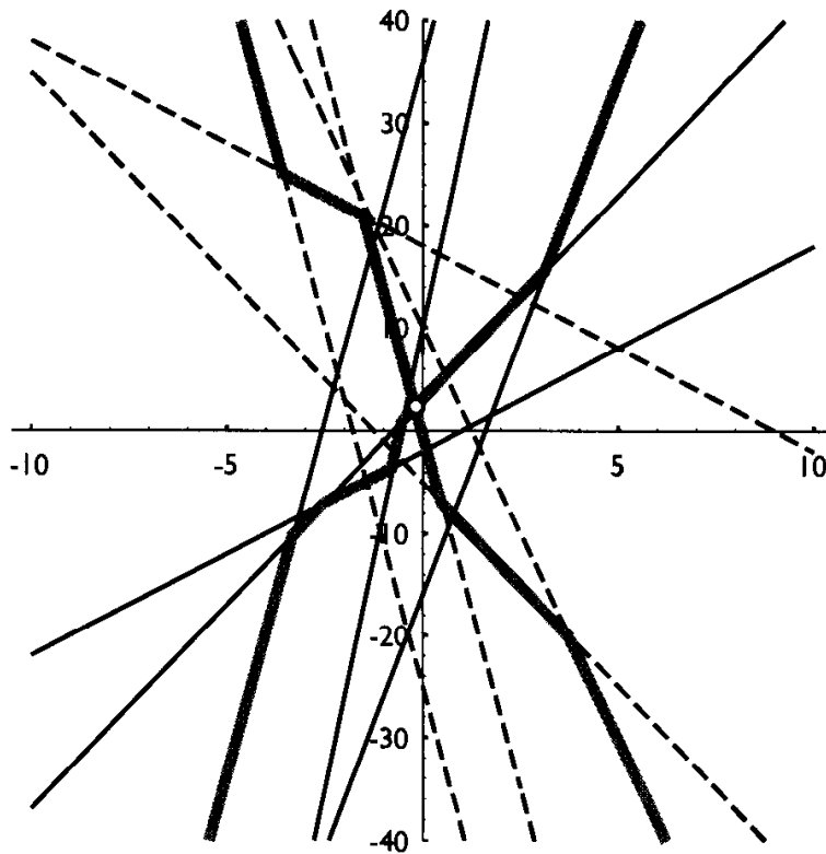
FIGURE 6.20 \mathcal{A} and \mathcal{B} together. The intersection of their median levels is at (-\frac{1}{6}, 2\frac{1}{3}) .
