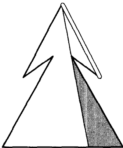
FIGURE 1.8 \lfloor n/4 \rfloor edge guards are necessary (Toussaint).
