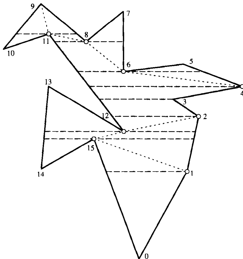
FIGURE 2.7 A partition into monotone mountains.
