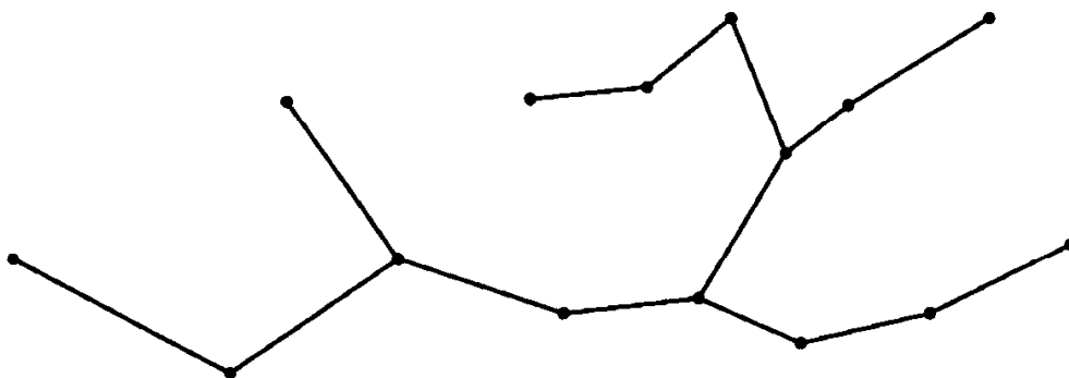
FIGURE 5.15 A Euclidean Minimum Spanning Tree.
