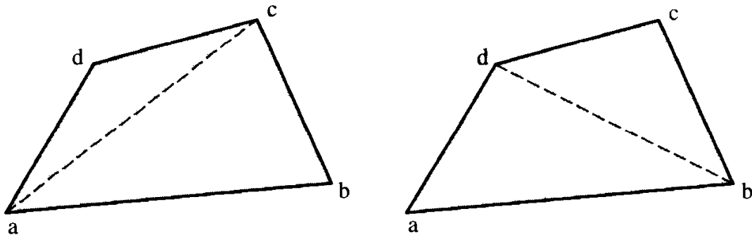
FIGURE 1.17 The two triangulations of a convex quadrilateral.
