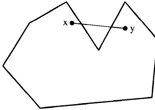
FIGURE 3.1 Any dent implies nonconvexity.
