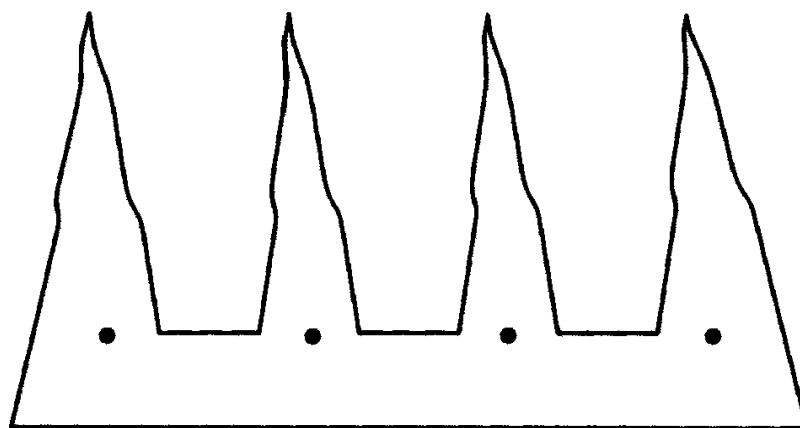
FIGURE 1.5 Chvátal's comb for n = 12 .
