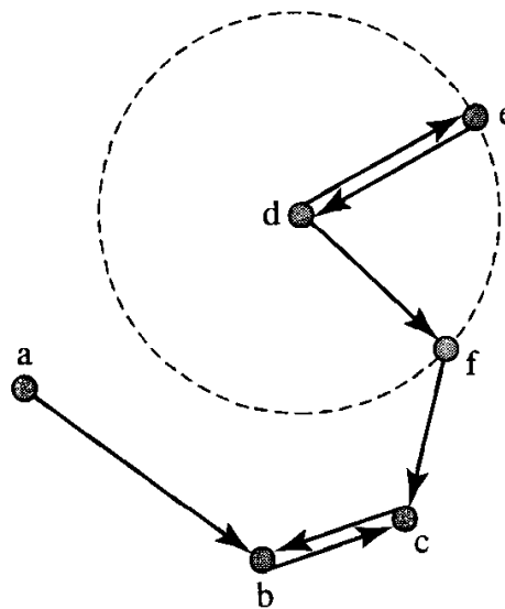
FIGURE 5.12 a \rightarrow b , but b \rightarrow c ; also d \rightarrow e and d \rightarrow f .
