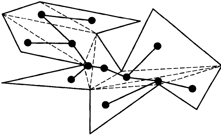
FIGURE 1.14 Triangulation dual.
