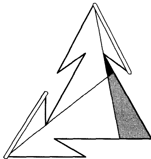
FIGURE 1.8 \lfloor n/4 \rfloor edge guards are necessary (Toussaint).
