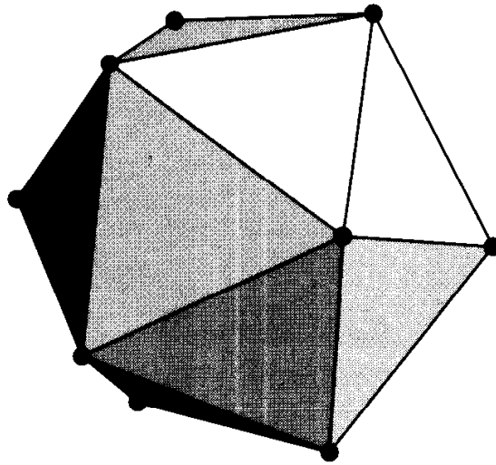
FIGURE 7.22 Icosahedron, P_0 (Figure 7.21(a)).
