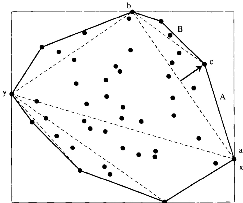
FIGURE 3.3 QuickHull discards the points in \triangle abc (shaded) and recurses on A and B . Here A = \emptyset and |B| = 2 .
