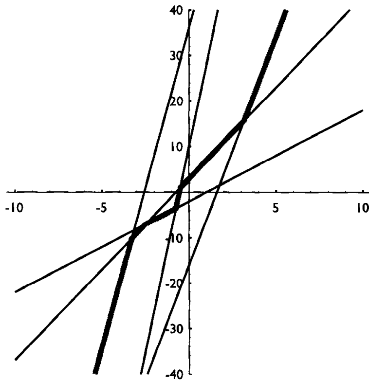
FIGURE 6.18 The duals of the points with x > 0 (set A in Figure 6.17) all have positive slope.
