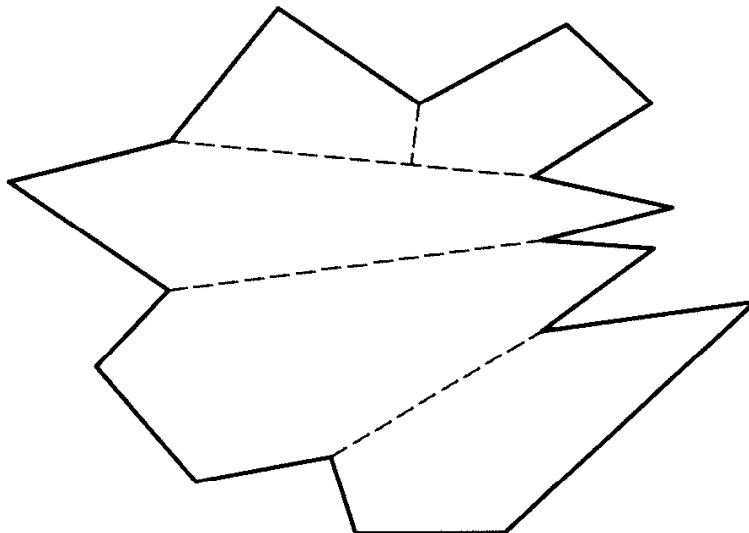
FIGURE 2.11 \lceil r/2 \rceil + 1 convex pieces: r = 7 ; 5 pieces.
