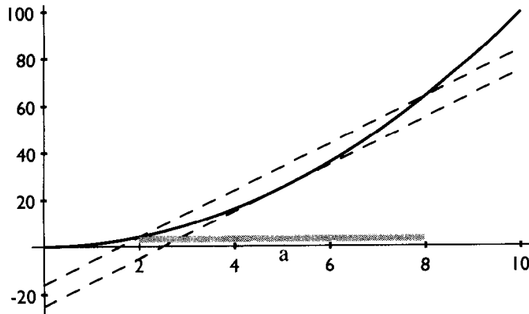
FIGURE 5.23 For a = 5 , the tangent is z = 10x - 25 .
