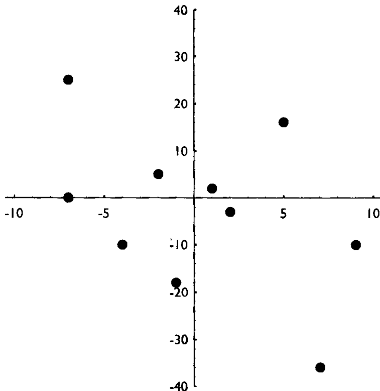
FIGURE 6.8 The points from Figure 6.7: \{(-7, 25), (-7, 0), (-4, -10), (-2, 5), (-1, -18), (1, 2), (2, -3), (5, 16), (7, -36), (9, -10)\} .
