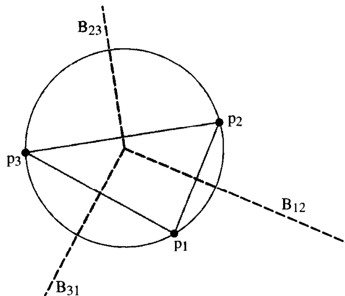
FIGURE 5.3 Three sites: bisectors meet at circumcenter.
