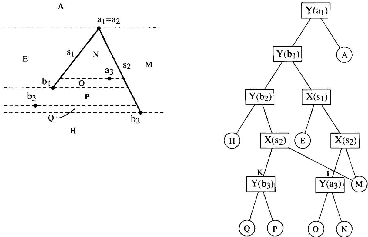
FIGURE 7.38 Search tree after inserting a_3 and b_3 .
