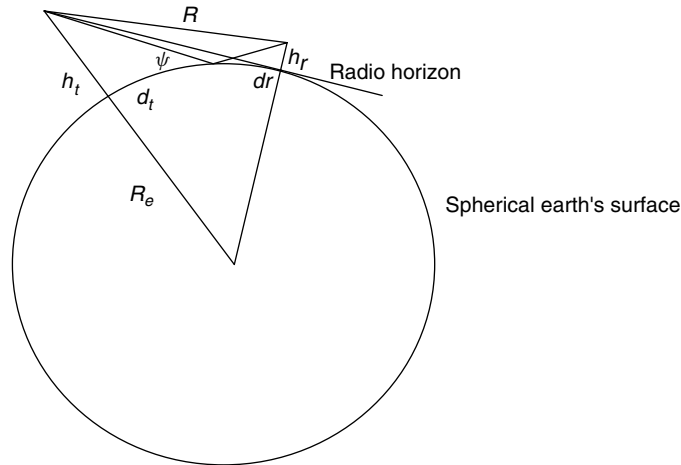
Figure 7-2. Broadcast antenna geometry.
