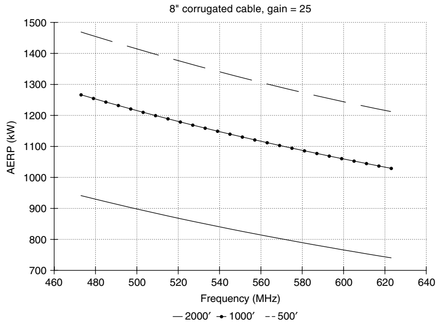
Figure 6-10. Maximum AERP.
