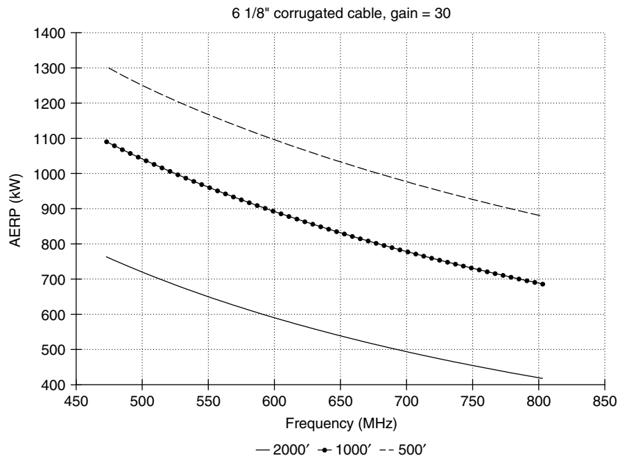
Figure 6-9. Maximum AERP.
