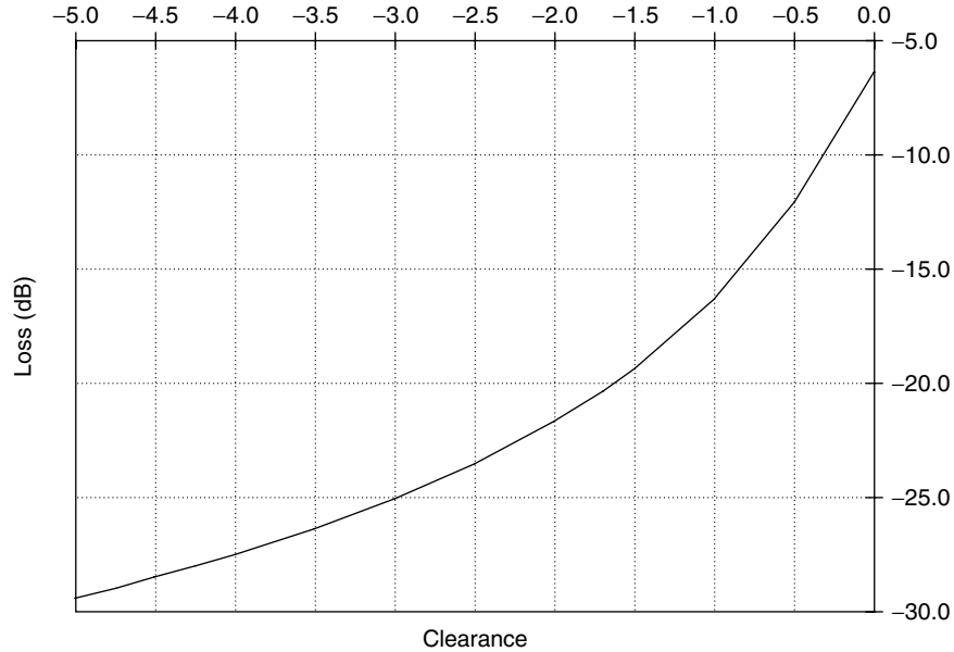
Figure 8-11. Knife-edge diffraction.
