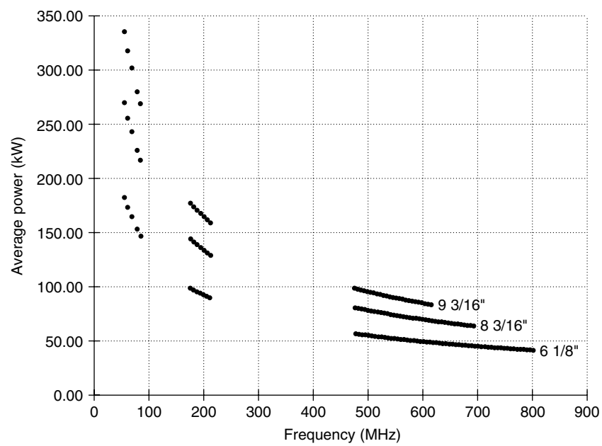
Figure 6-2. Rigid coax power rating.
