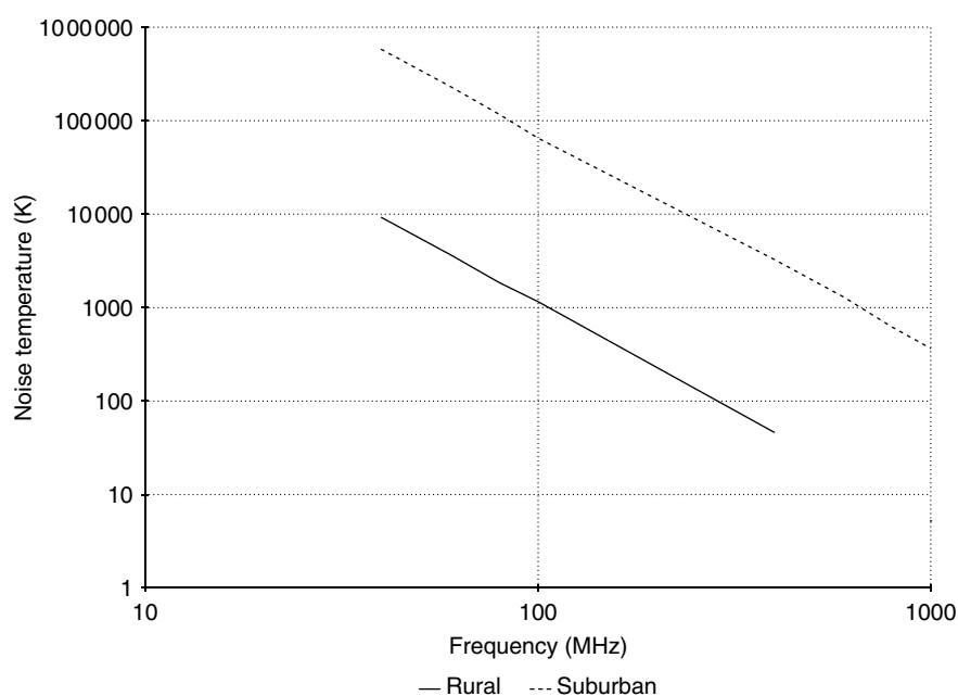
Figure 2-1. External noise temperature. (From Reference Data for Radio Engineers , 6th ed., Howard W. Sams, Indianapolis, Ind., 1977, p. 29-2; used with permission.)
