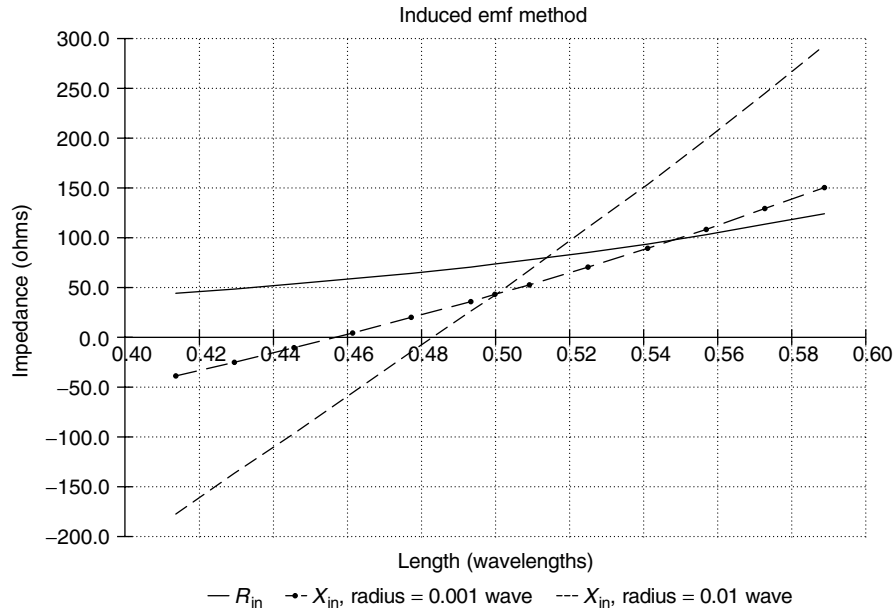
Figure 7-33. Dipole impedance.
