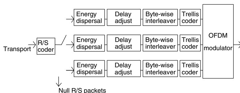
Figure 1-12. Block diagram of ISDB-T channel coding.
