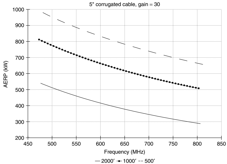
Figure 6-8. Maximum AERP.
