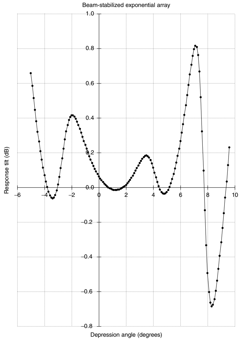
Figure 7-18. Frequency-response tilt.
