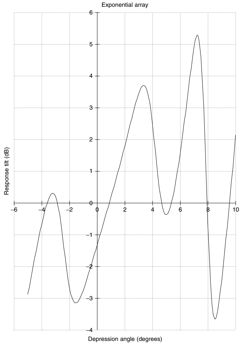
Figure 7-16. Frequency-response tilt.
