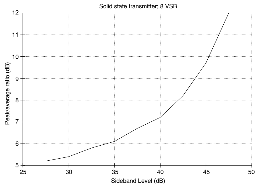
Figure 4-7. Peak-to-average ratio versus sideband level. (From M.J. Horspool, "A New Solid State UHF Television Transmitter Design for Digital Terrestrial Broadcasting," Conference Proceedings of the International Conference and Exhibition on Terrestrial and Satellite Broadcasting , New Delhi, India, January 9–21, 1998.)
