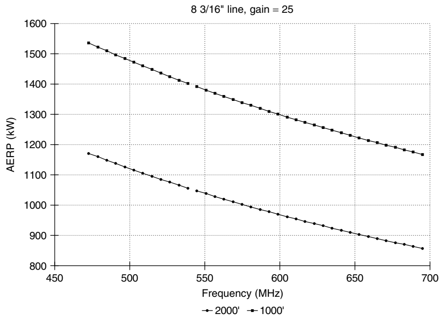
Figure 6-4. Maximum AERP.
