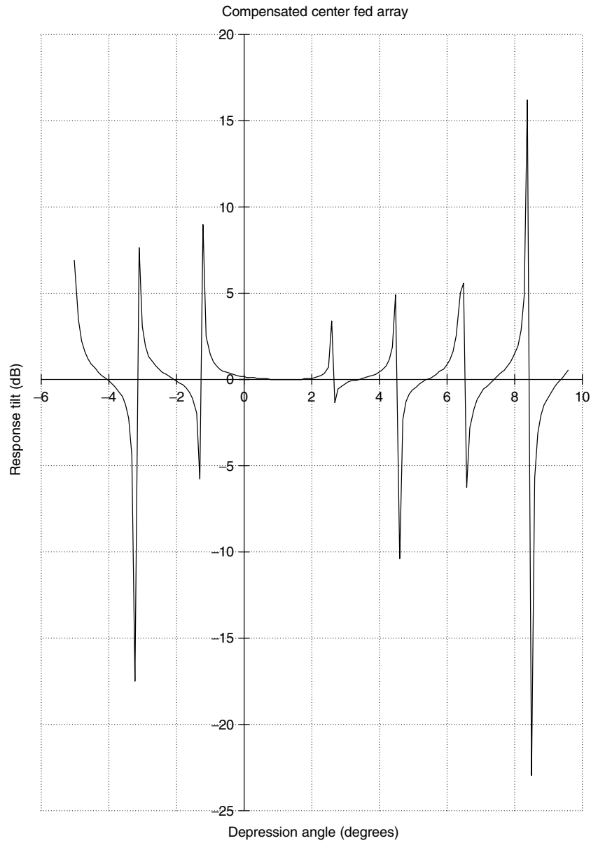
Figure 7-13. Frequency-response tilt.
