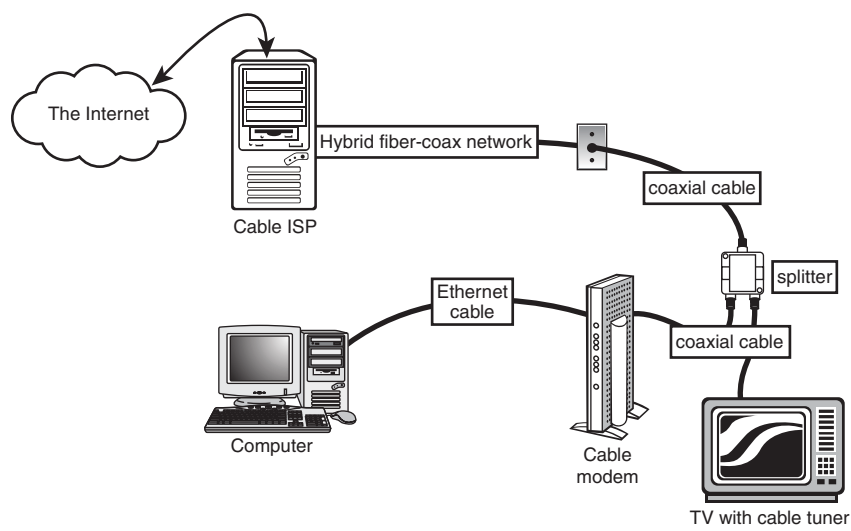
Figure 16.1 A typical hybrid fiber-coax cable TV network that also includes two-way cable modem service.
