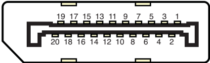
Figure 12.10 DisplayPort socket and pin configuration.
