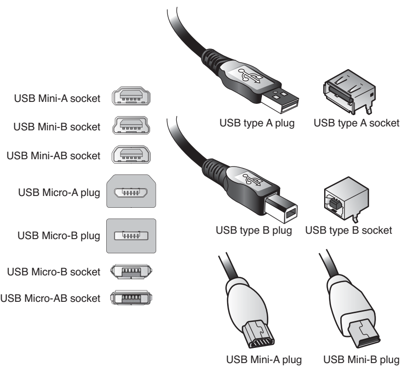
Figure 14.7 USB plugs and sockets. Note that a Mini-AB socket is a dual-purpose socket that can accept either Mini-A or Mini-B plugs. Likewise, a Micro-AB socket is a dual-purpose socket for either Micro-A or Micro-B plugs. (There is no Micro-A socket.) The newer Mini and Micro plugs and sockets have plastic portions inside the connectors that are required to be color coded, as shown in Table 14.3.
