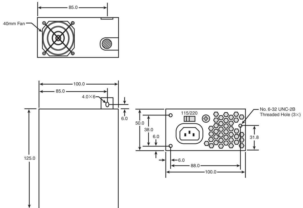
Figure 18.5 SFX/SFX12V low-profile power supply with internal 40mm fan.
