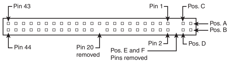
Figure 7.4 The 50-pin unitized PATA connector detail (used on 2 1/2-inch notebook/laptop PATA drives with a 44-pin cable).
