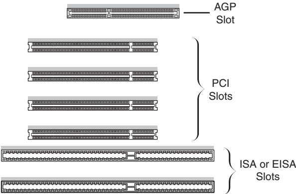
Figure 4.40 Typical configuration of 32-bit 33MHz PCI slots in relation to ISA or EISA and AGP slots.
