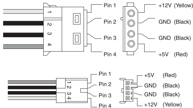
Figure 18.30 Peripheral and floppy power connectors.
