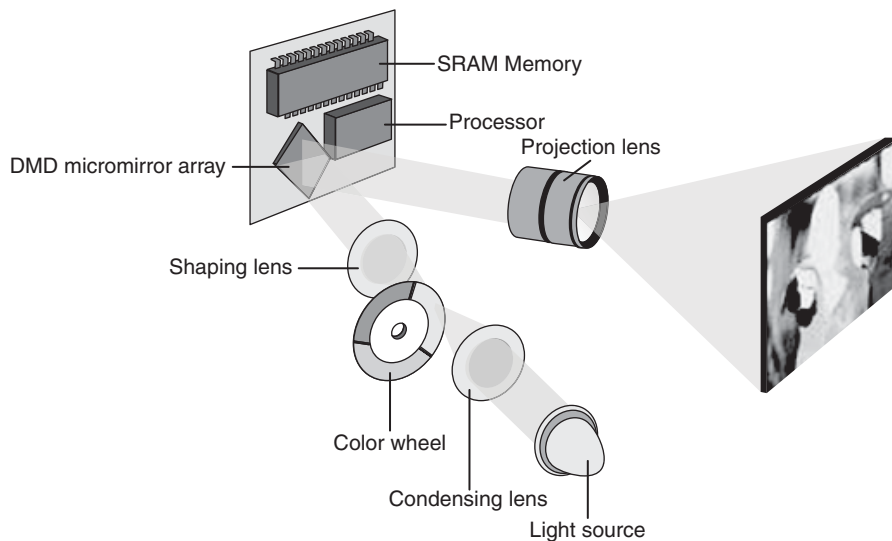
Figure 12.25 How a typical DLP projector works.
