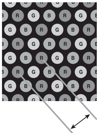
Figure 12.18 Dot-shaped subpixels, where pixel or dot pitch is the shortest distance between same color subpixels.
