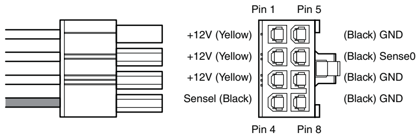
Figure 18.34 PCI Express 8-pin (2x4) auxiliary 150W power supply connector.
