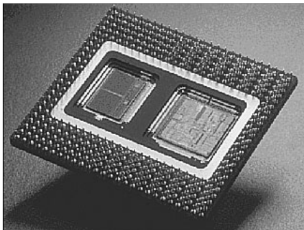
Figure 3.22 Pentium Pro processor with 256KB L2 cache. (The cache is on the left side of the processor die.) Photograph used by permission of Intel Corporation.
