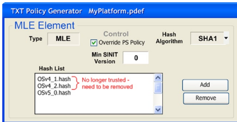
Figure 3-13. MLE policy generator
