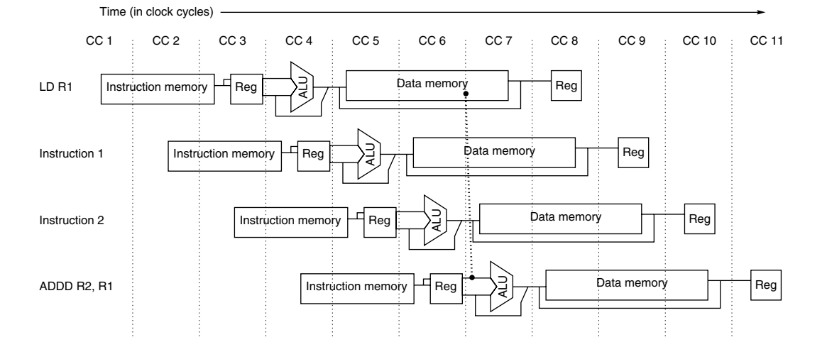
Figure A.38 The structure of the R4000 integer pipeline leads to a 2-cycle load delay. A 2-cycle delay is possible because the data value is available at the end of DS and can be bypassed. If the tag check in TC indicates a miss, the pipeline is backed up a cycle, when the correct data are available.
