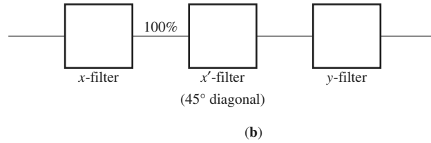
FIGURE 4 Light beams subjected to Polaroid filters.
