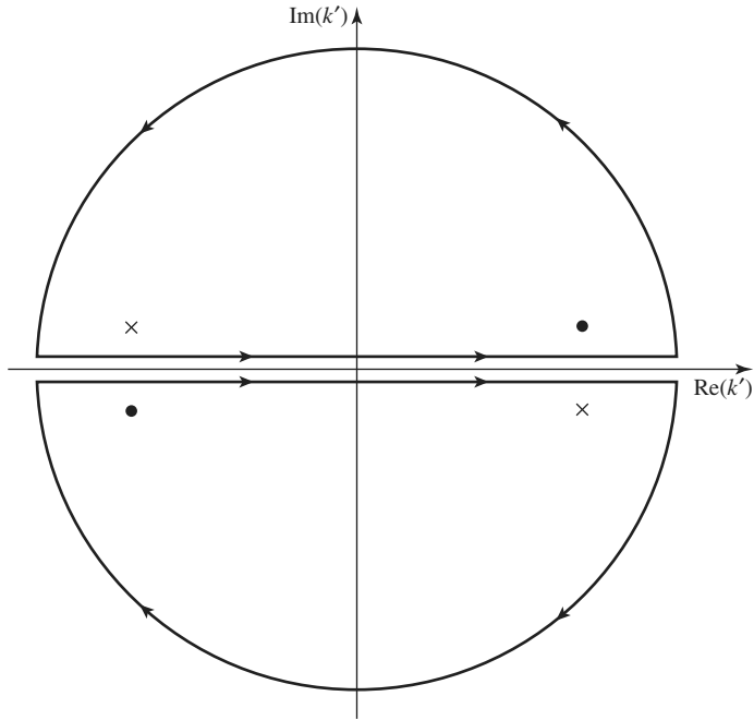
FIGURE 1 Integrating the two terms in (2.9) using complex contours. The dots (crosses) mark the positions of the two poles for the + (−) form of G_{\pm}(\mathbf{x}, \mathbf{x}') . We replace the integral over a real-valued k' in (2.9) with one of the two contours in the figure, choosing the one on which the factor e^{\pm ik'|\mathbf{x}-\mathbf{x}'|} tends to zero along the semicircle at large \text{Im}(k') . Thus, the only contribution to the contour integral is along the real axis.
