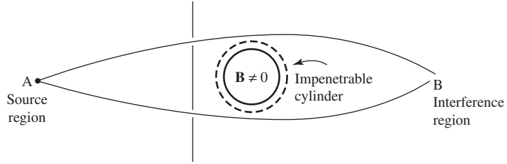
FIGURE 12 The Aharonov-Bohm effect.
