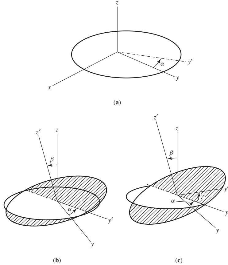
FIGURE 4 Euler rotations.
