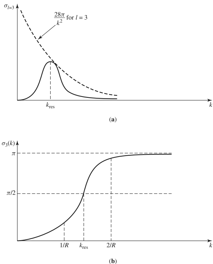
FIGURE 15 Plots of (a) \sigma_{l=3} versus k , where at resonance, \delta_3(k_{\text{res}}) = \pi/2 and \sigma_{l=3} = (4\pi/k_{\text{res}}^2) \times 7 = 28\pi/k_{\text{res}}^2 , and (b) \delta_3(k) versus k . The curves are for a spherical well with 2mV_0R^2/\hbar^2 = 5.5 .
