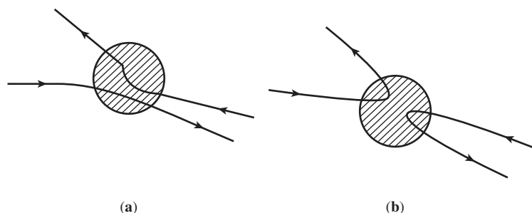
FIGURE 1 Two different paths, (a) and (b), of a two-electron system, for example, in which we cannot assert, even in principle, through which of the paths the electrons pass.
