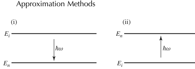
FIGURE 11 (i) Stimulated emission: Quantum-mechanical system gives up \hbar\omega to V (possible only if initial state is excited). (ii) Absorption: Quantum-mechanical system receives \hbar\omega from V and ends up as an excited state.
