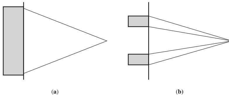
FIGURE 2 (a) Classical physics prediction for results from the Stern-Gerlach experiment. The beam should have been spread out vertically, over a distance corresponding to the range of values of the magnetic moment times the cosine of the orientation angle. Stern and Gerlach, however, observed the result in (b), namely that only two orientations of the magnetic moment manifested themselves. These two orientations did not span the entire expected range.
