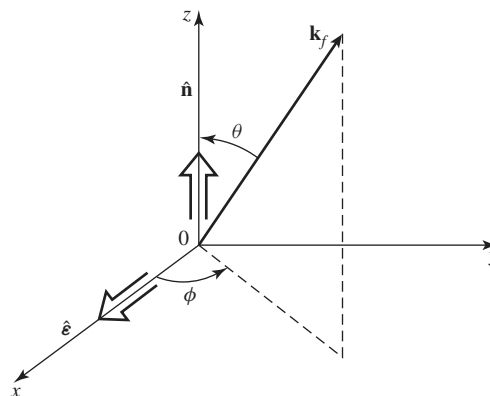
FIGURE 12 Polar coordinate system with \hat{e} and \hat{n} along the x - and z -axes, respectively, and \mathbf{k}_f = (k_f \sin\theta \cos\phi, k_f \sin\theta \sin\phi, k_f \cos\theta) .
