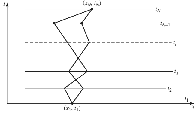
FIGURE 6 Paths in the xt -plane.
