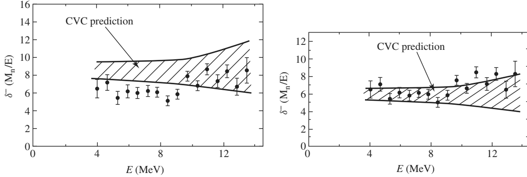
FIGURE 2 Dramatic consequences arise when permutation symmetry is neglected. The data points are from R. D. McKeown et al., Phys. Rev. C22 (1980) 738, who test a prediction of the Conserved Vector Current (CVC) hypothesis. The \beta^\pm - \alpha correlation \delta^- is plotted against the \beta^\pm energy. The prediction comes from a different, previous experiment, which at first neglected permutation symmetry. The corrected plot is on the right, from R. D. McKeown et al., Phys. Rev. C26 (1982) 2336, where the CVC prediction is smaller by a factor of \sqrt{2} .
