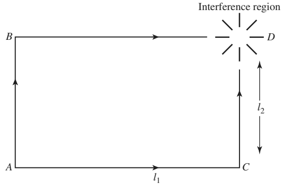
FIGURE 9 Experiment to detect gravity-induced quantum interference.
