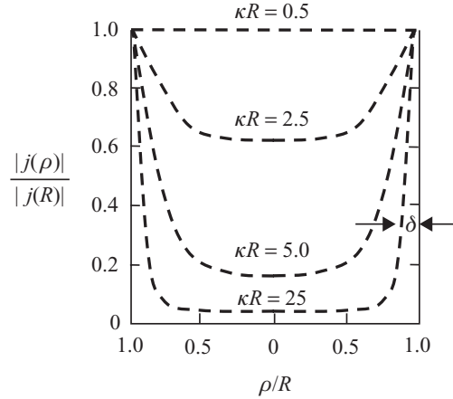
Figure 14.13: The magnitude of the current density |j(\rho)| normalized to its value at the surface of the wire for different values of \kappa R . The thickness of the skin layer for \kappa R = 25 is indicated by \delta . Figure adapted from King (1945).
