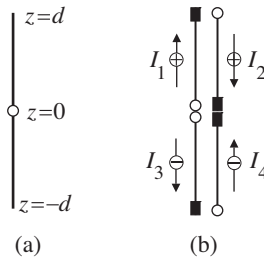
Figure 20.12: (a) A dipole antenna; (b) four linear end-fed antennas. For each, a wave of current launches from the open circle and is absorbed at the closed square. Plus and minus signs identify the charge driven in the direction of the arrows. Figure adapted from Smith (2001). Copyright 2001, American Association of Physics Teachers.
