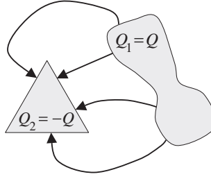
Figure 5.10: The electric field near a two-conductor capacitor.
