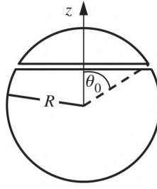
Figure 20.21: A perfectly conducting sphere with a gap at a fixed latitude. A voltage V \cos \omega t is applied across the gap.
