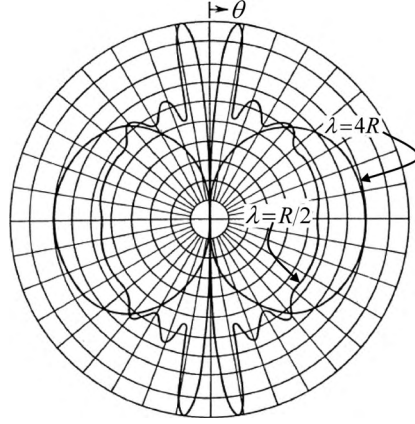
Figure 20.22: The time-averaged angular distribution of power radiated by the slotted sphere in Figure 20.21 with \theta_0 = \pi/2 . Figure from Harrington (1961).
