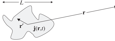
Figure 20.16: To calculate fields in the radiation zone ( r \gg L ), a low-order multipole expansion is valid when \mathbf{j}(\mathbf{r}, t) varies sufficiently slowly in time.
