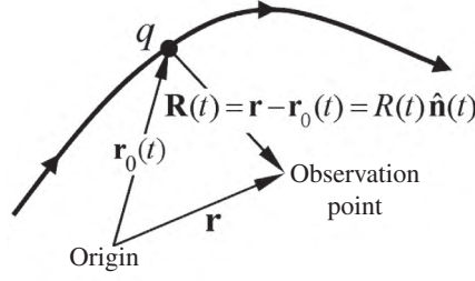
Figure 23.1: The trajectory \mathbf{r}_0(t) of a point charge q .
