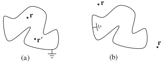
Figure 8.13: (a) \mathbf{r} and \mathbf{r}' lie inside a grounded shell of finite volume; (b) \mathbf{r} and \mathbf{r}' lie outside a grounded shell of finite volume.
