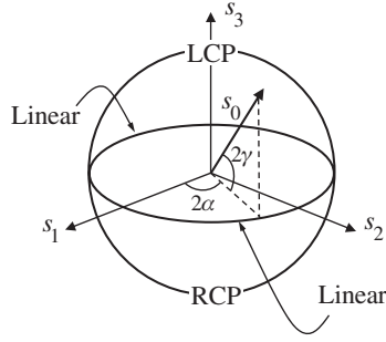
Figure 16.9: A Poincaré sphere with radius s_0 . The Cartesian coordinates of the tip of the indicated vector are (s_1, s_2, s_3) .
