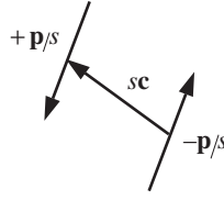
Figure 4.10: A quadrupole composed of two oppositely directed dipoles.
