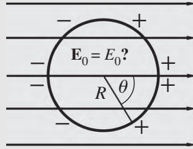
Figure 5.2: A conducting sphere in a uniform external field E\hat{\mathbf{z}} . Plus and minus signs indicate the induced surface charge density \sigma(\theta) .
