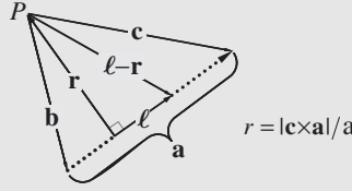
Figure 10.4: The wire segment a (dotted) carries a steady current I from the head of the vector b to the head of the vector c . The observation point is P .
