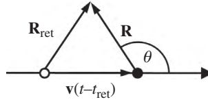
Figure 23.18: The present-time position (black dot) and retarded-time position (small white circle) of a charge moving with constant velocity v . R and R_{\text{ret}} point to the observation point.
