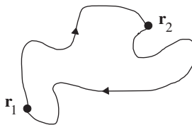
Figure 3.3: A closed path C that can be used in (3.16) to demonstrate that the work done by the Coulomb force is path-independent.
