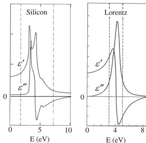
Figure 18.4: Real and imaginary parts of \hat{\epsilon}(\omega)/\epsilon_0 for silicon. Left panel: experiment. Right panel: Lorentz model. Vertical dashed lines are discussed in the text. Figure adapted from Wooten (1972).
