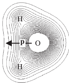
Figure 4.2: Contours of constant charge density for an \text{H}_2\text{O} molecule. This object has a non-zero electric dipole moment \mathbf{p} because chemical bonding draws negative (electron) charge toward the oxygen atom from the hydrogen atoms. Figure adapted from Bader (1970).
