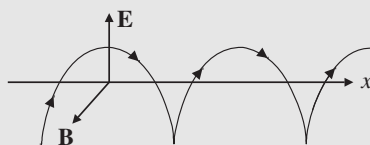
Figure 12.1: The trajectory of a charge q > 0 in the crossed fields \mathbf{B} = B\hat{\mathbf{z}} and \mathbf{E} = E\hat{\mathbf{y}} . The particle begins at rest from the origin.
