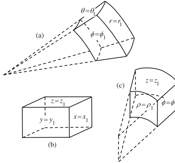
Figure 7.3: Volumes bounded by surfaces where one coordinate variable is constant: (a) spherical coordinates; (b) Cartesian coordinates; (c) cylindrical coordinates.
