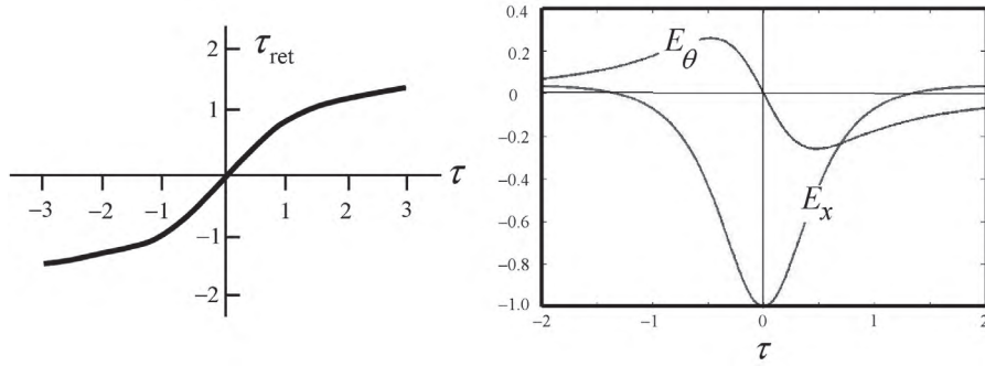
Figure 23.12: Left panel: approximate solution for the function \tau_{\text{ret}}(\tau) which satisfies (23.120). Right panel: the electric field from a pulse of synchrotron radiation as a function of scaled observer time. The observation point is \Theta = 1 in the y - z plane of Figure 23.8.
