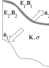
Figure 2.8: An infinitesimally thin interface between two macroscopic regions (labeled 1 and 2) carries a surface charge density \sigma and a surface current density \mathbf{K} . The unit normal \hat{\mathbf{n}}_1 points outward from region 1. The unit normal \hat{\mathbf{n}}_2 points outward from region 2.
