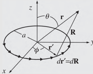
Figure 20.4: A ring formed from N point electric dipoles arranged head-to-tail.
