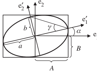
Figure 16.6: The polarization ellipse (heavy solid line) traced out by the tip of the \mathbf{E} vector for a general monochromatic plane wave.
