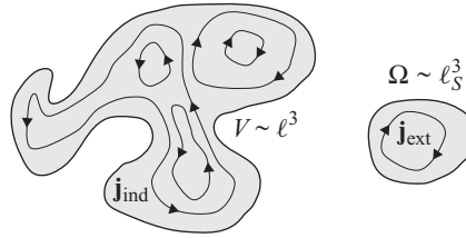
Figure 14.18: By Faraday induction, the closed loops of a time-varying external current density \mathbf{j}_{\text{ext}} induce closed loops of eddy current with density \mathbf{j}_{\text{ind}} in a nearby ohmic medium.
