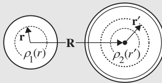
Figure 4.13: Two spherical charge distributions that do not overlap in space.
