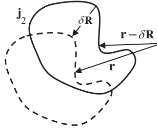
Figure 12.13: Illustration that a rigid shift \delta \mathbf{R} of the current density \mathbf{j}_2 produces a change in the current density at a point \mathbf{r} of \delta \mathbf{j}_2(\mathbf{r}) = \mathbf{j}_2(\mathbf{r} - \delta \mathbf{R}) - \mathbf{j}_2(\mathbf{r}) .
