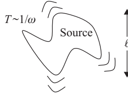
Figure 14.9: A source distribution of size \ell with maximal time variations that occur over a characteristic time T \sim 1/\omega .
