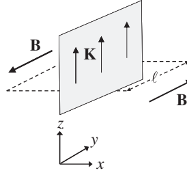
Figure 10.6: An infinite sheet of current with density \mathbf{K} = K\hat{\mathbf{z}} and the Ampèrian loop (dashed) used to find \mathbf{B} .
