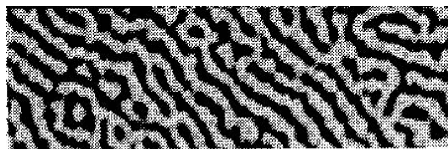
Figure 4.6: Fluorescence microscopic image ( 40\text{ }\mu\text{m} \times 160\text{ }\mu\text{m} ) looking down onto a liquid mixture of cholesterol and a phospholipid trapped at an air-water interface parallel to the image. The black regions are long, thin “drops” of the liquid, with a thickness of exactly one molecule. Figure from Seul and Chen (1993).
