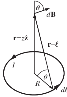
Figure 10.2: Geometry for a Biot-Savart calculation of the magnetic field on the symmetry axis of a circular current loop.
