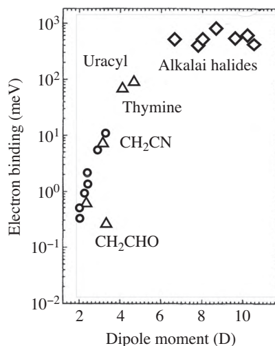
Figure 4.4: The binding energy of an electron captured by a polar molecule. One debye (D) is = 3.36 \times 10^{-30} C-m. Figure adapted from Desfr  ois et al. (1994).
