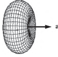
Figure 23.6: Angular distribution of radiation emitted by a slowly moving ( v \ll c ) point charge with acceleration \mathbf{a} .
