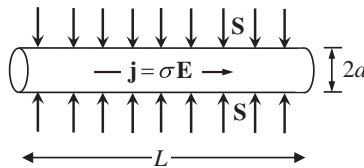
Figure 15.1: The lines of the Poynting vector \mathbf{S} point radially inward at the surface of a current-carrying ohmic wire.
