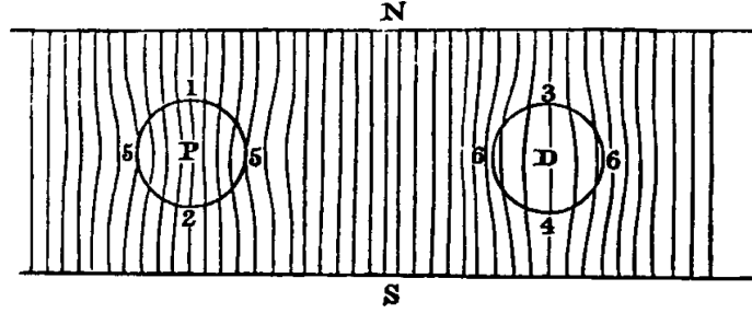
Figure 13.13: A diagram of lines of \mathbf{B}(\mathbf{r}) published by Faraday for a uniform field perturbed by magnetizable rods that point out of the plane of the paper. \mathbf{B}_{\text{in}} > \mathbf{B}_0 for the paramagnetic (P) rod on the left. \mathbf{B}_{\text{in}} < \mathbf{B}_0 for the diamagnetic (D) rod on the right. Faraday did not know that the field inside both rods is uniform [see (13.82)]. The numerical labeling was used by him in his discussion. The diagram appears in an 1851 entry of his Experimental Researches in Electricity .
