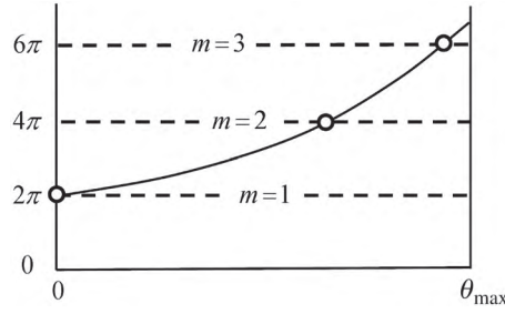
Figure 19.15: Graphical solution of (19.97) shows that only a finite number of modes propagate in a typical dielectric waveguide.
