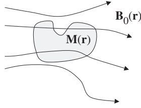
Figure 13.20: An isolated sample of magnetized matter in the presence of an external magnetic field \mathbf{B}_0(\mathbf{r}) . The field lines represent \mathbf{B}_0(\mathbf{r}) only.
