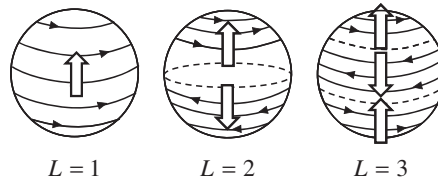
Figure 11.8: Lines of surface current density on a sphere which produce pure dipole ( L = 1 ), quadrupole ( L = 2 ), and octupole ( L = 3 ) magnetic fields outside the sphere. See text for discussion of the superimposed arrows.
