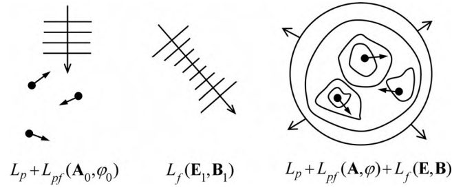
Figure 24.1: A tale of three Lagrangians. Left panel: particle trajectories are determined by the Coulomb-Lorentz force exerted by an external field with specified potentials (\mathbf{A}_0, \varphi_0) . Middle panel: a field (\mathbf{E}_1, \mathbf{B}_1) evolves according to the source-free Maxwell equations. Right panel: a field (\mathbf{E}, \mathbf{B}) evolves according to the Maxwell-equations with the particles as the source of charge and current. The Coulomb-Lorentz force exerted by this field acts back on the particles and determines their trajectories.
