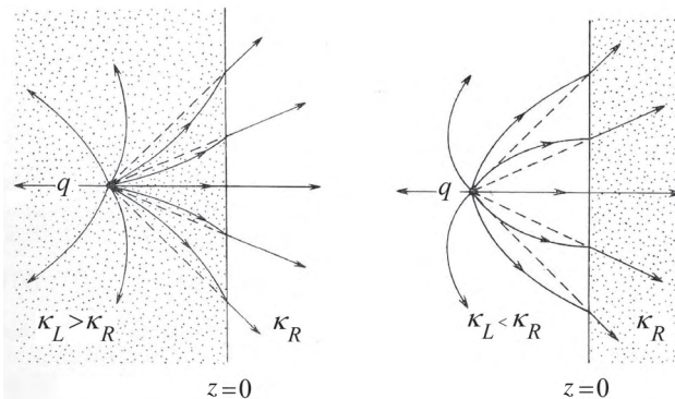
Figure 8.4: Lines of \mathbf{E}(\mathbf{r}) for a point charge near a flat dielectric interface for \kappa_L > \kappa_R (left panel) and \kappa_L < \kappa_R (right panel). Figure from Durand (1966).
