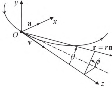
Figure 23.8: A point charge moves along a curved trajectory in the x - z plane.
