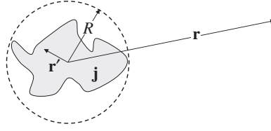
Figure 11.1: A localized current distribution confined to the interior of a sphere of radius R . The observation point \mathbf{r} lies outside the sphere.
