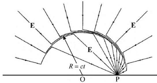
Figure 23.3: Electric field lines for a point (negative) charge that is abruptly accelerated from rest (at point O) to at state of uniform speed at point P. Figure from Purcell (1965).
