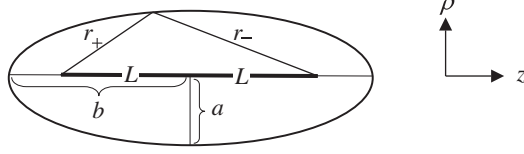
Figure 5.4: A prolate ellipsoid of revolution with semi-minor axis a and semi-major axis b . The focal length L = \sqrt{b^2 - a^2} . The line segments r_{\pm} begin at opposite foci and end at the same point on the ellipsoid surface. The surface is the locus of points where r_+ + r_- = 2b .
