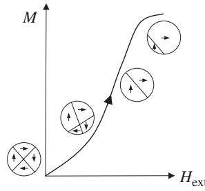
Figure 13.27: Evolution of magnetic domains during the initial magnetization of a ferromagnet. The arrows give the local direction of \mathbf{M} in each domain.
