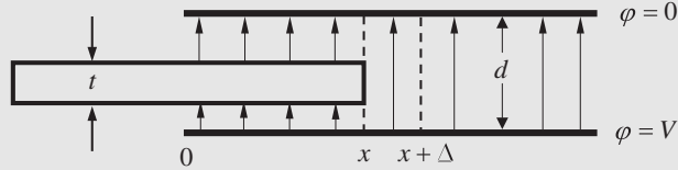
Figure 5.13: A conducting sheet of thickness t partially inserted into a capacitor with plate separation d > t .
