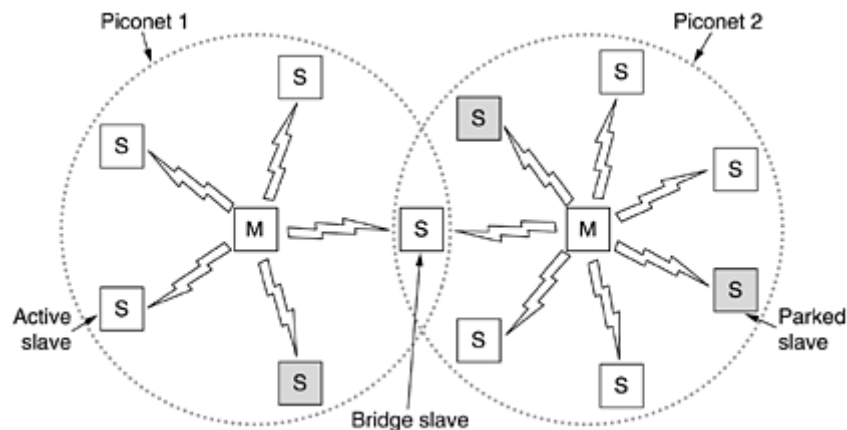
Figure 4-35. Two piconets can be connected to form a scatternet.
