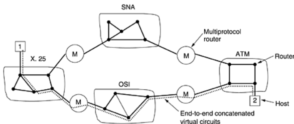
Figure 5-45. Internetworking using concatenated virtual circuits.
