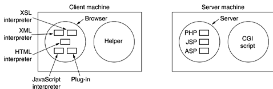
Figure 7-40. The various ways to generate and display content.
