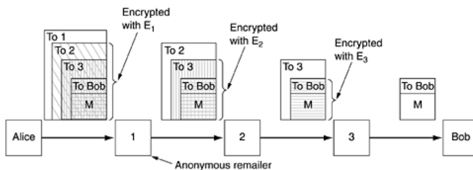
Figure 8-54. How Alice uses 3 remailers to send Bob a message.
