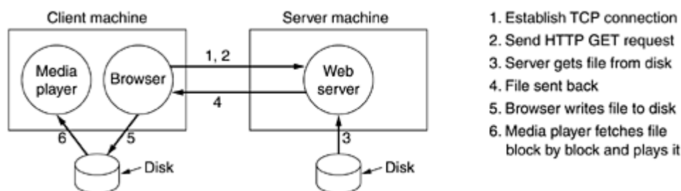
Figure 7-59. A straightforward way to implement clickable music on a Web page.
