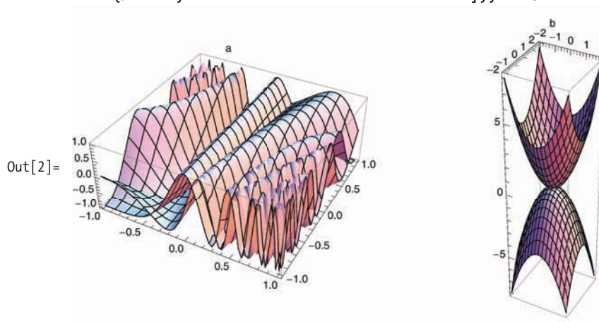
Figure 7-1. 3D plots of multiple functions
