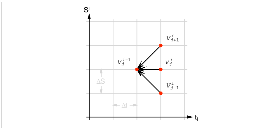
Figure 14-1. Explicit FDM
