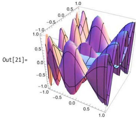
Figure 7-8. Surface in 3D space
