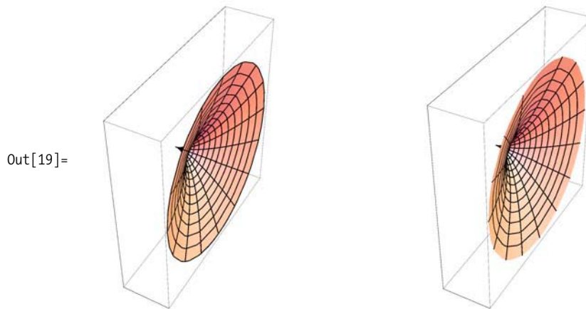
Figure 7-6. Emulating SurfaceOfRevolution
