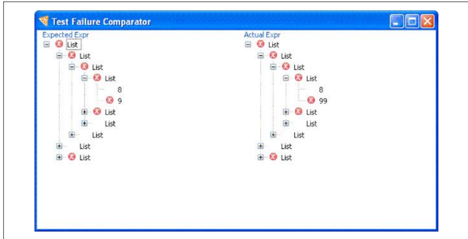
Figure 19-8. Use the test failure comparator to drill down into test results to detect problems
