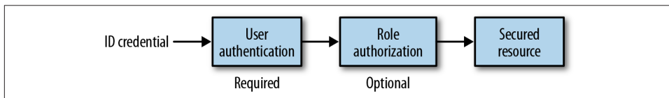
Figure 6-8. Users/roles security
