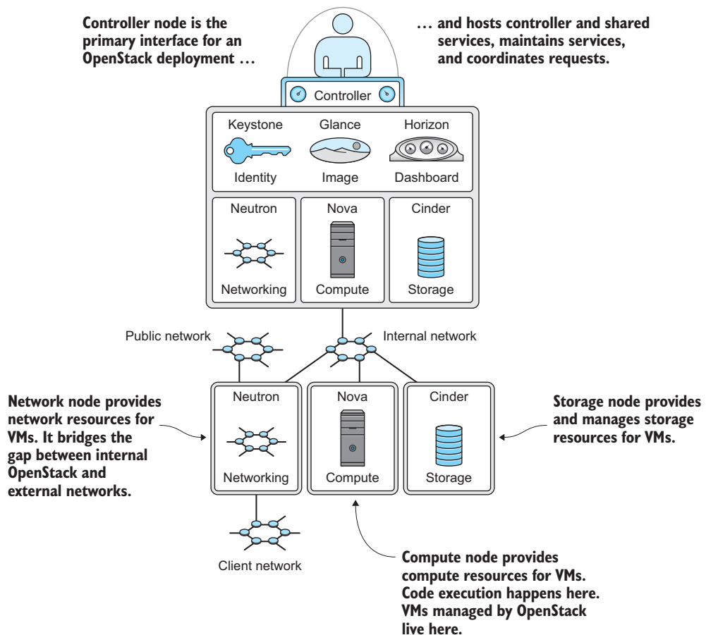
Figure 5.1 Multi-node architecture
