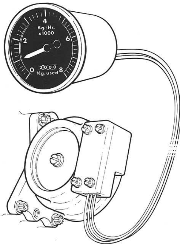
Fig. 12-10 Fuel flow transmitter and indicator.
