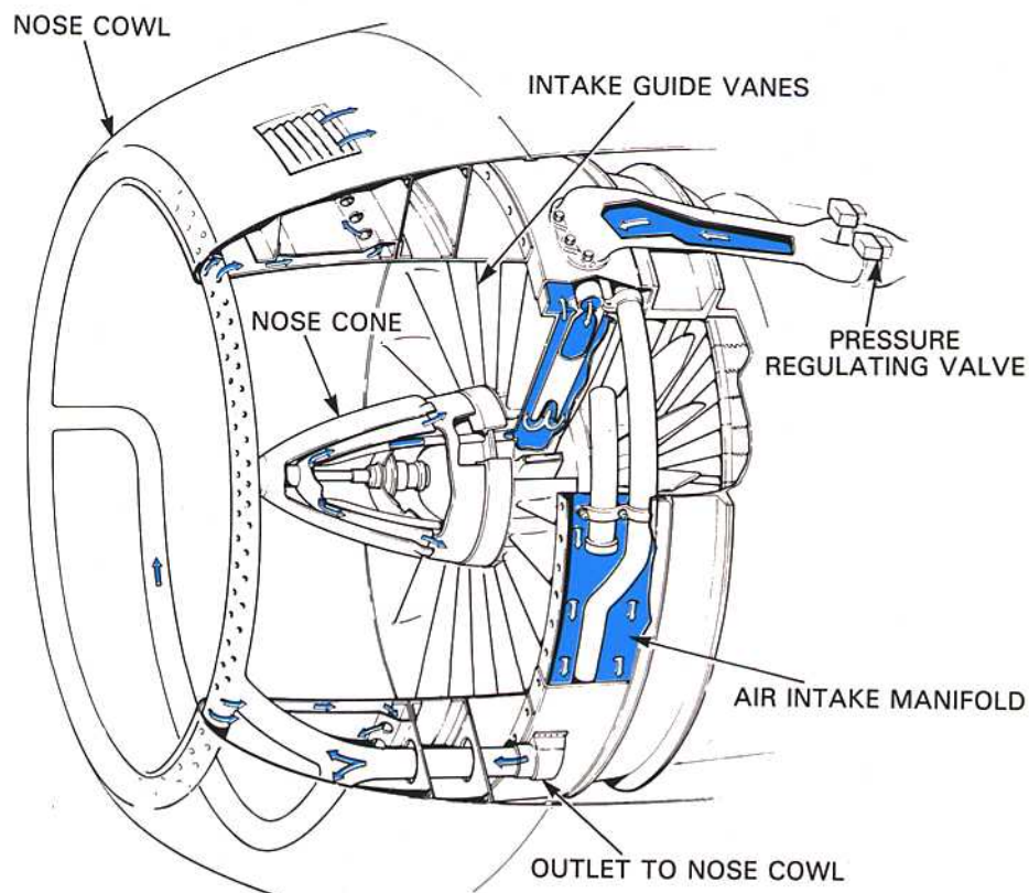
Fig. 13-2 Hot air ice protection.
