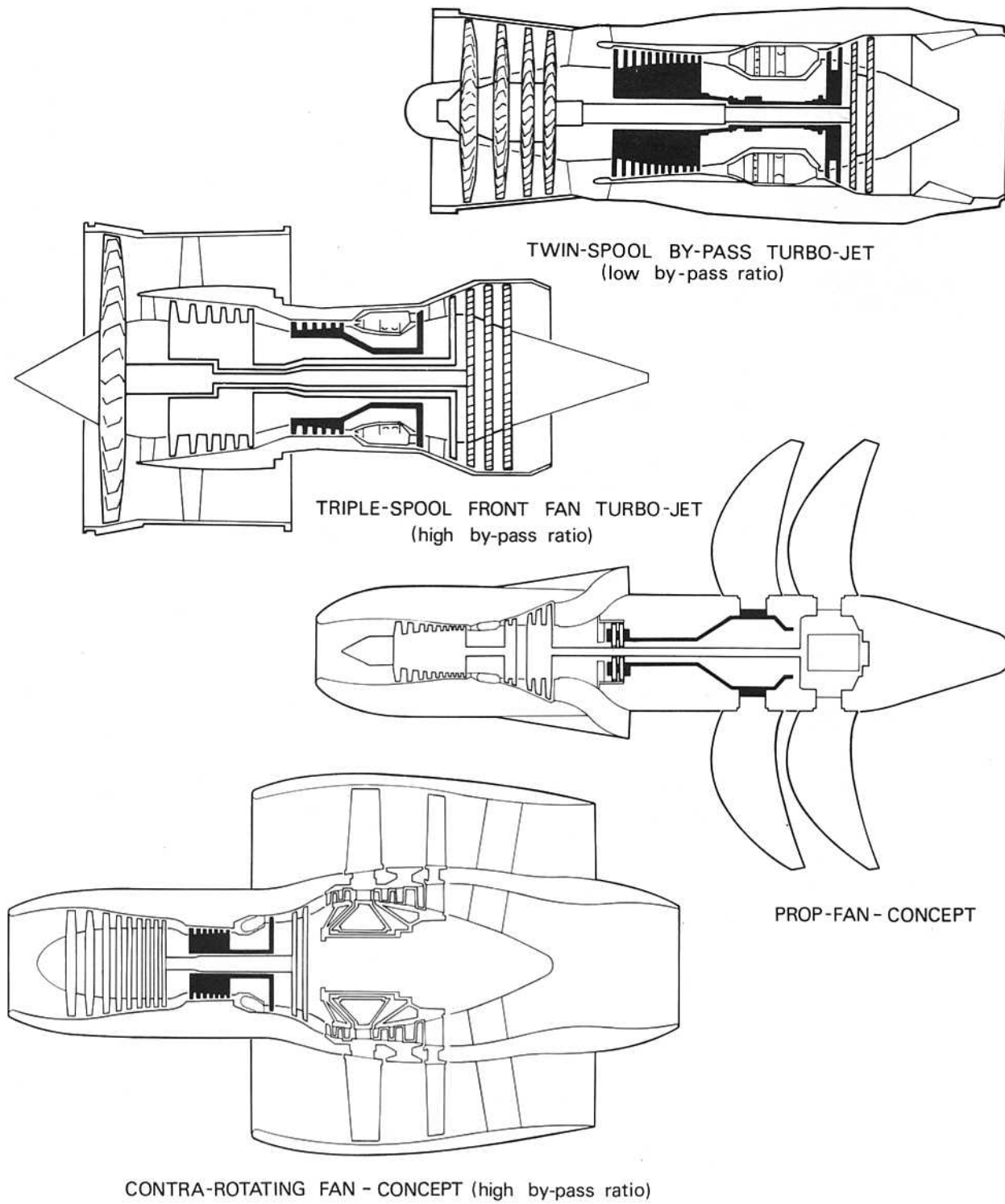
Fig. 1-9-2 Mechanical arrangement of gas turbine engines.
