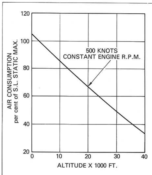
Fig. 10-1 Airflow changing with altitude.
