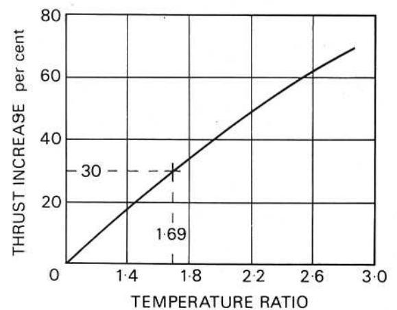
Fig. 16-8 Thrust increase and temperature ratio.
