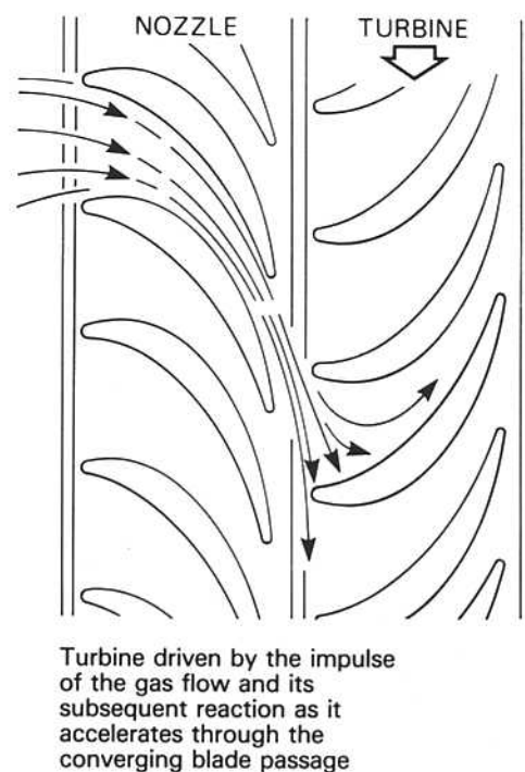
Fig. 5-5 Comparison between a pure Impulse turbine and an impulse/reaction turbine.
