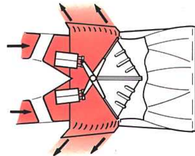
CLAMSHELL DOORS IN REVERSE THRUST POSITION
