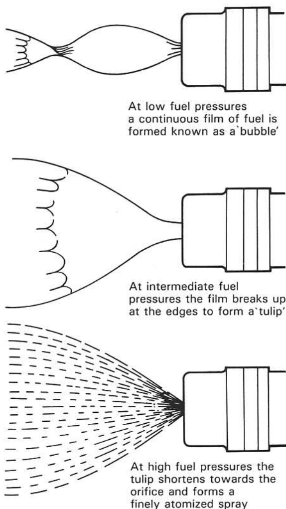
Fig. 10-15 Various stages of fuel atomization.
