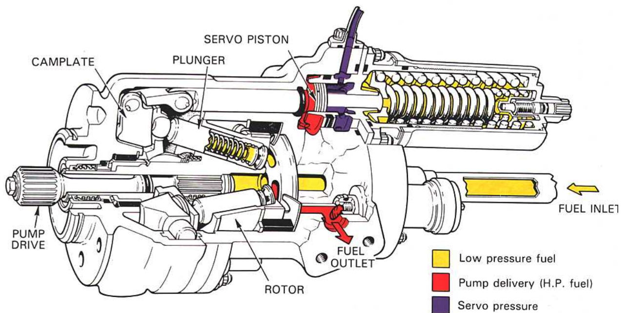
Fig. 10-14 A plunger-type fuel pump.
